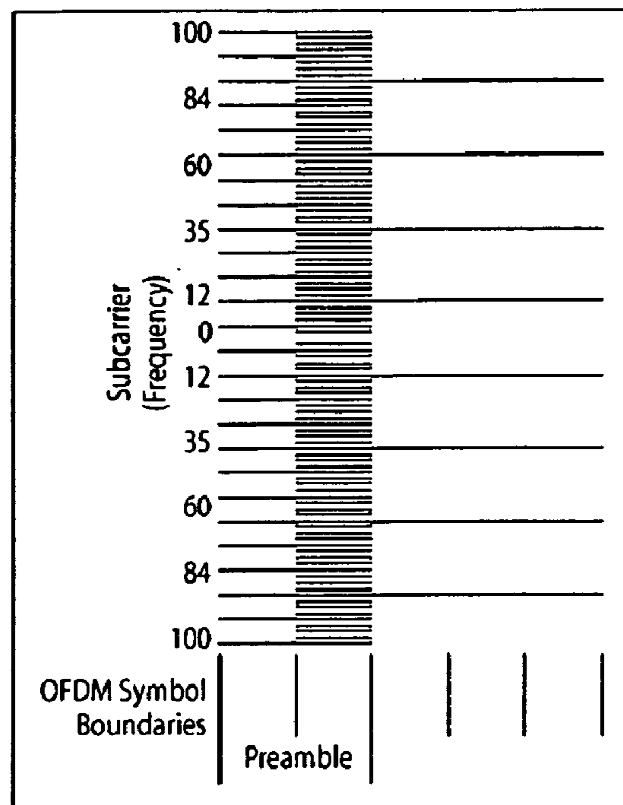
Figure 12 802.16a OFDM downlink pilot and preamble structure
