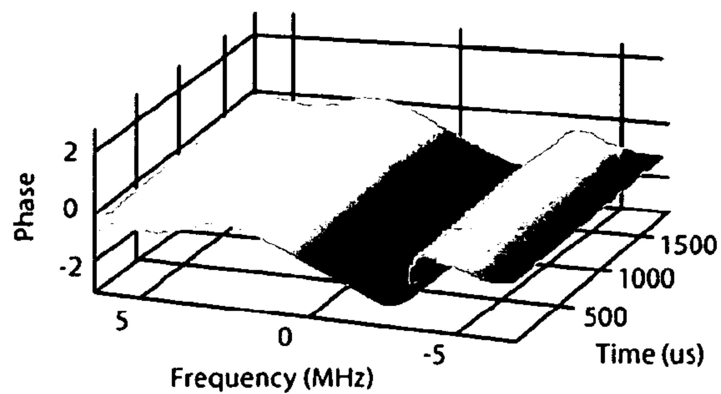
(a) Phase
