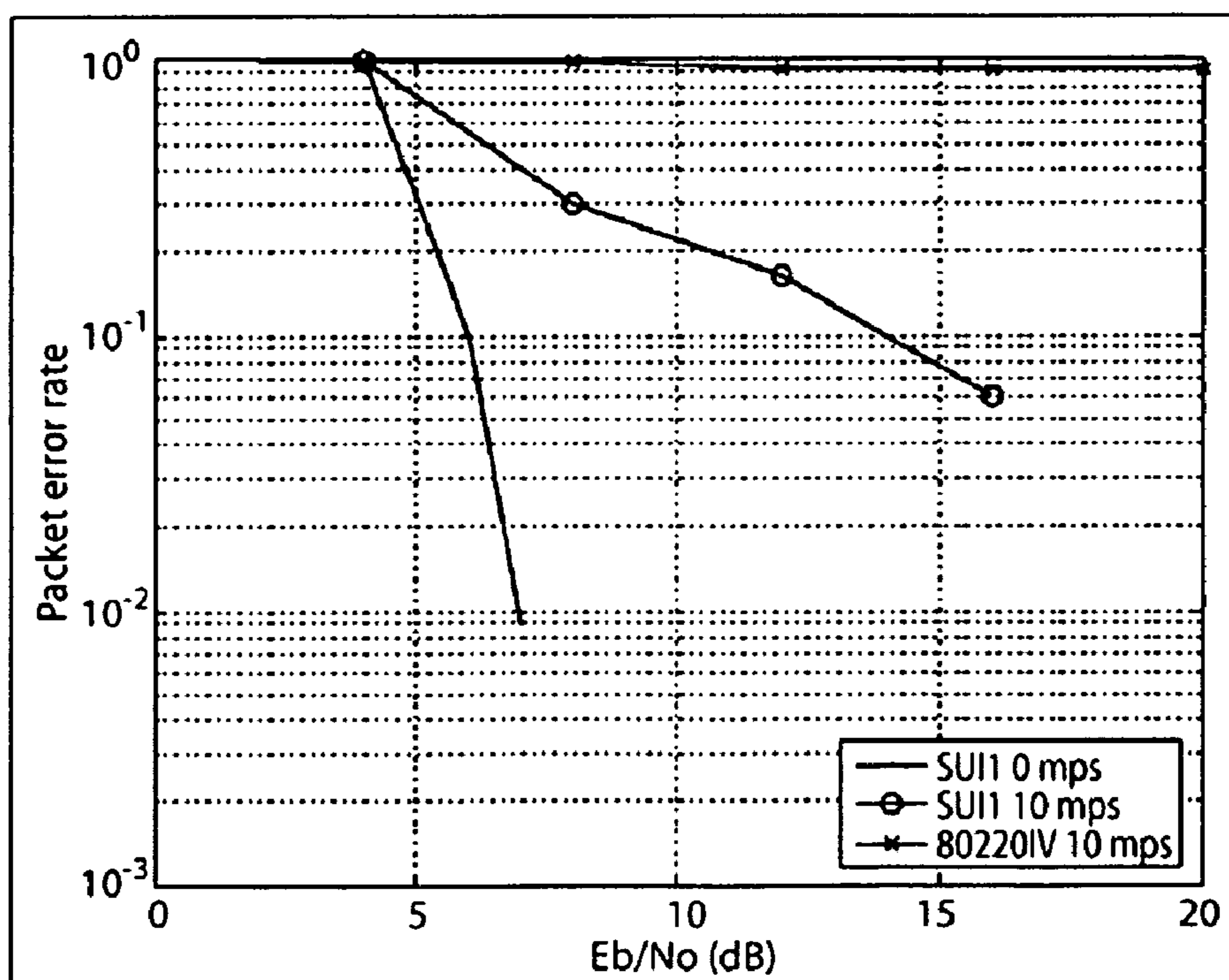
Figure 13 Packet error rate with conventional pilot assisted phase tracking
