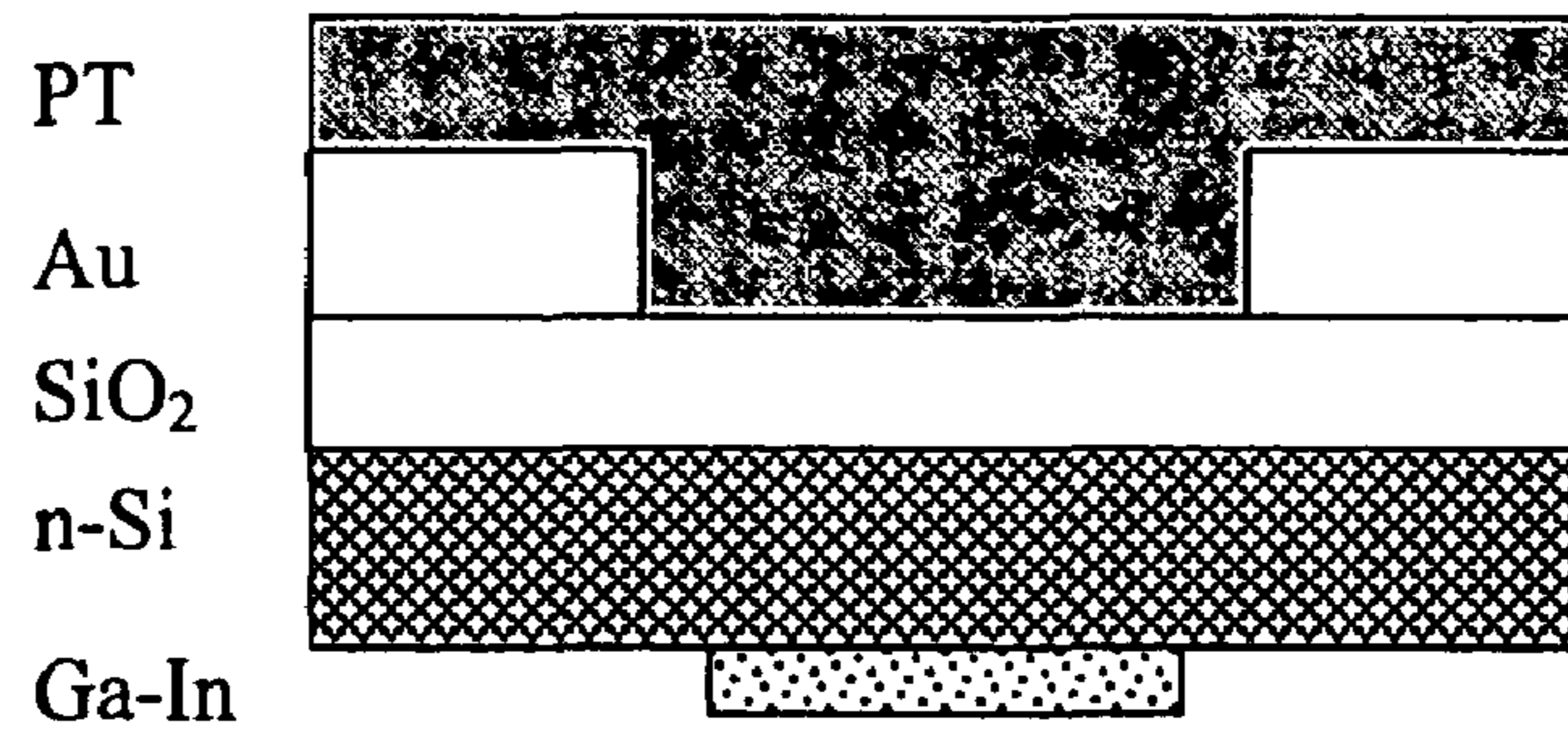
Figure 2 (prior art)
