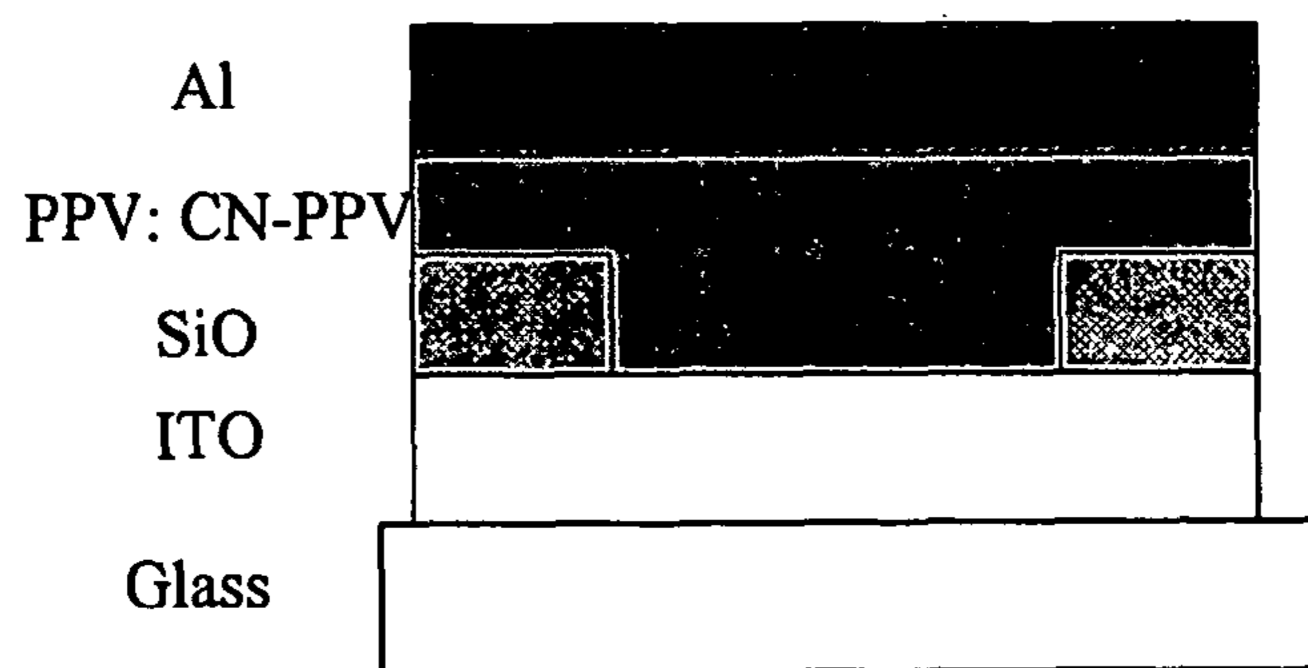
Figure 6 (prior art)
