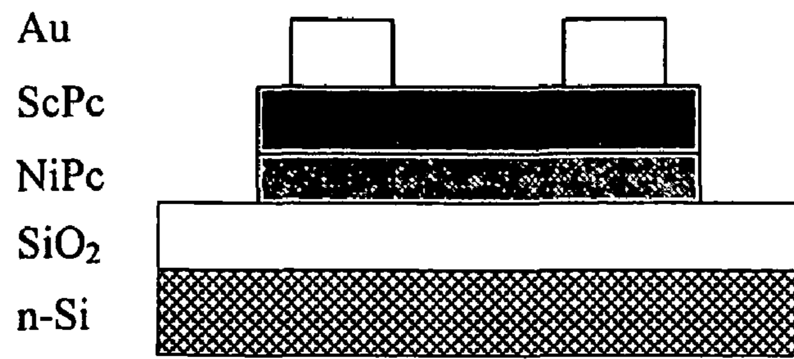
Figure 1 (prior art)
