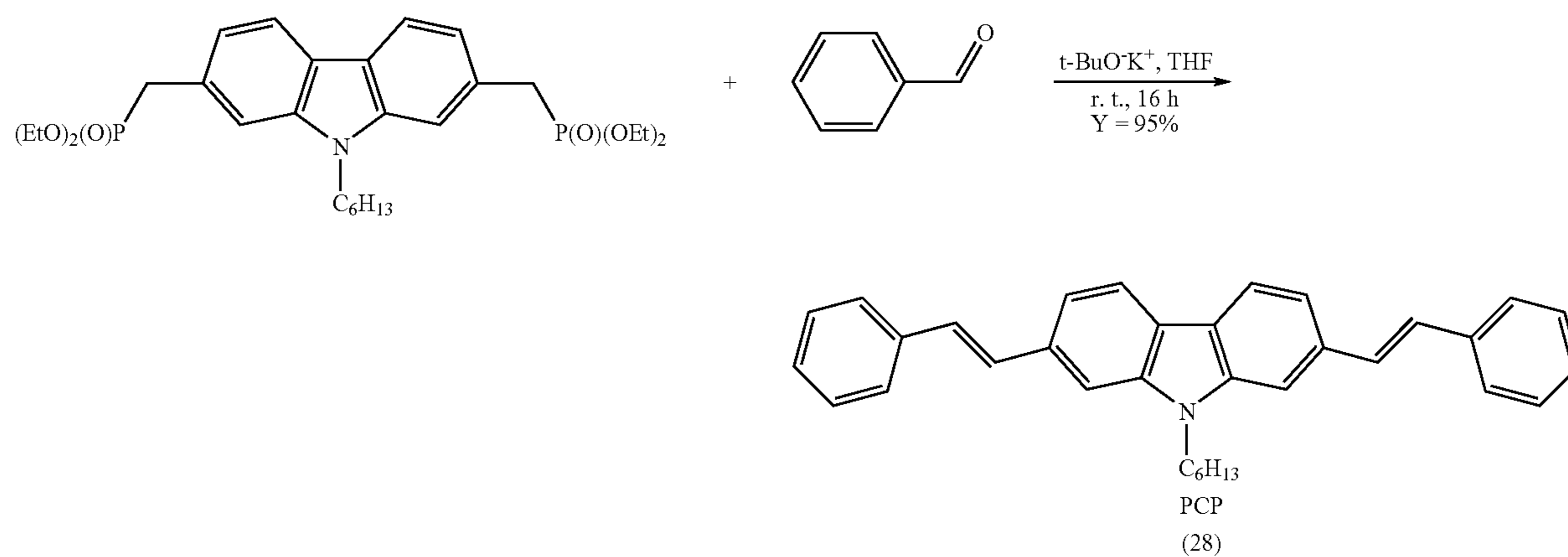
Scheme 3: Synthetic Route to 2,7-carbazolenevinylene oligomers
