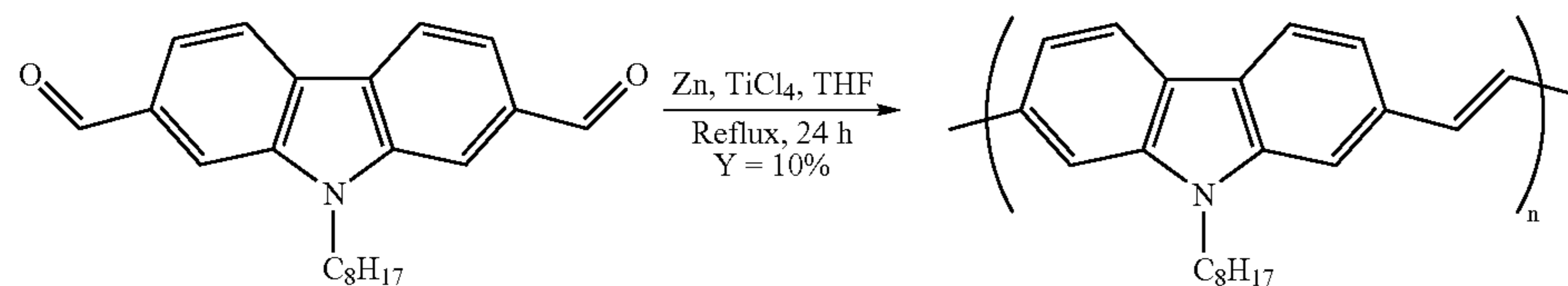
Scheme 4: Synthetic Route to 2,7-carbazolenevinylene polymers
