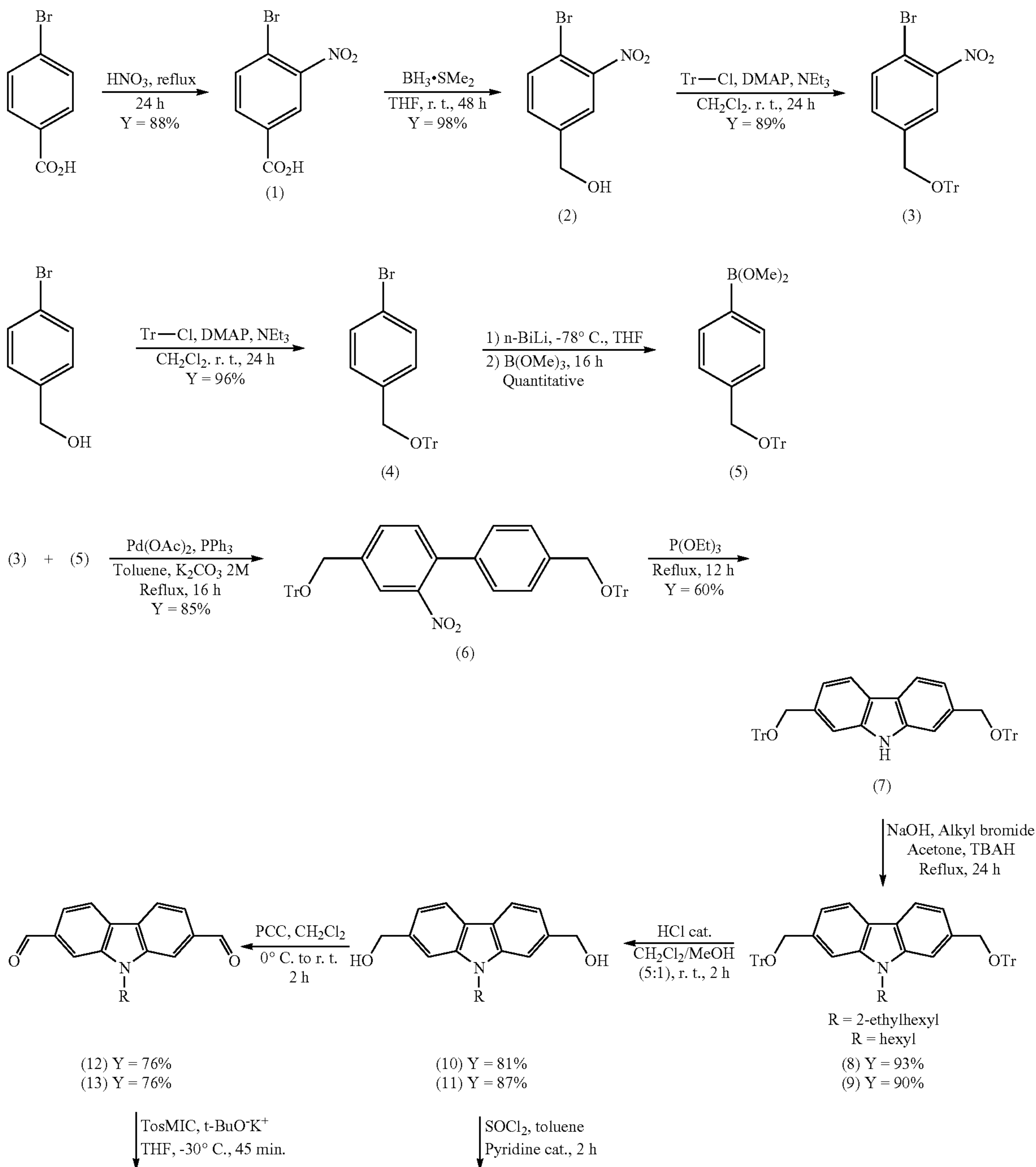
Scheme 1: Synthetic Route to 2,7-difunctionalized carbazole
