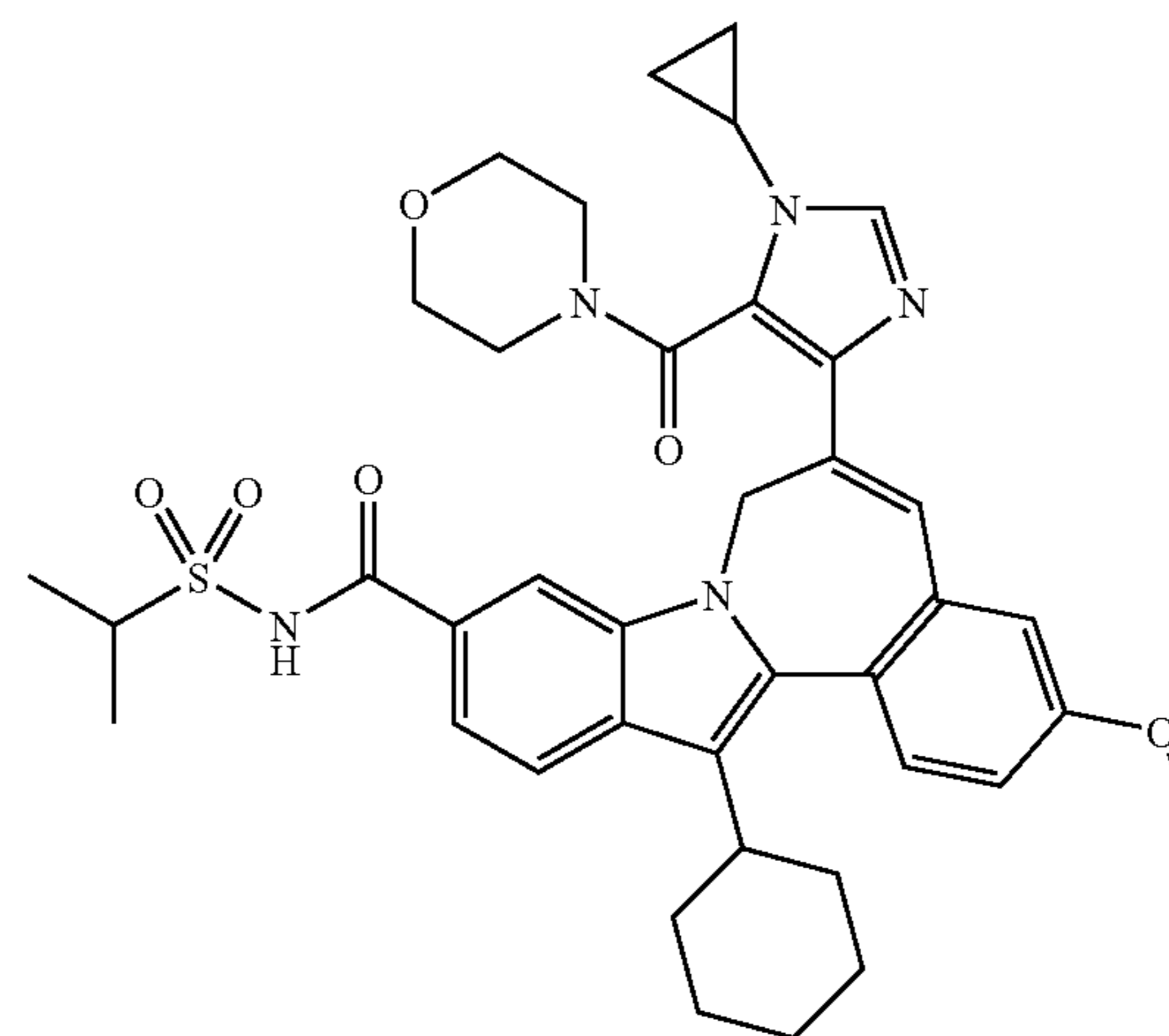
Scheme Depicting Synthesis of Compound 9:
