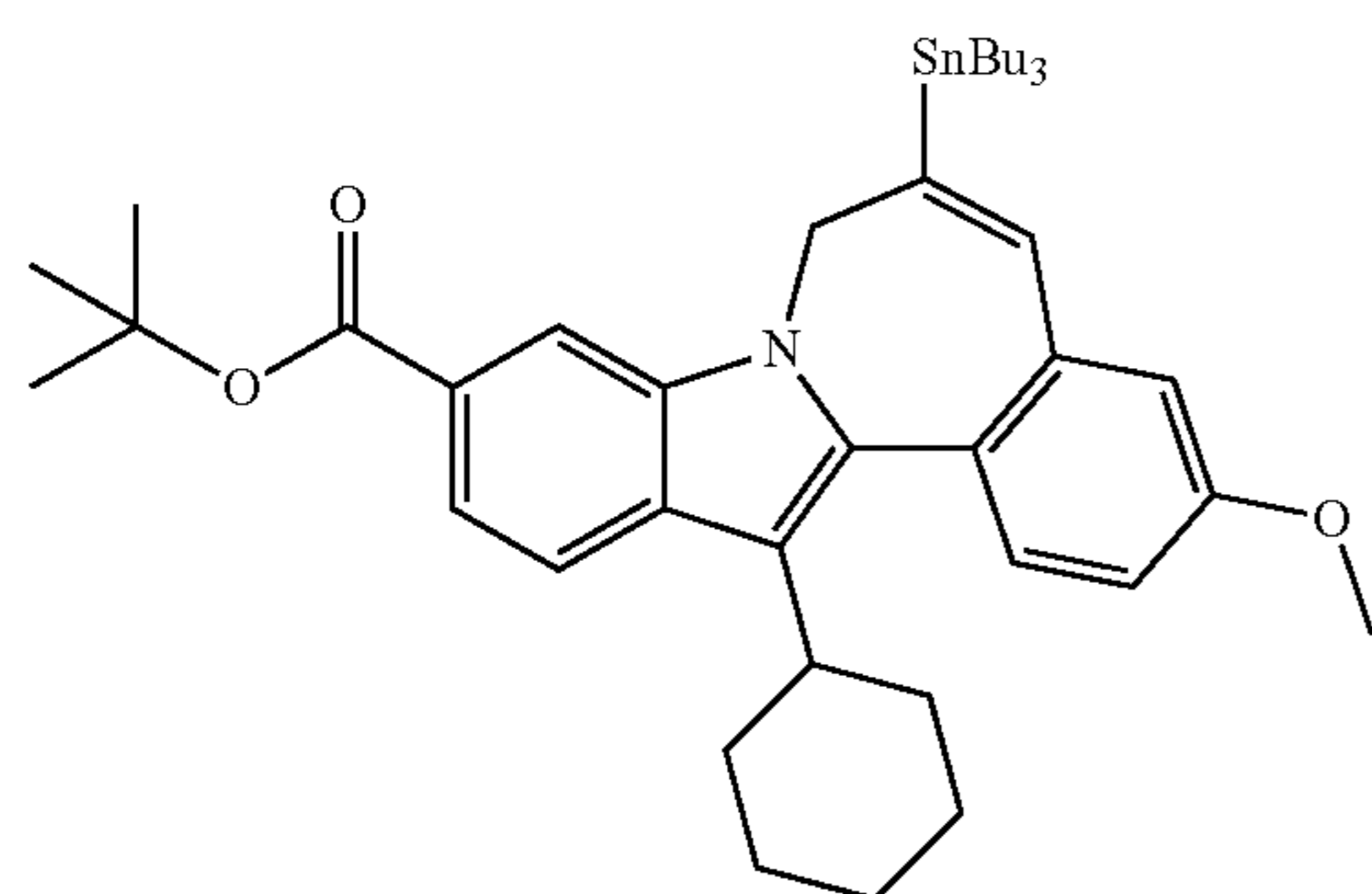
compound 1-3
