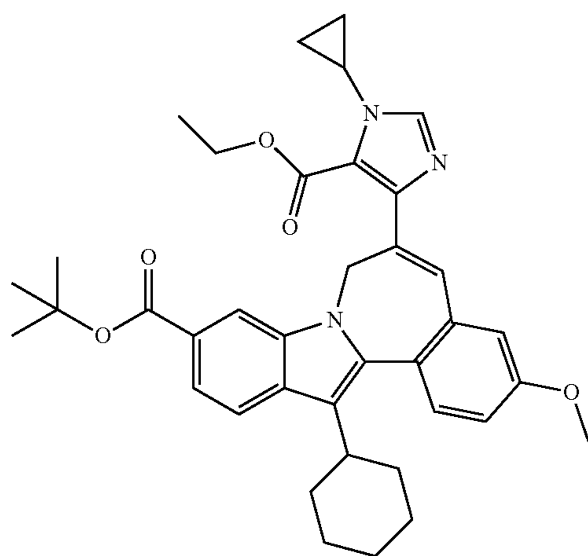
compound 9-4
