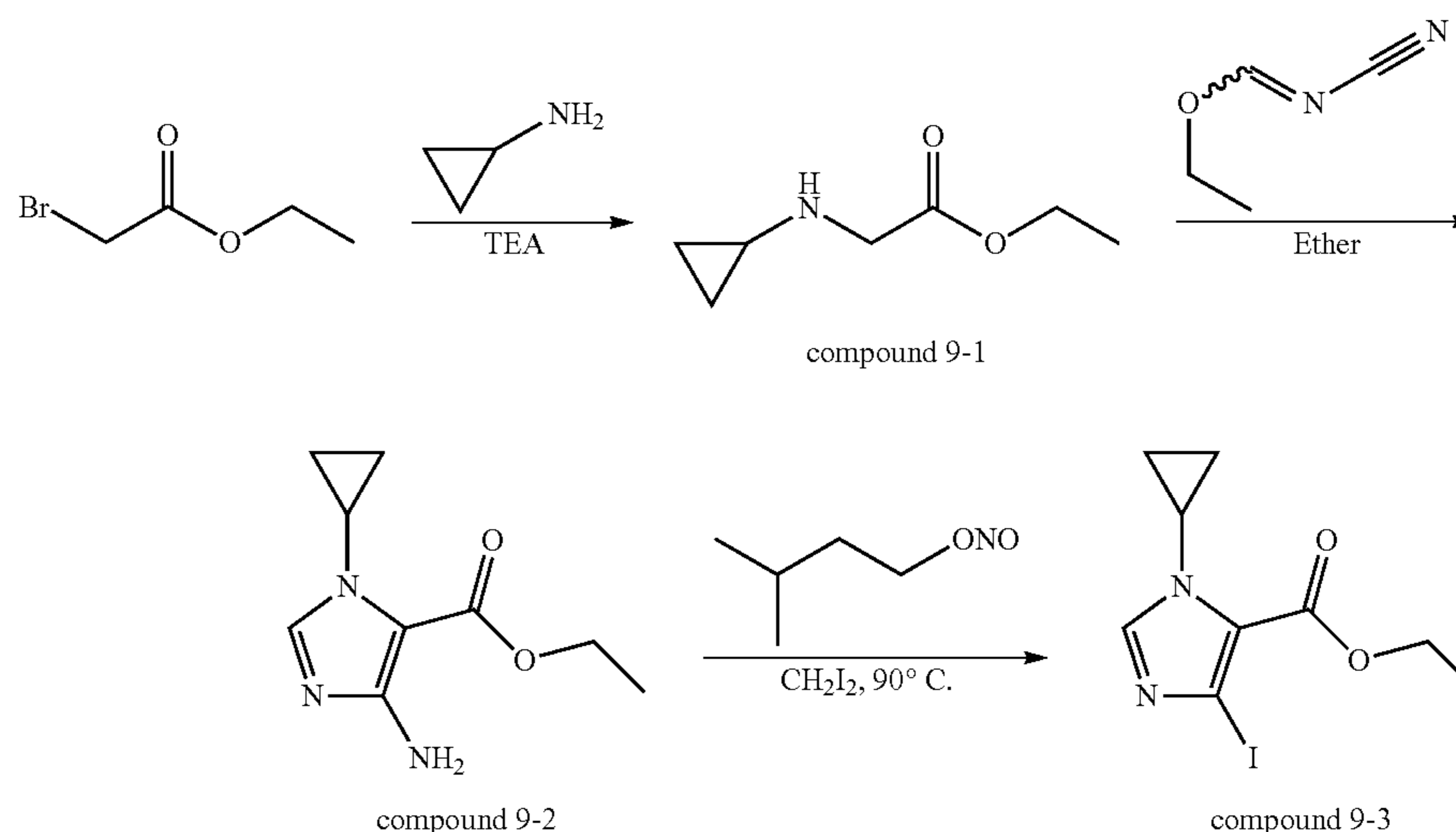
Scheme Depicting Synthesis of Compound 9:
