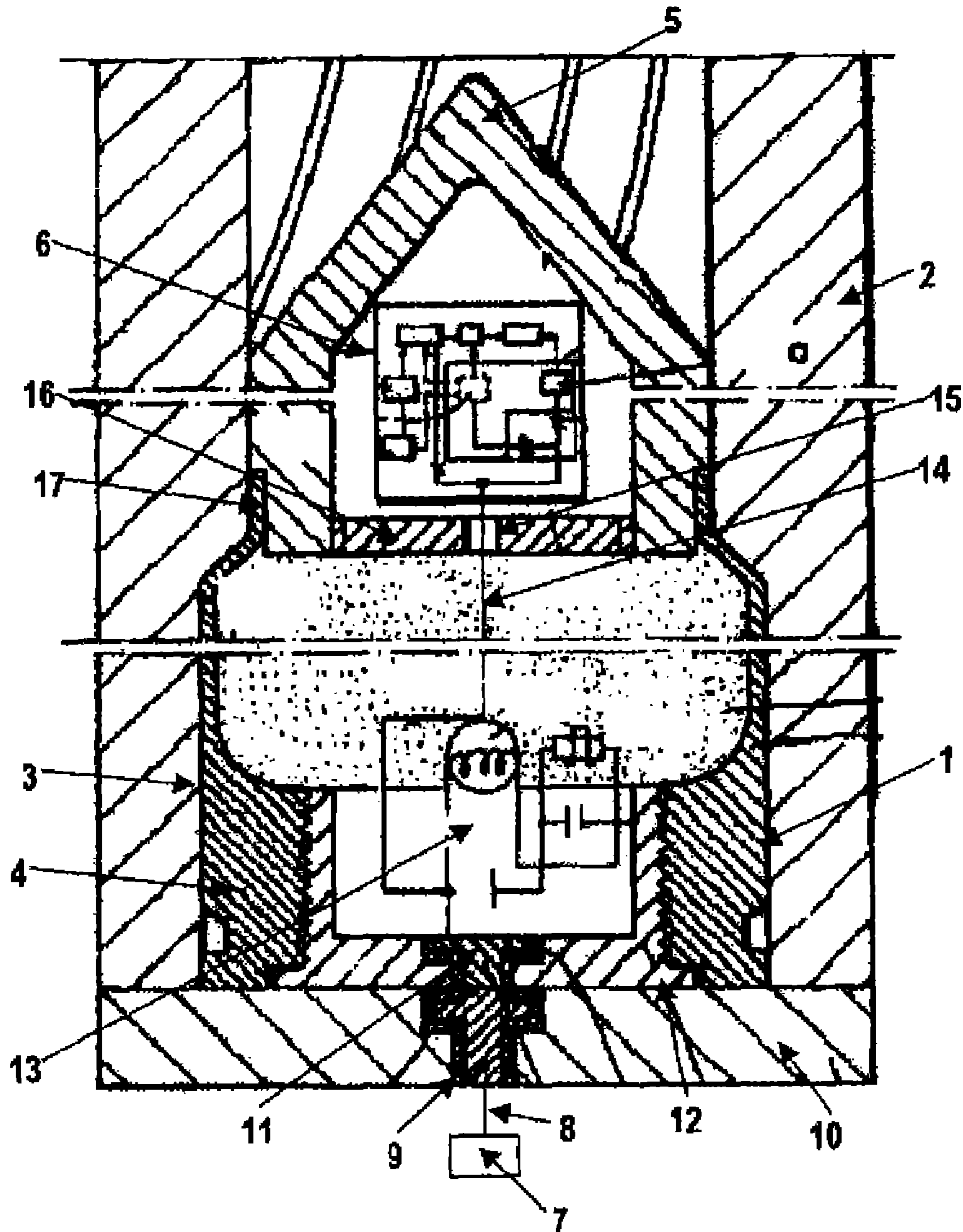
FIGURE 1 - PRIOR ART
