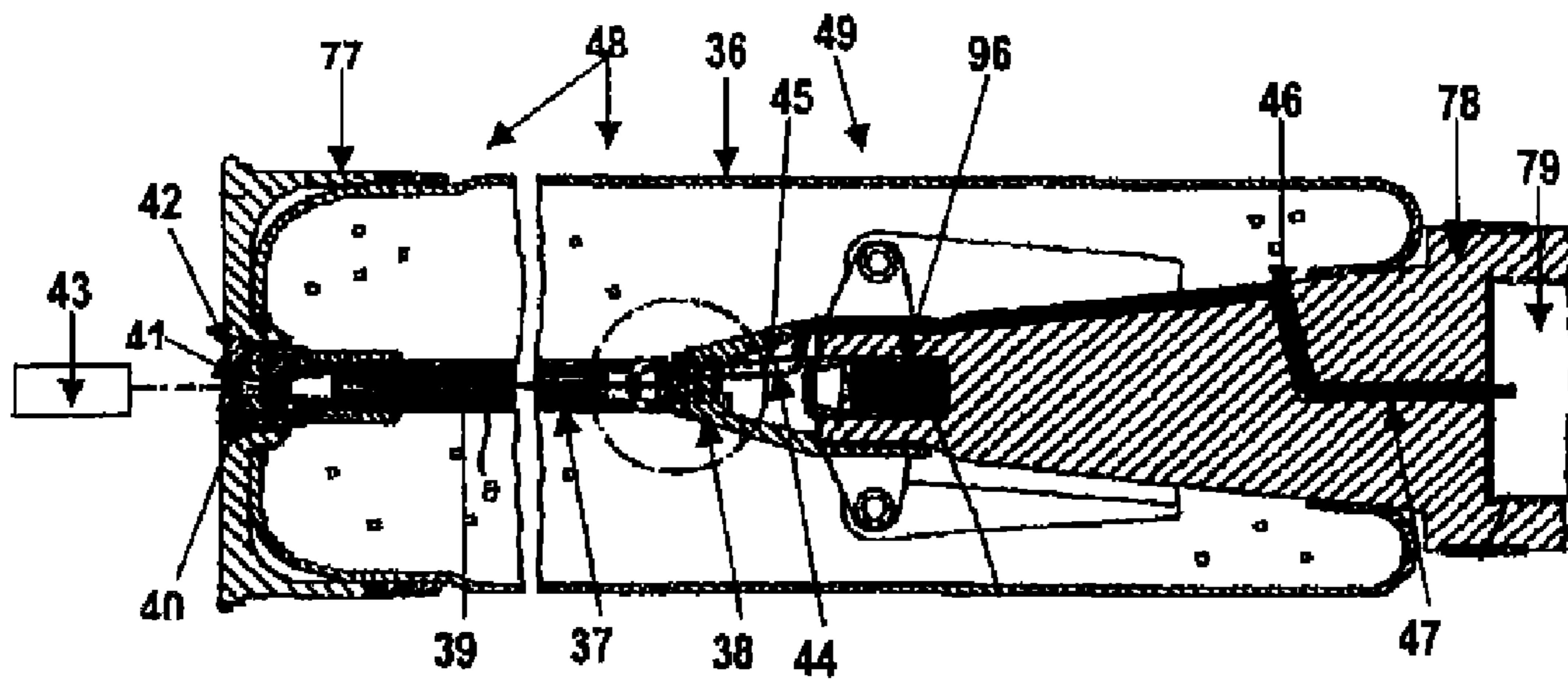
FIGURE 3 - PRIOR ART
