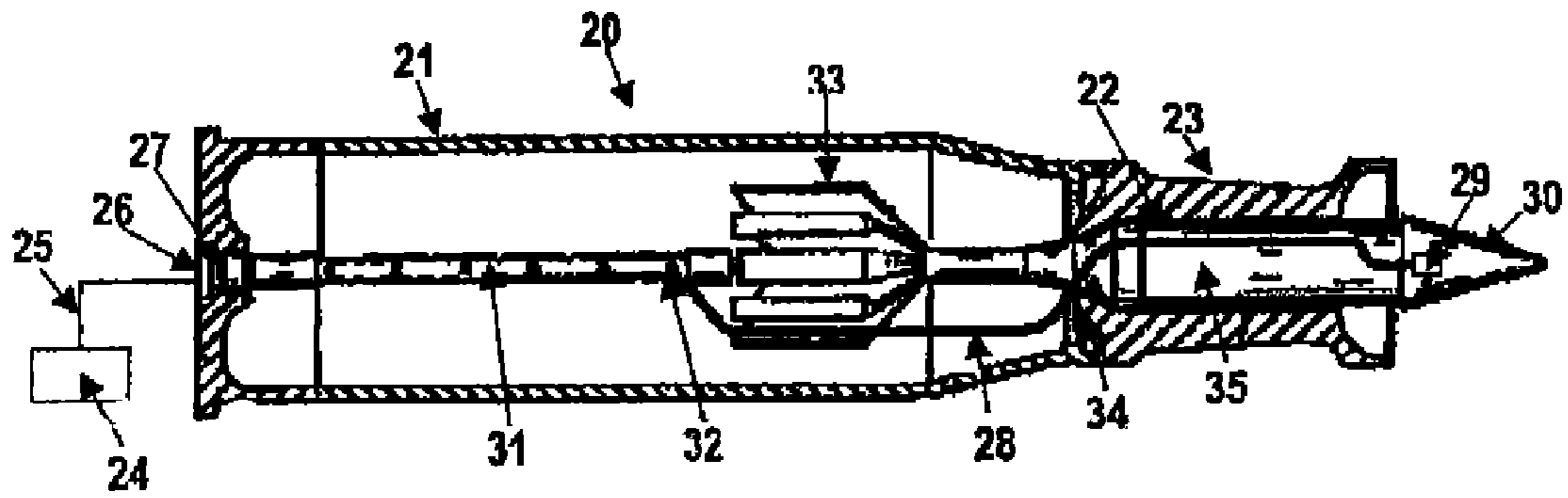
FIGURE 2 - PRIOR ART
