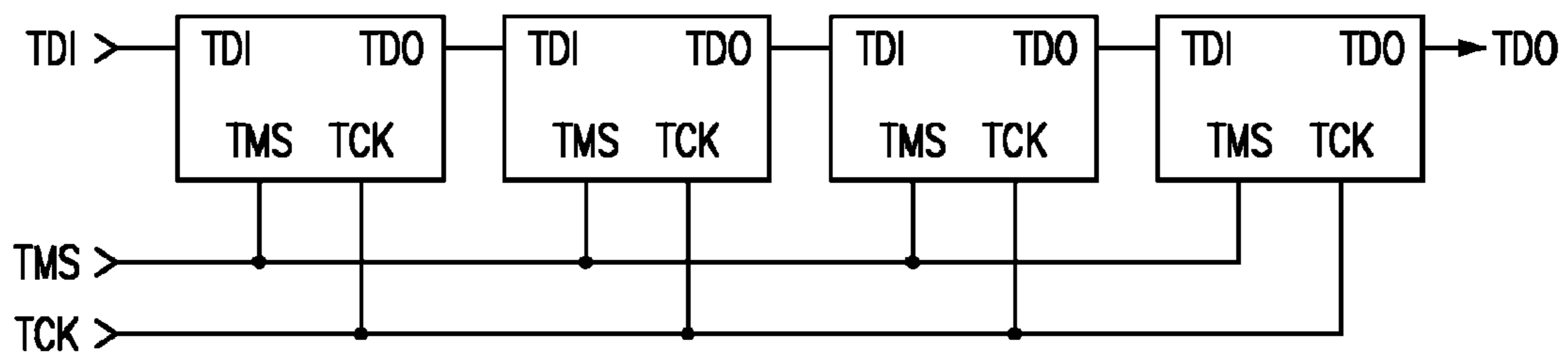
FIG. 13 (PRIOR ART)
