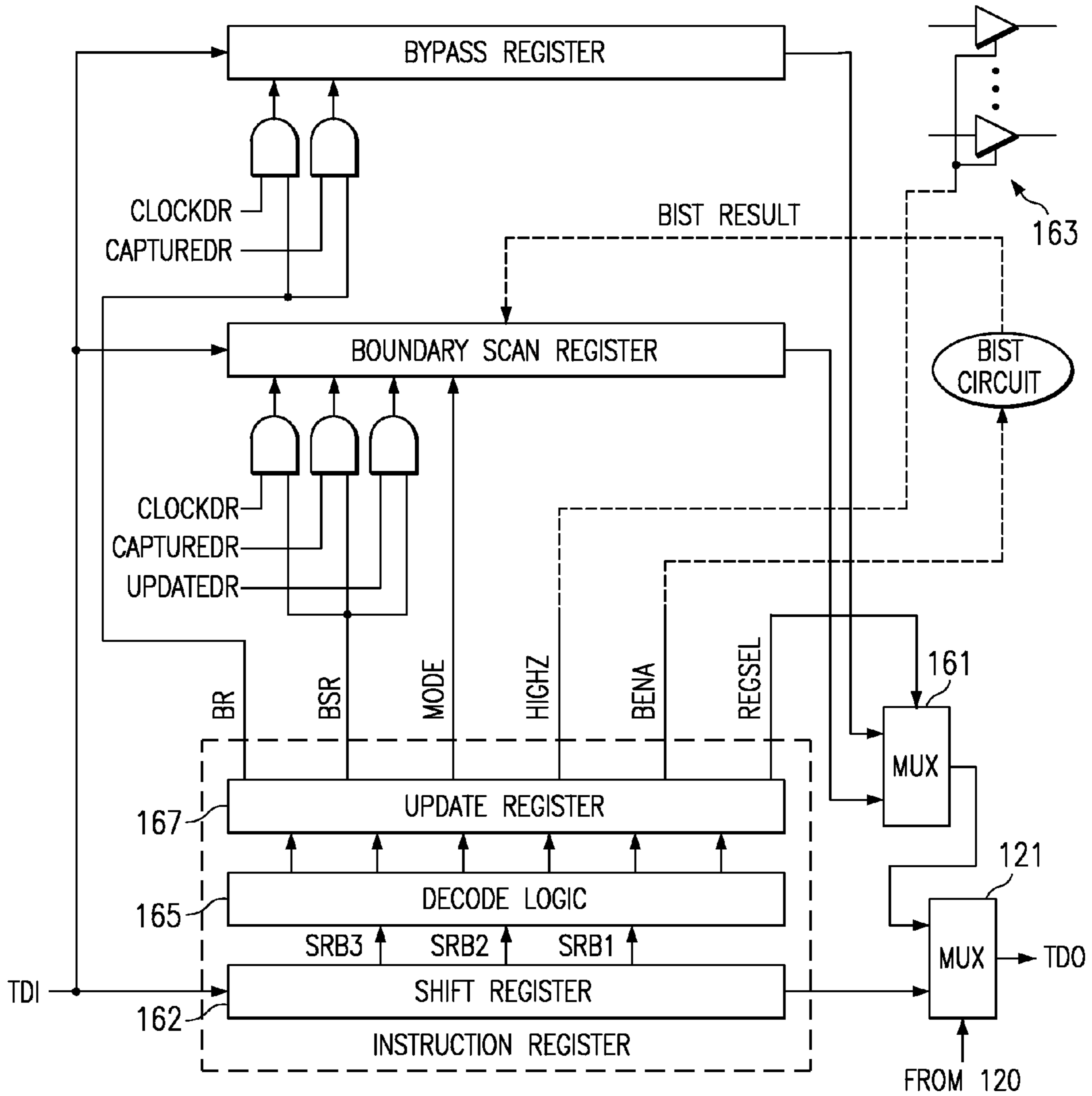
FIG. 16 (PRIOR ART)
