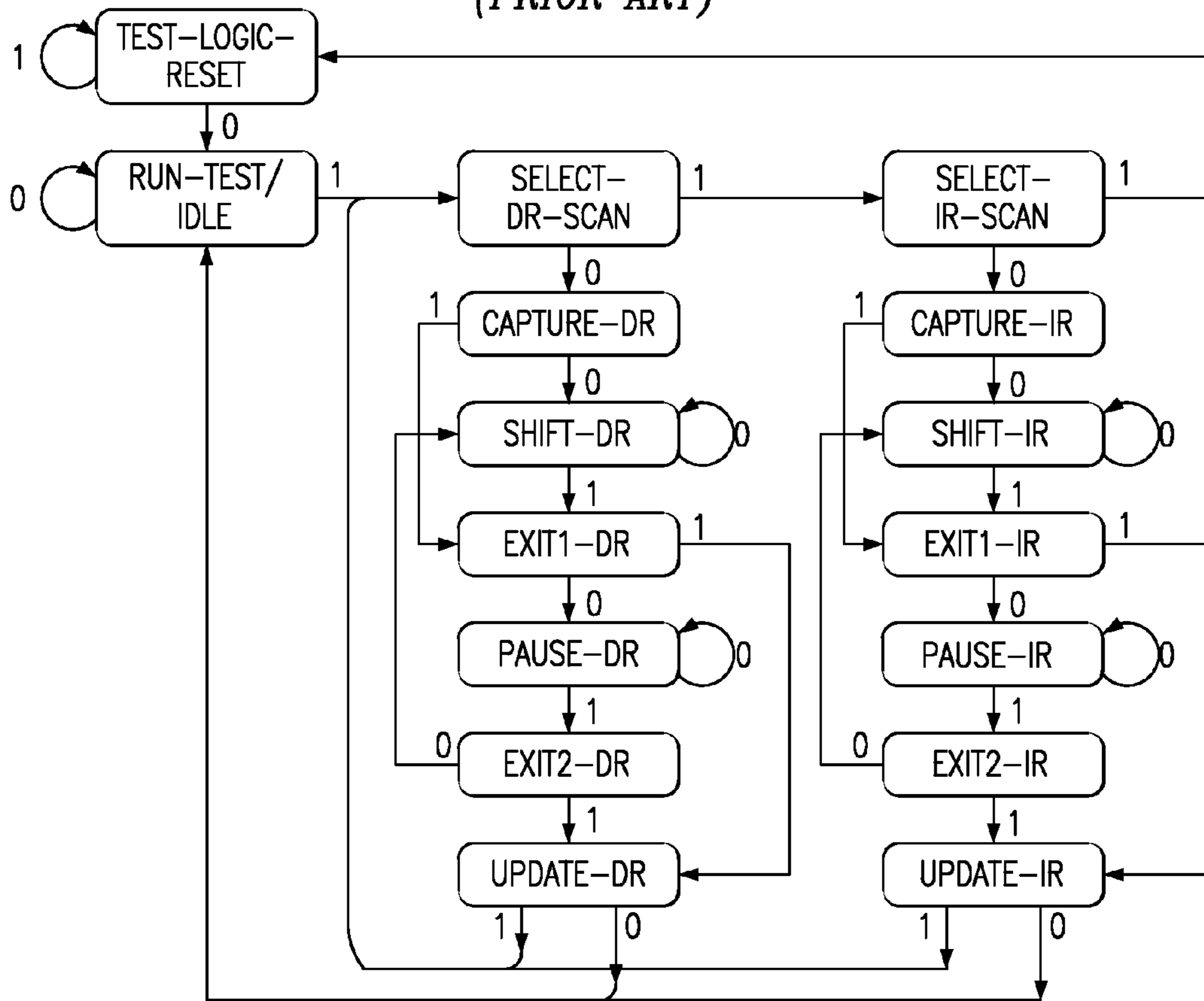
FIG. 14 (PRIOR ART)
