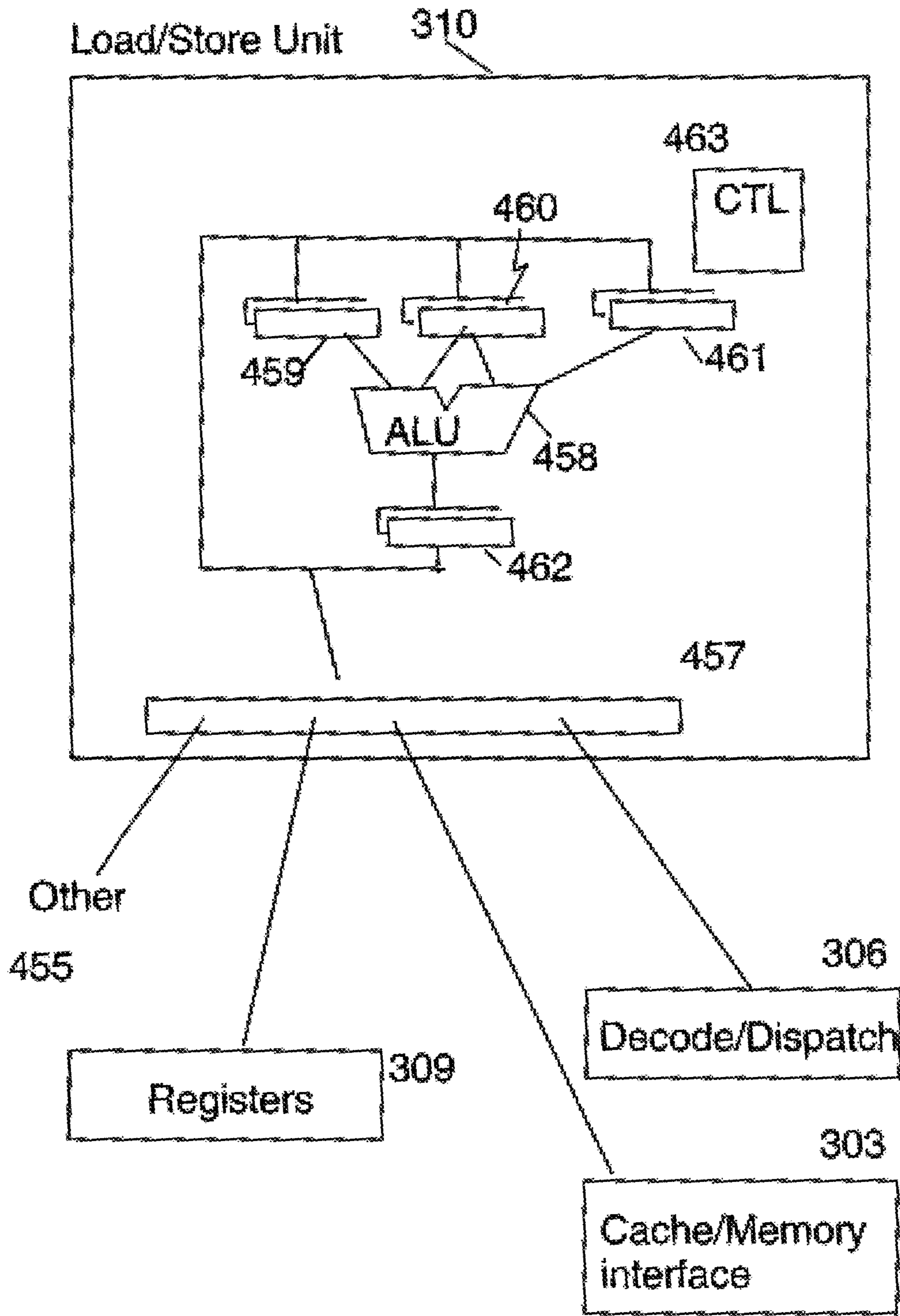
FIG. 4C Prior Art
