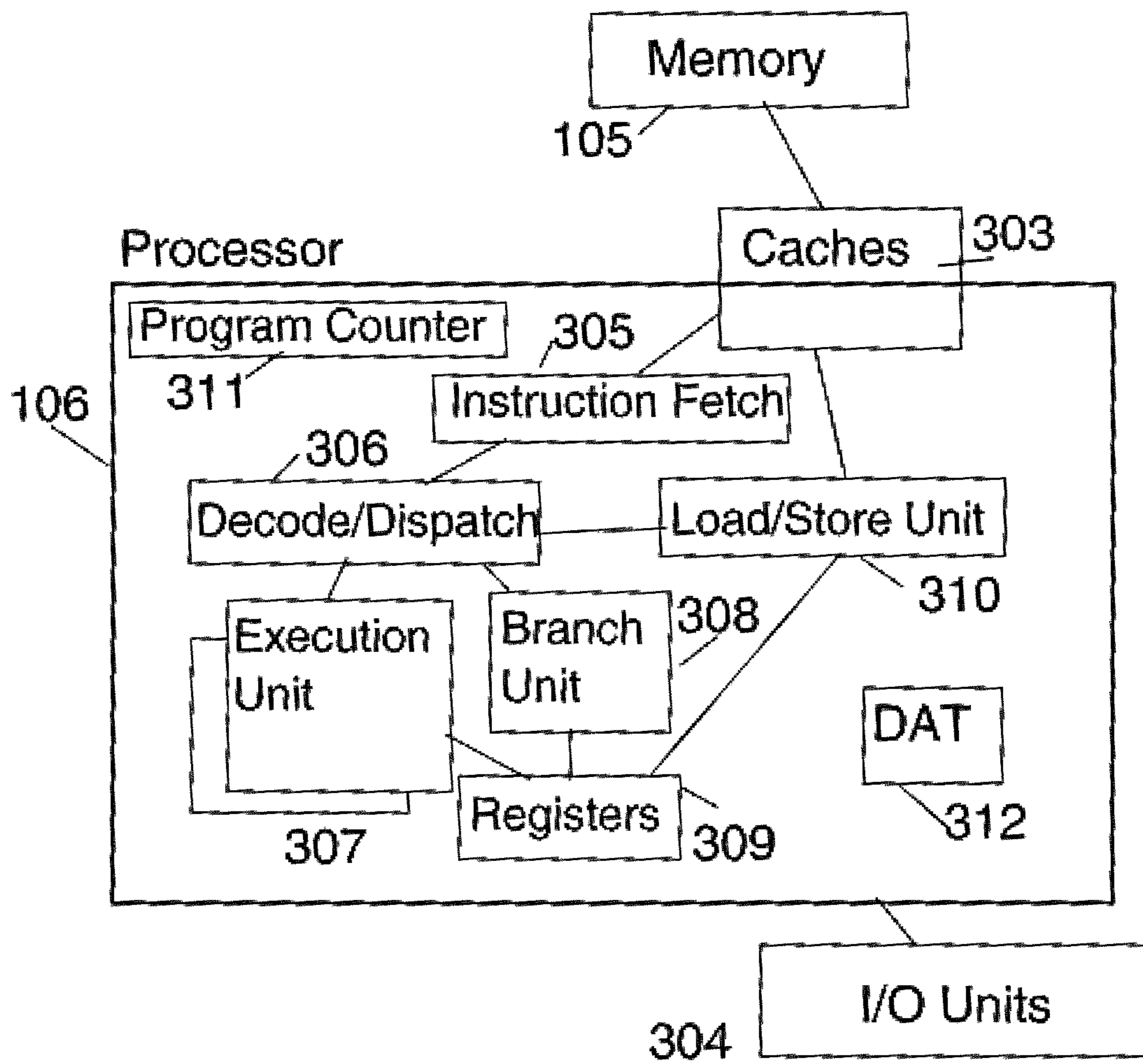
FIG. 3 Prior Art
