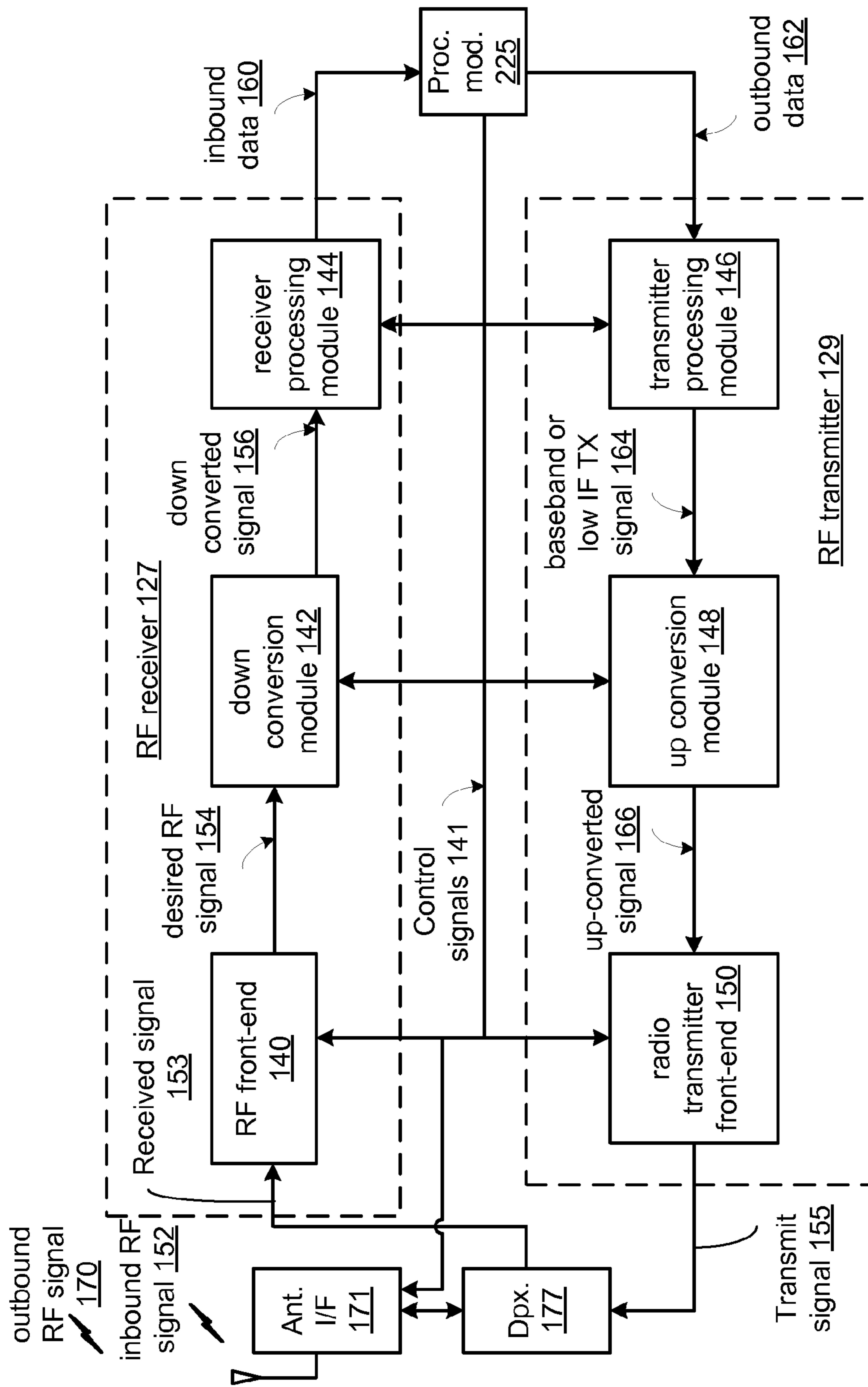
RF transceiver 123
