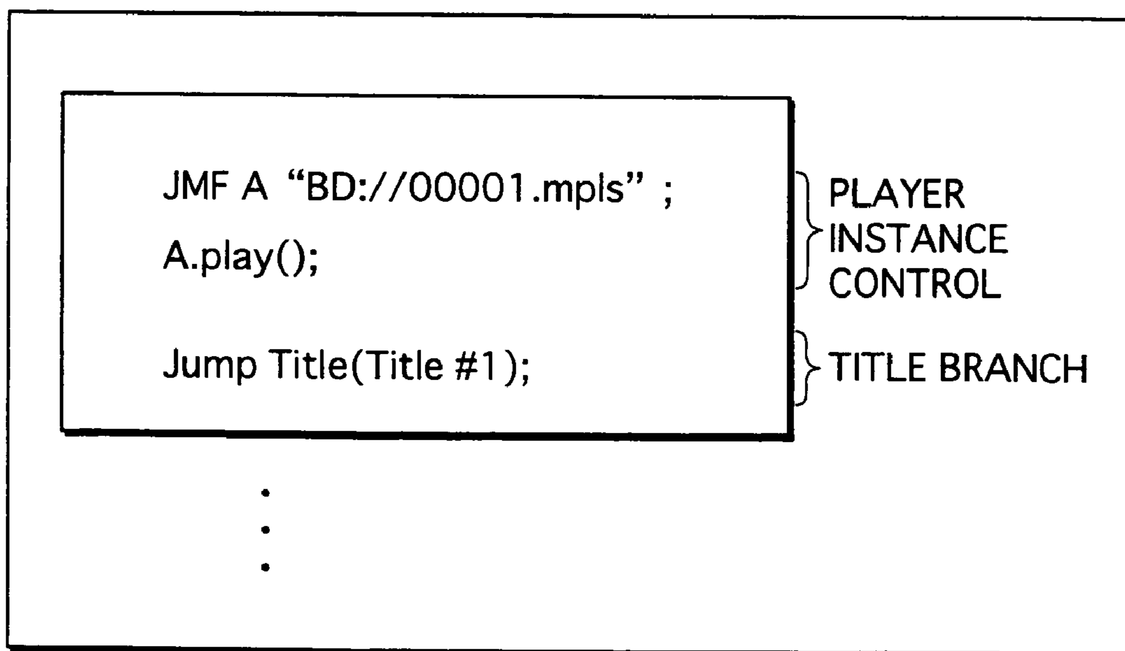
xlet PROGRAM
