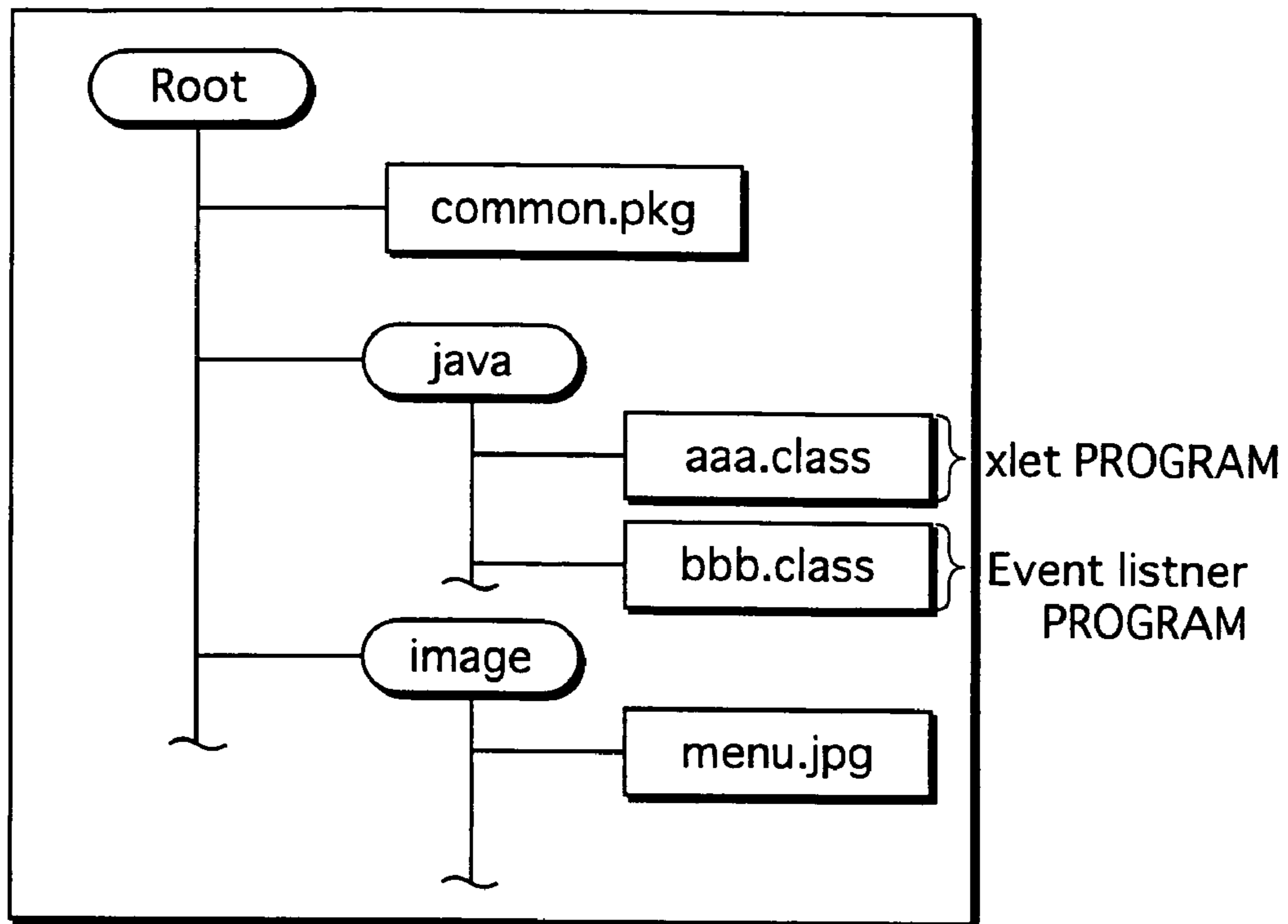
JAR FILE
