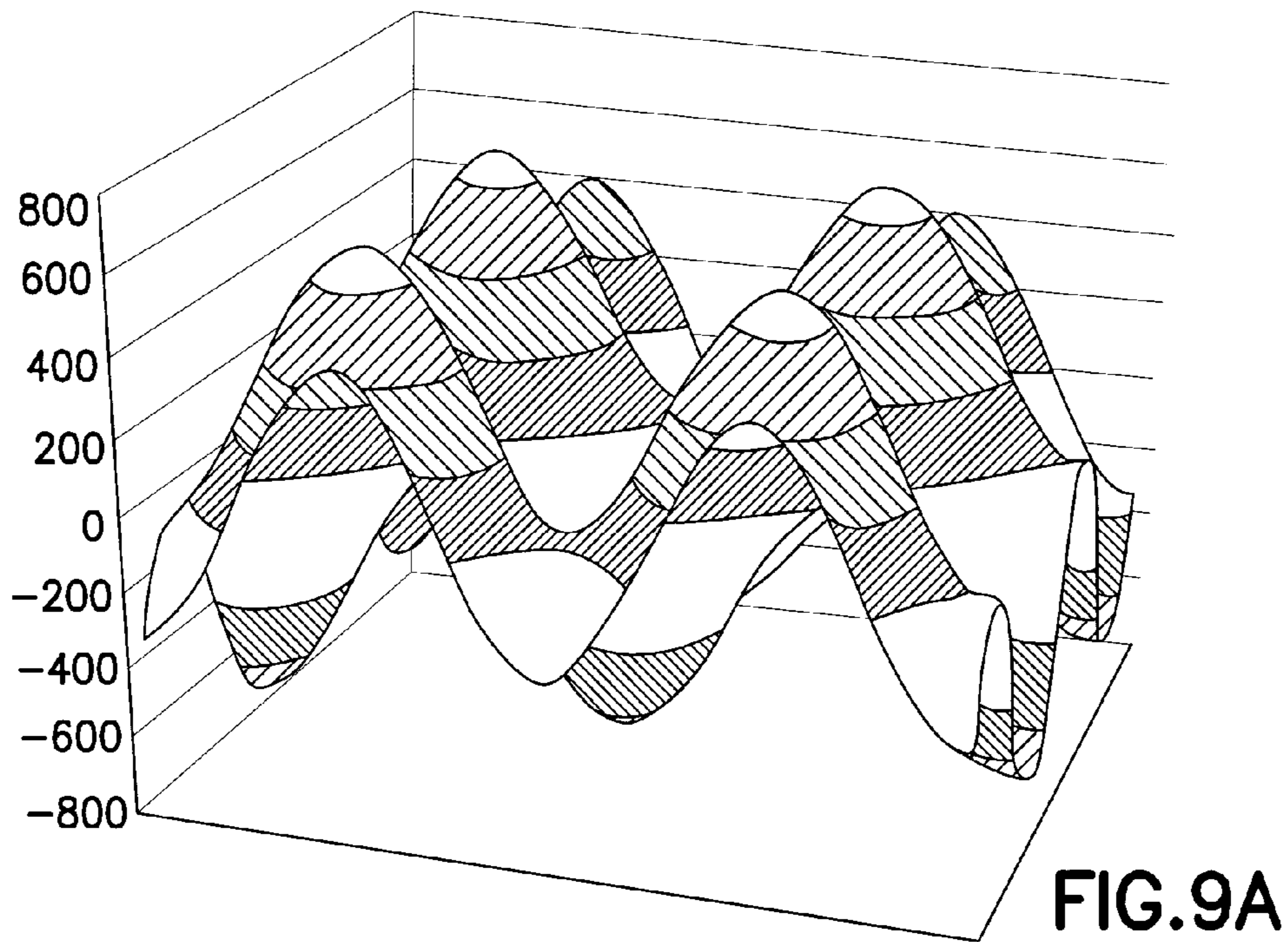
PERPENDICULAR FIELD SENSING (NORMAL) B_y(x,z)
