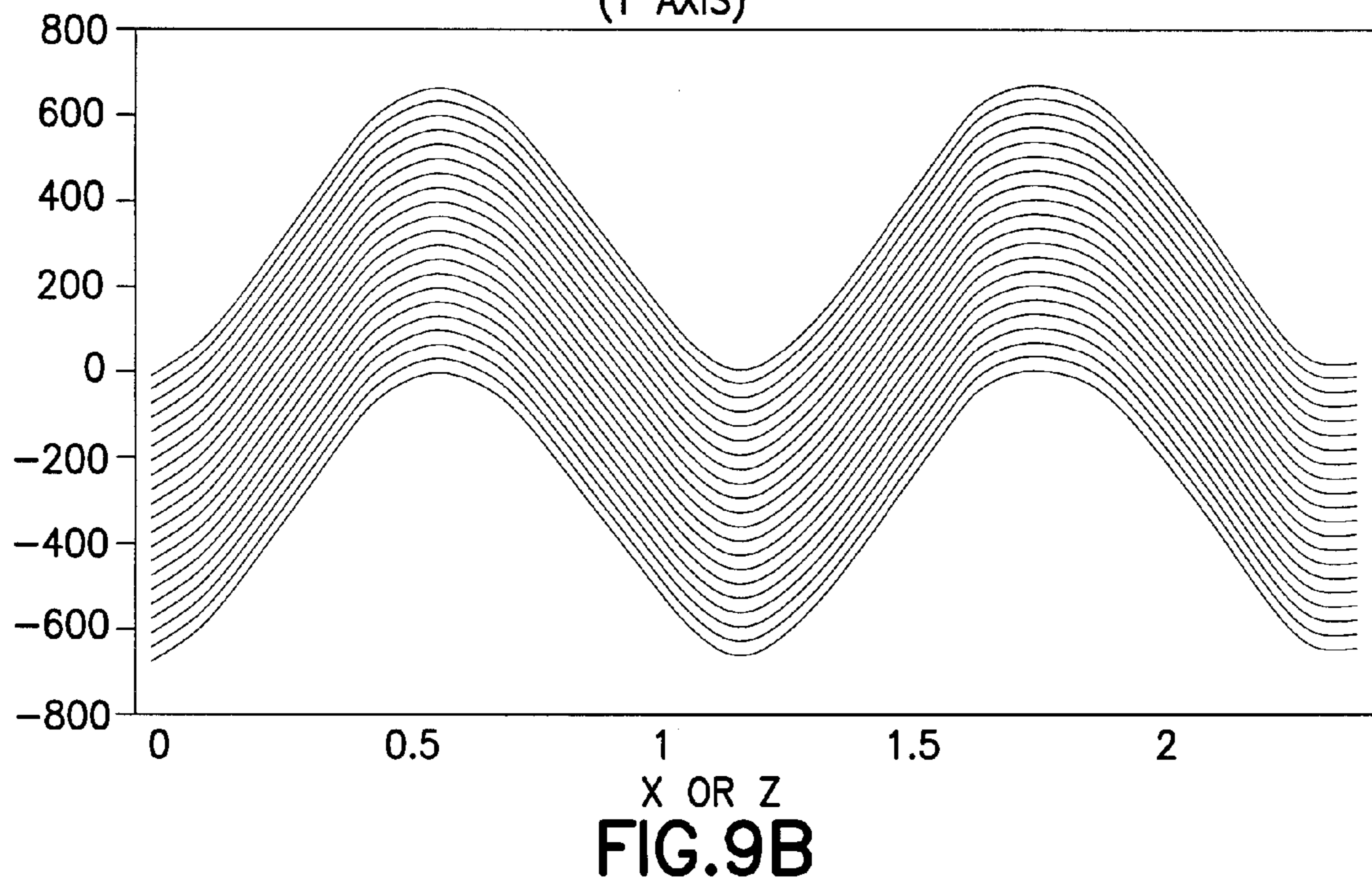
HALL SENSOR OUTPUT (Y AXIS)
