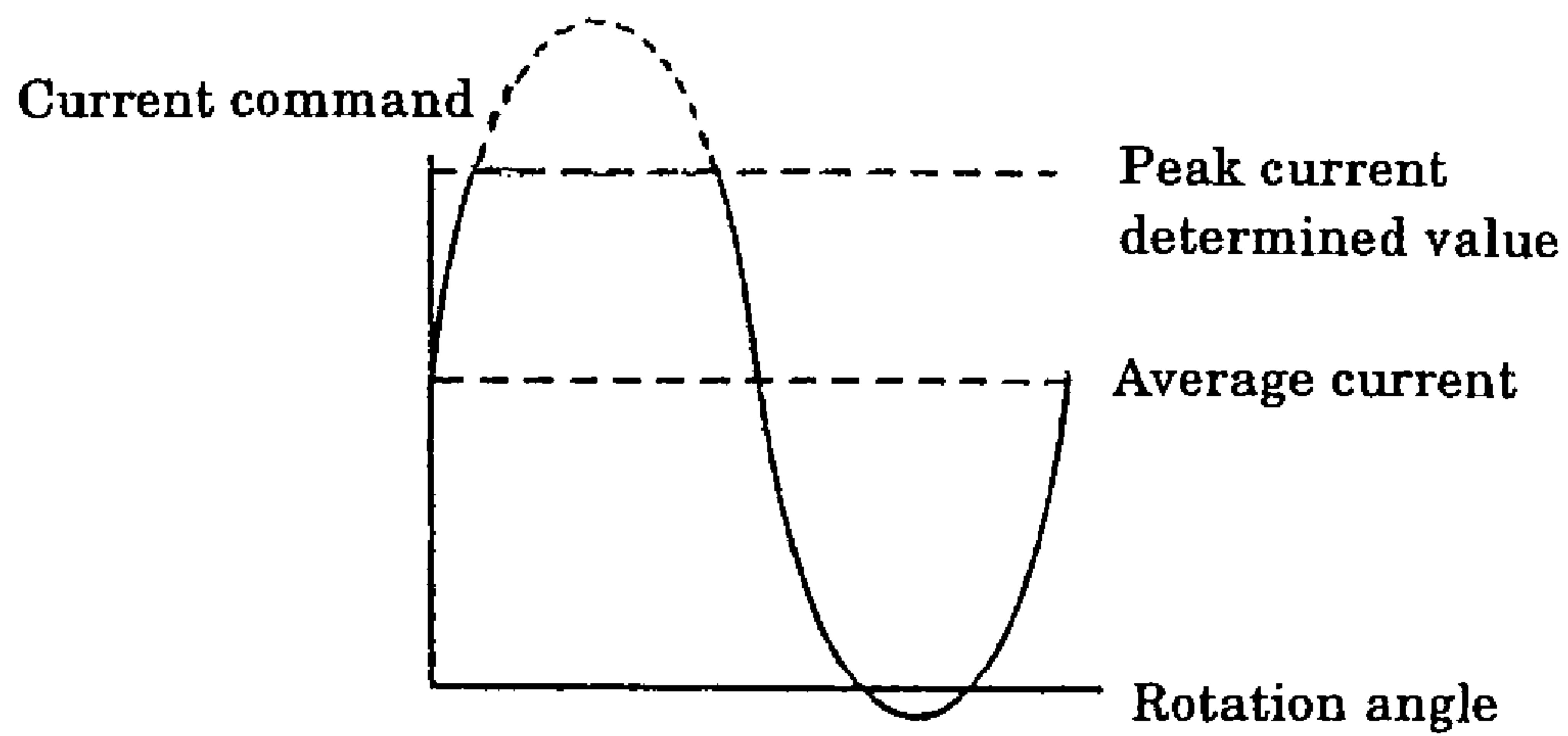
(B) Clipped current command
