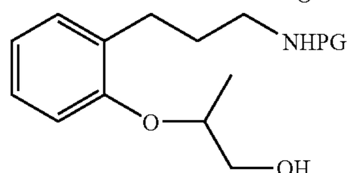
T33a [(R)-isomer] T33b [(S)-isomer]
