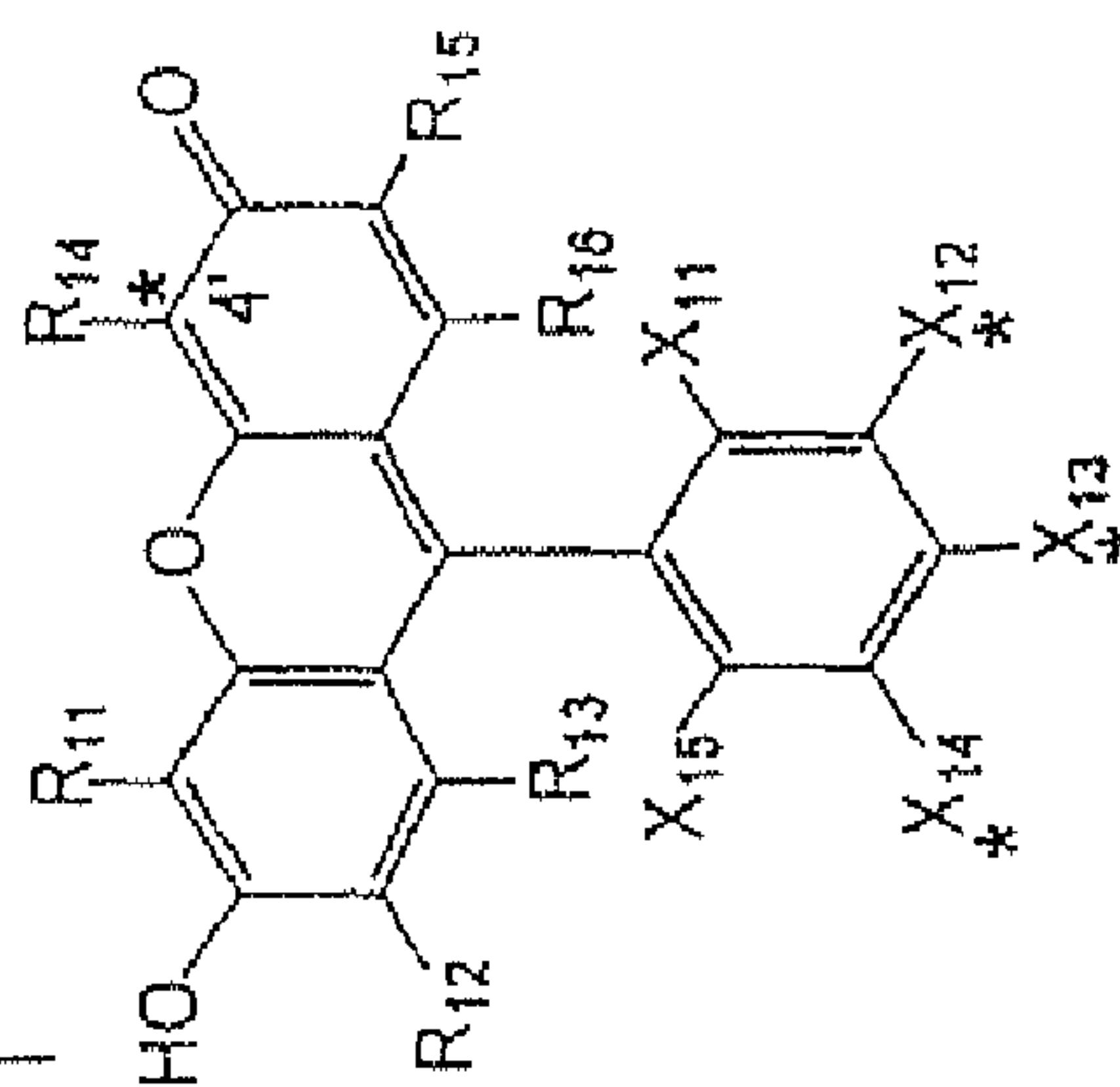
FLUORESCIEIN
