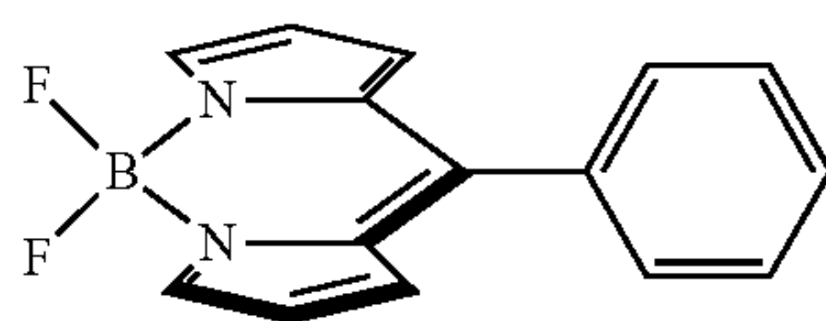
5-phenyldipyrrinatoboron difluoride
