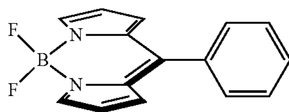
5-phenyldipyrrinatoboron difluoride
