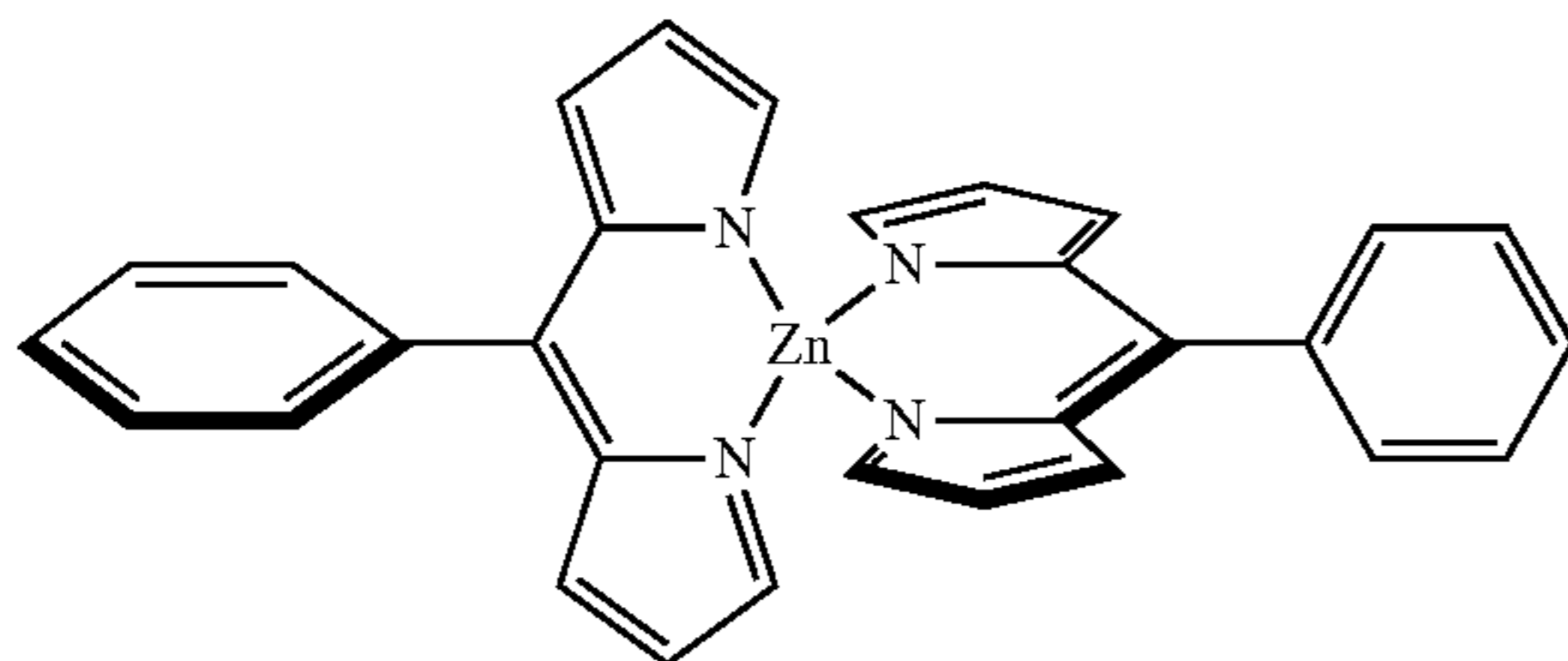
bis(5-phenyldipyrrinato)zinc(II)
