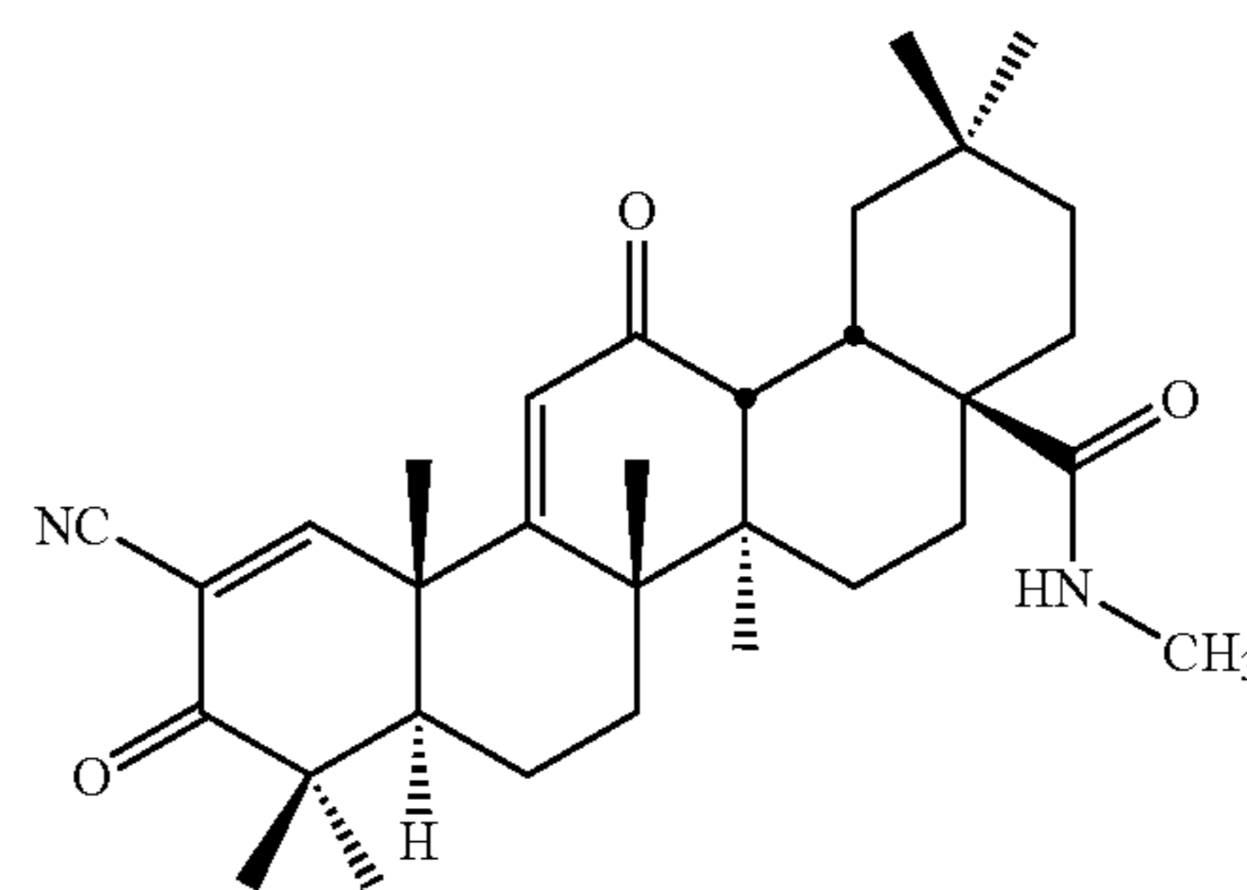
CDDO-MA (TP-224)
