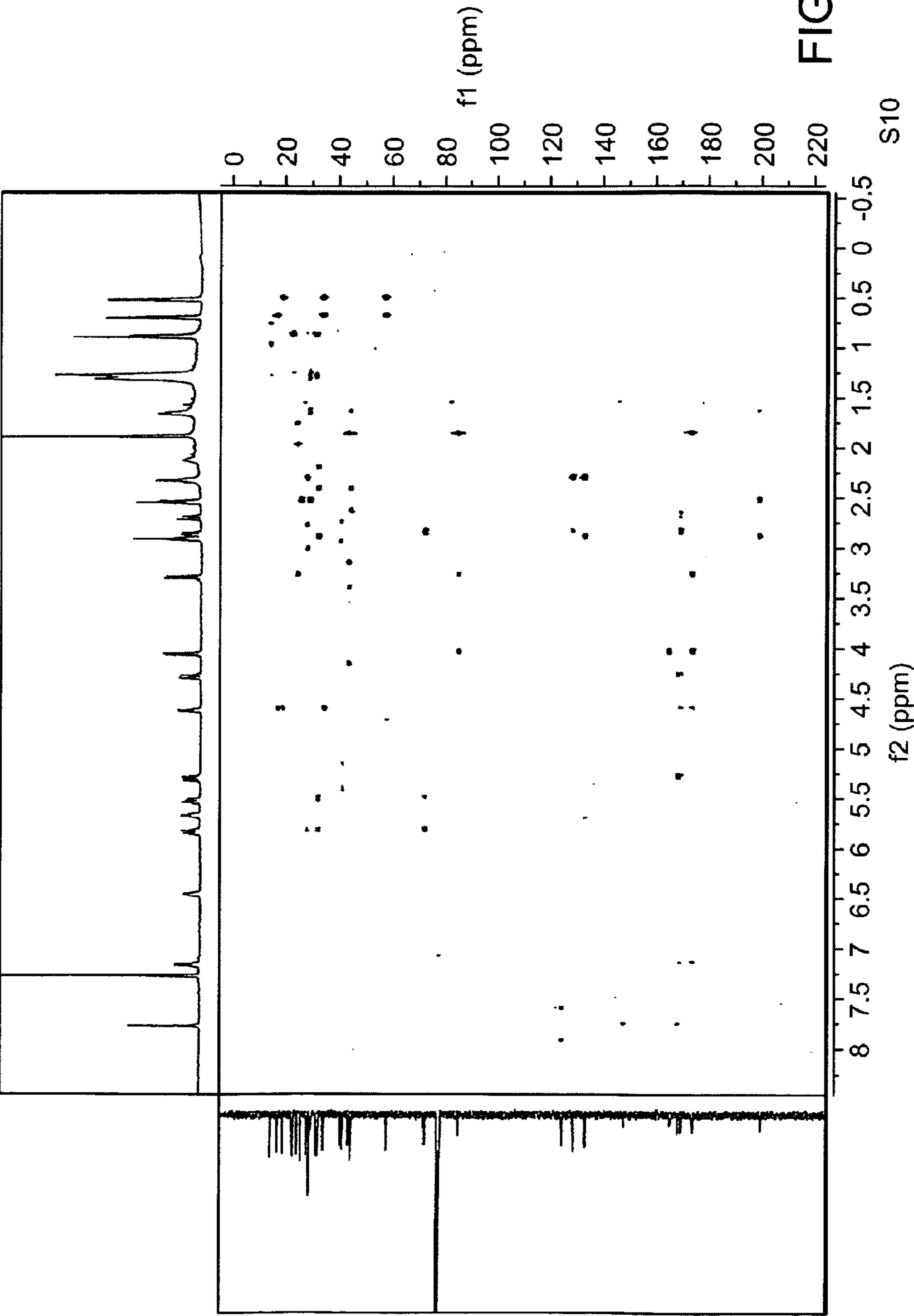
HMBC Spectrum of Largazole (1) in CDCl 3 (optimized for ^nJ_{\text{CH}} = 7 \text{ Hz} )
