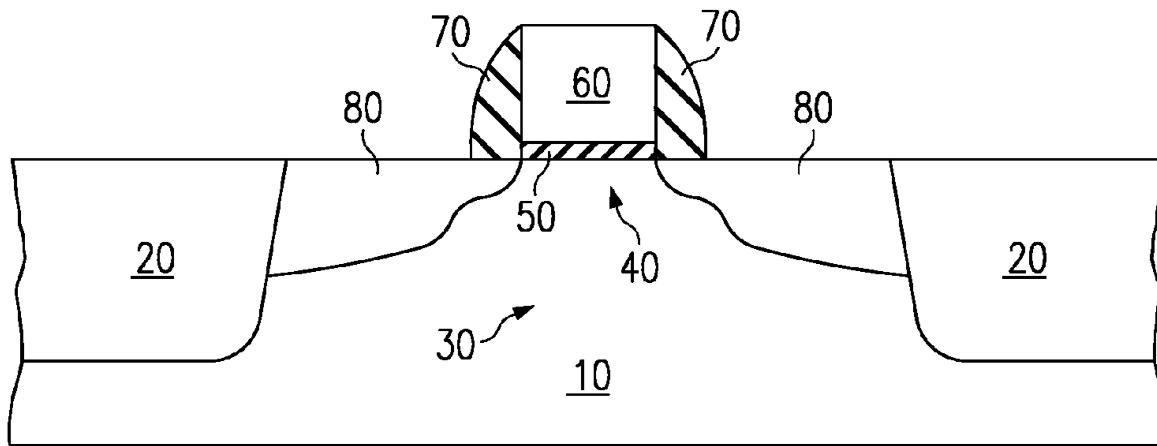
FIG. 1 (PRIOR ART)
