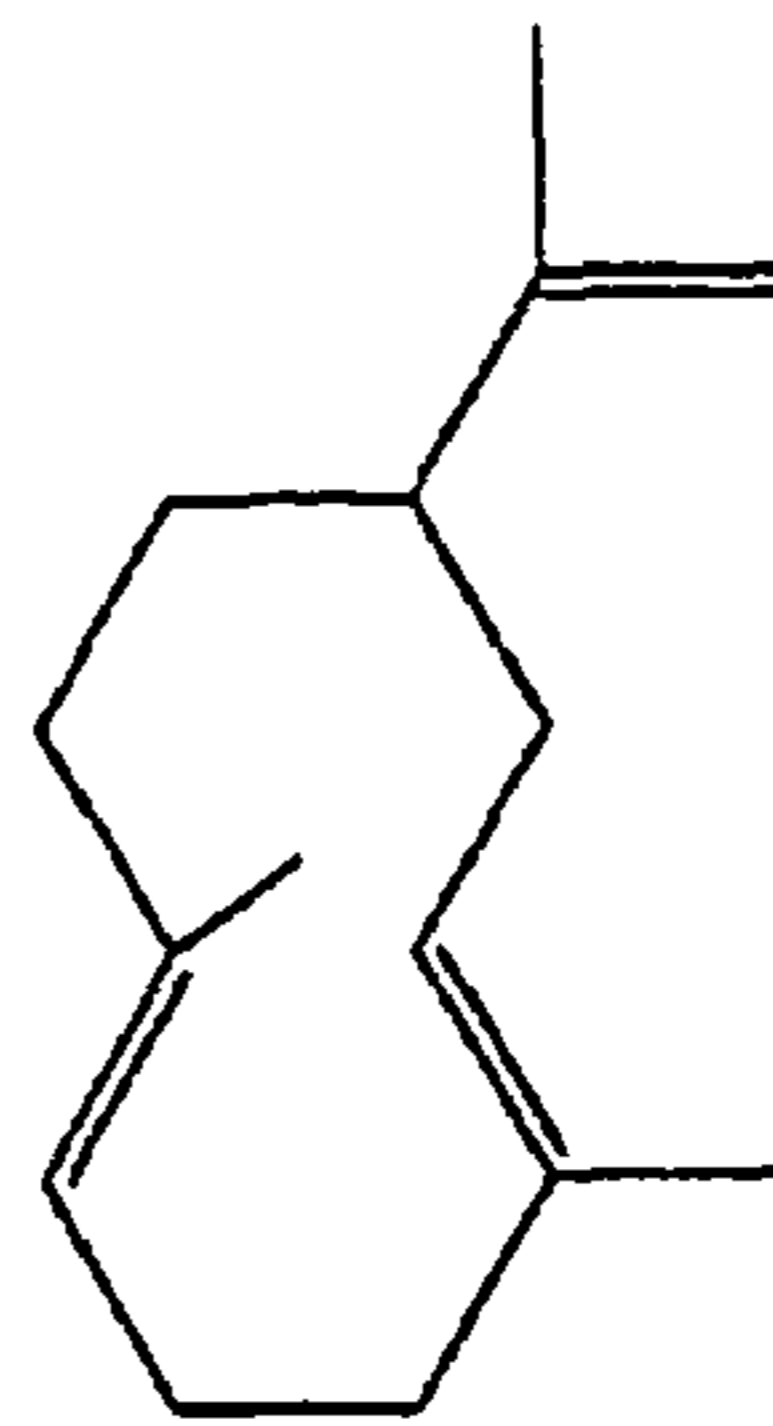
(+)-GERMACRENE A
