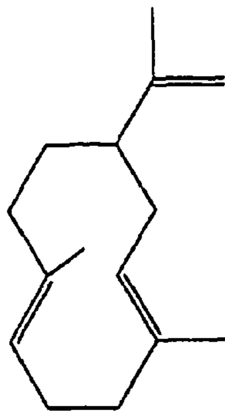
(+)-GERMACRENE A
