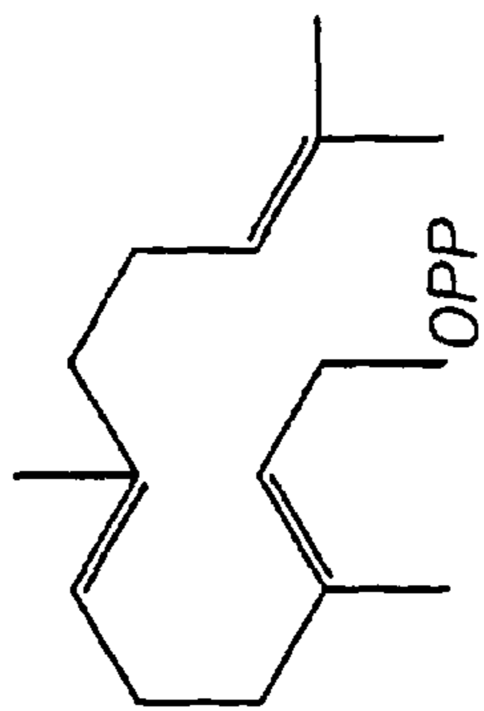
FARNESYL DIPHOSPHATE
