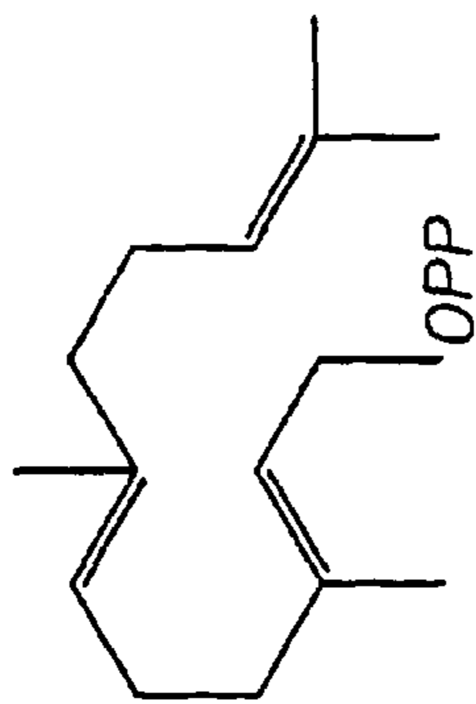
FARNESYL DIPHOSPHATE
