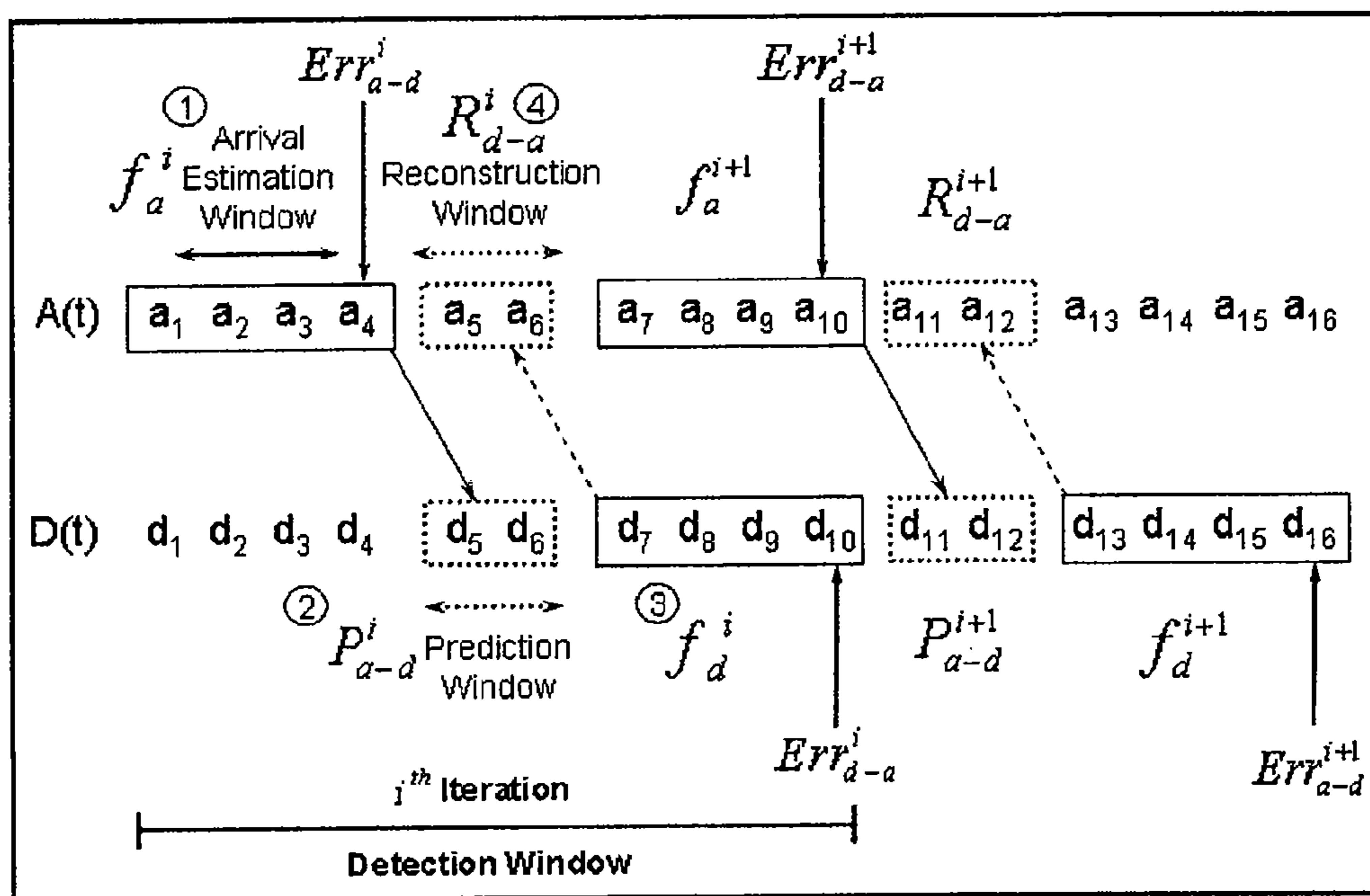
Figure 2. Diagram showing the four significant steps in SYN Flooding detection algorithm.
