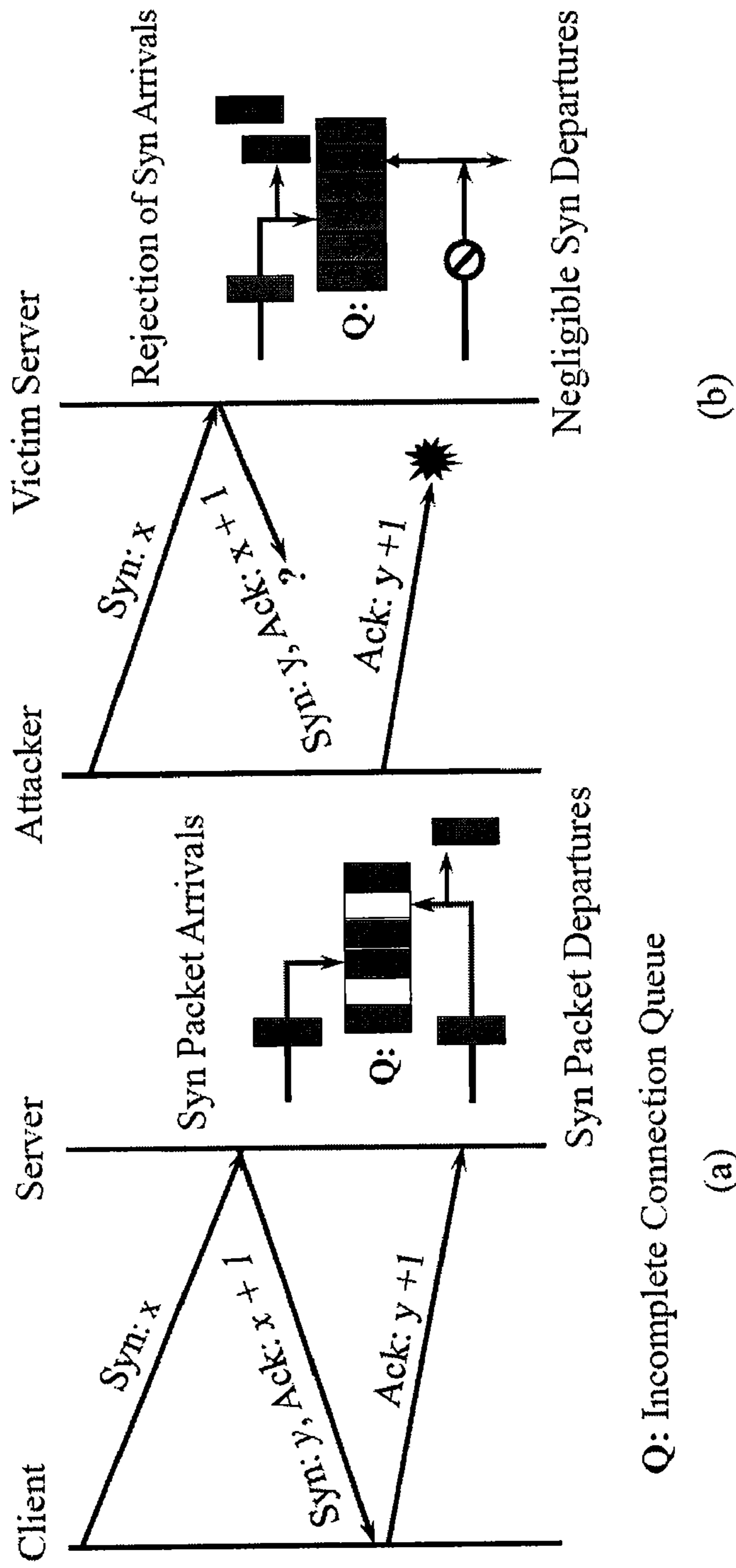
Figure 1(a) illustrates a normal TCP connection establishment, while Figure 1(b) illustrates an attack situation.
