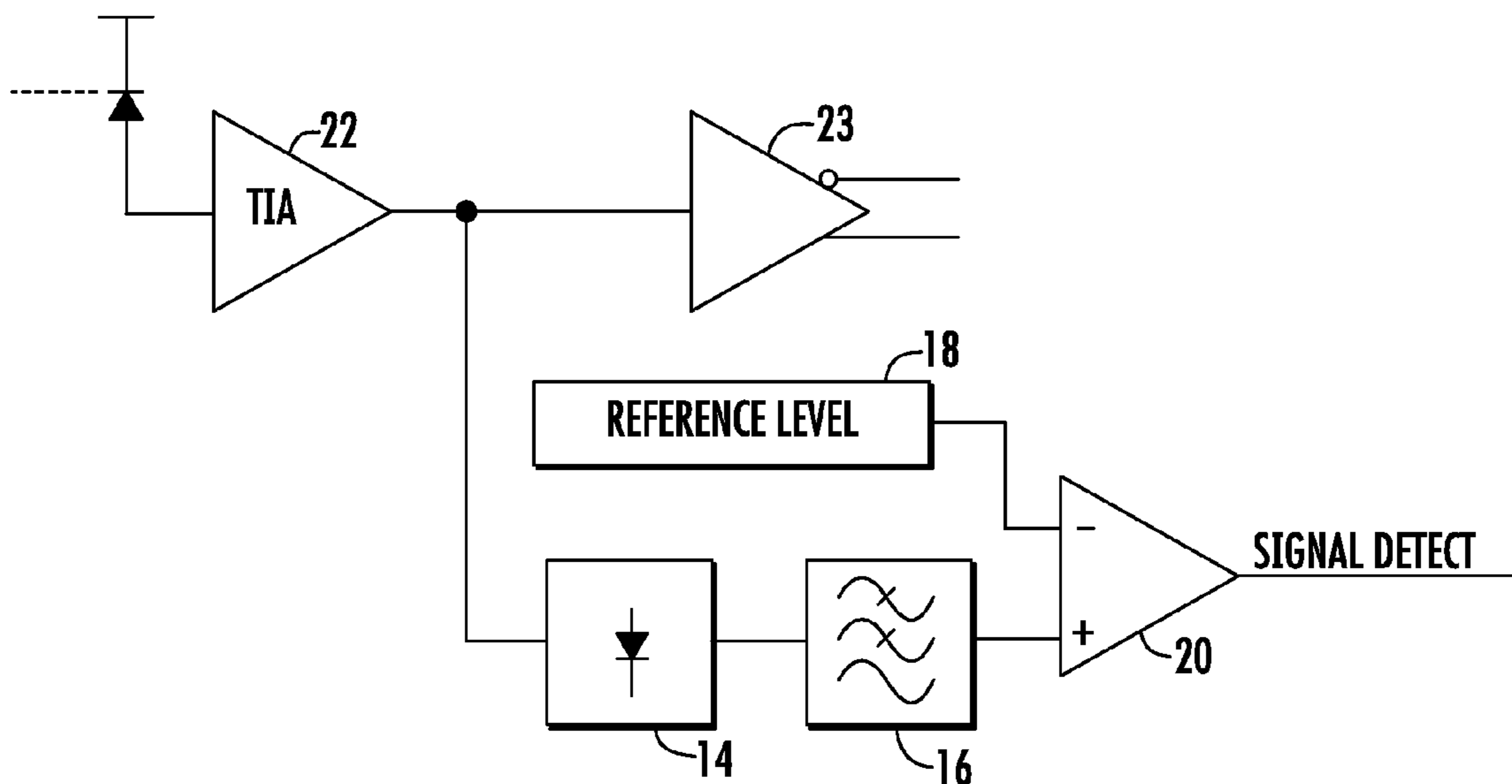
FIG. 2 (PRIOR ART)
