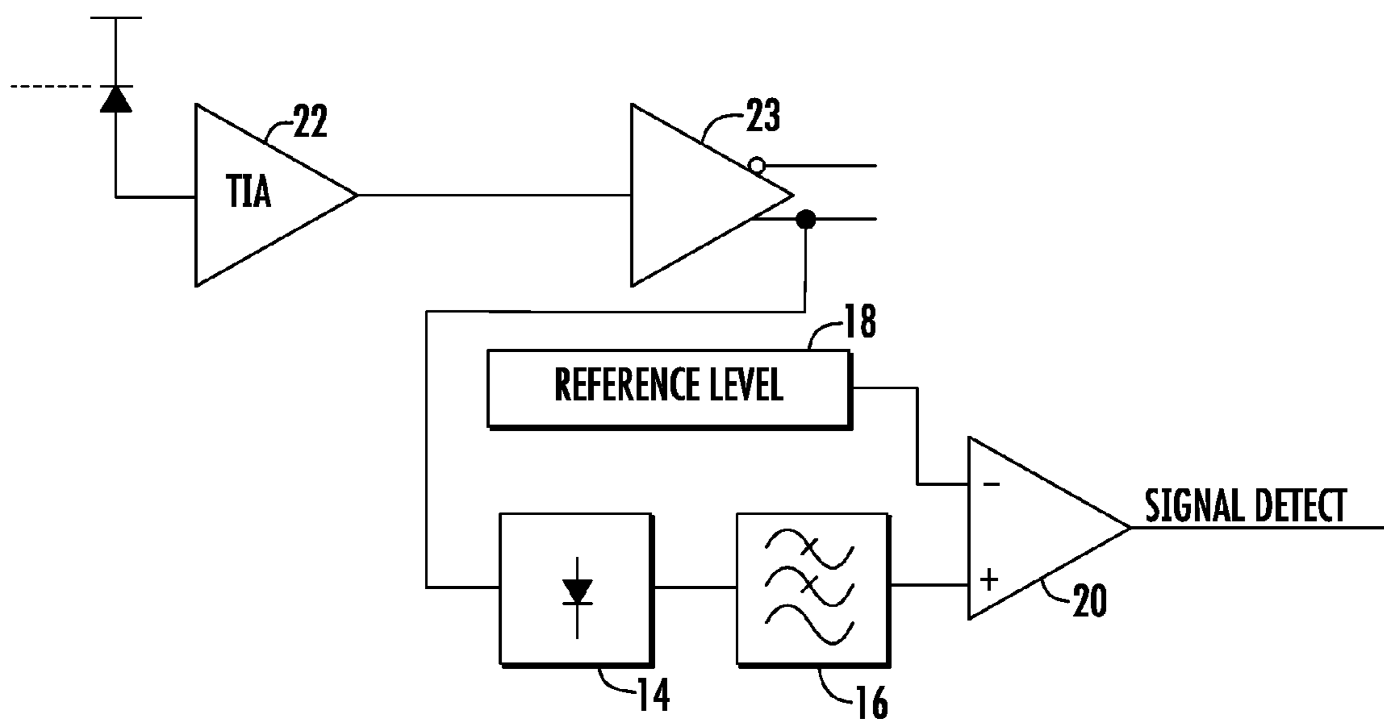
FIG. 3 (PRIOR ART)
