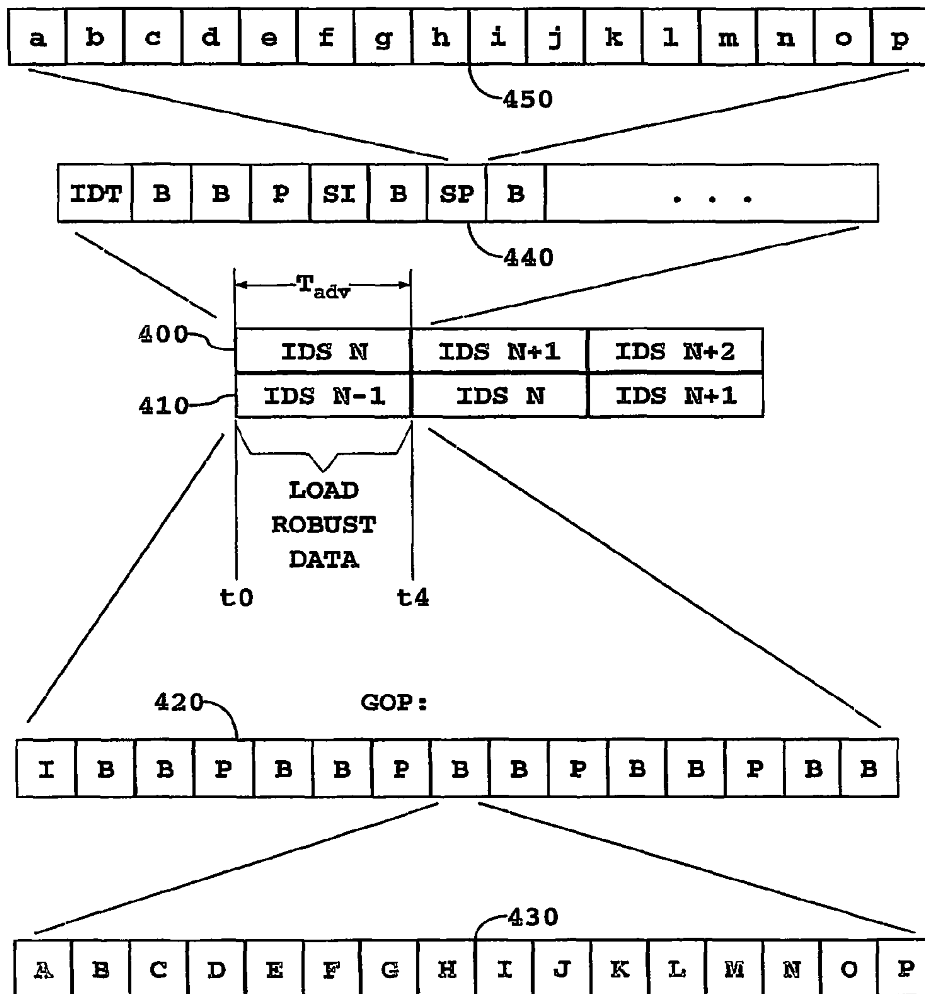
Fig. 4 GOP Streams
