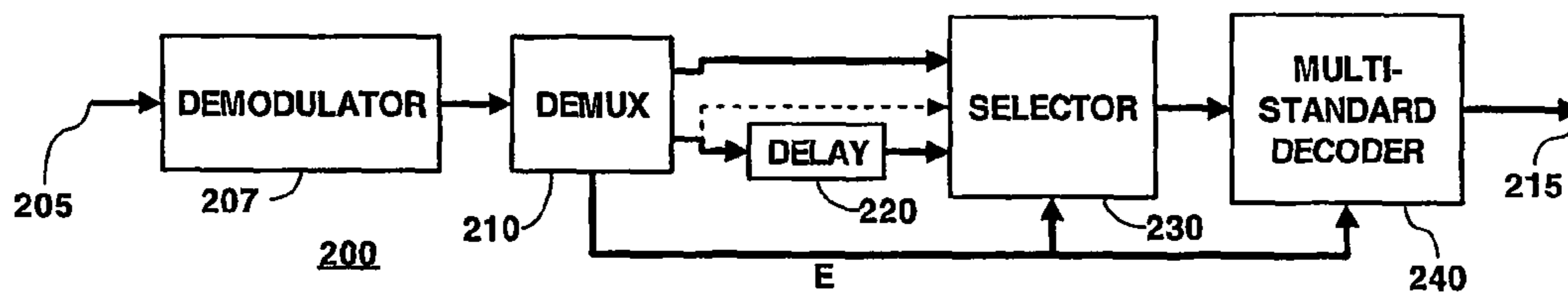
Fig. 2 Receiver
