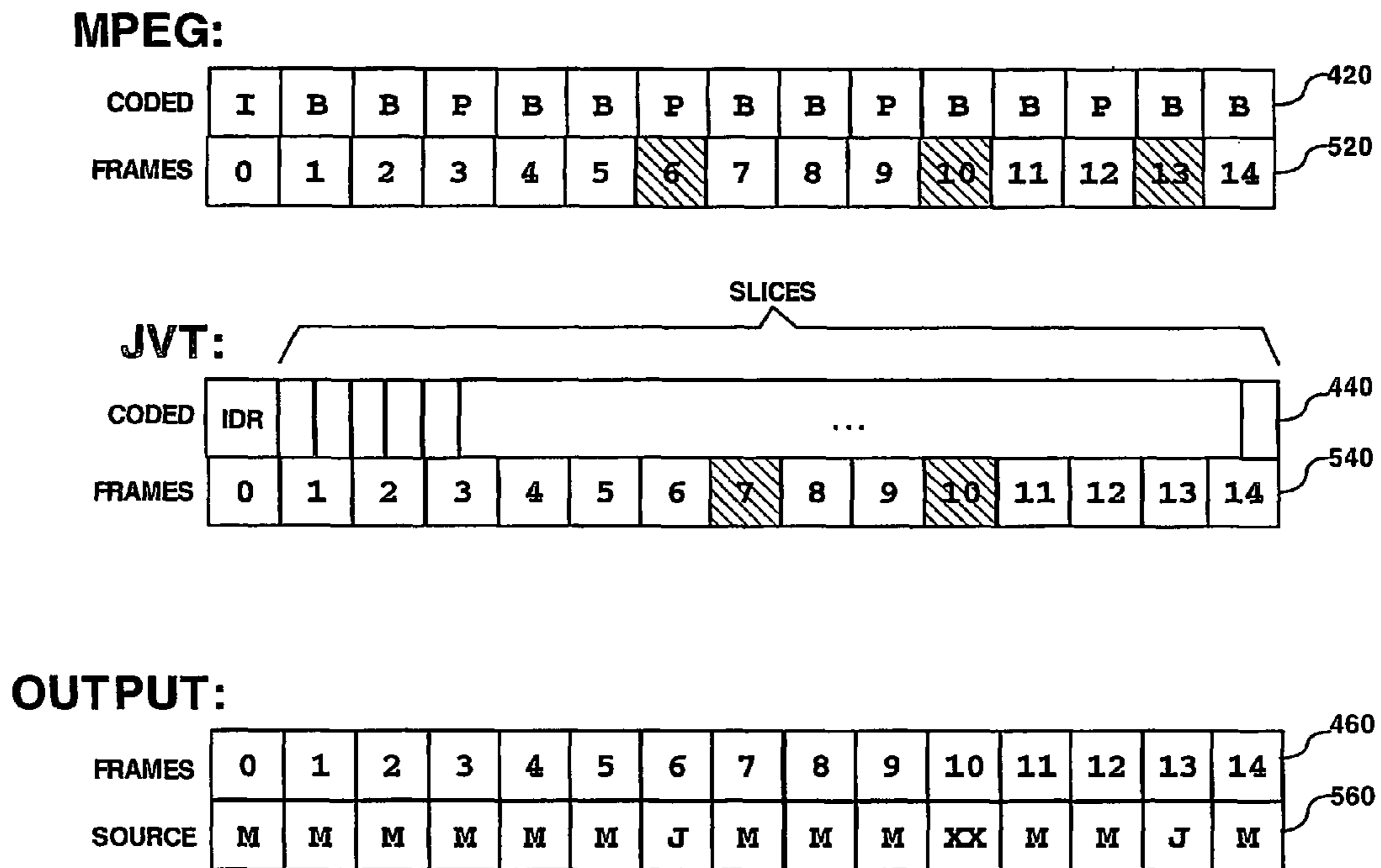
Fig. 7 Picture layer streams
