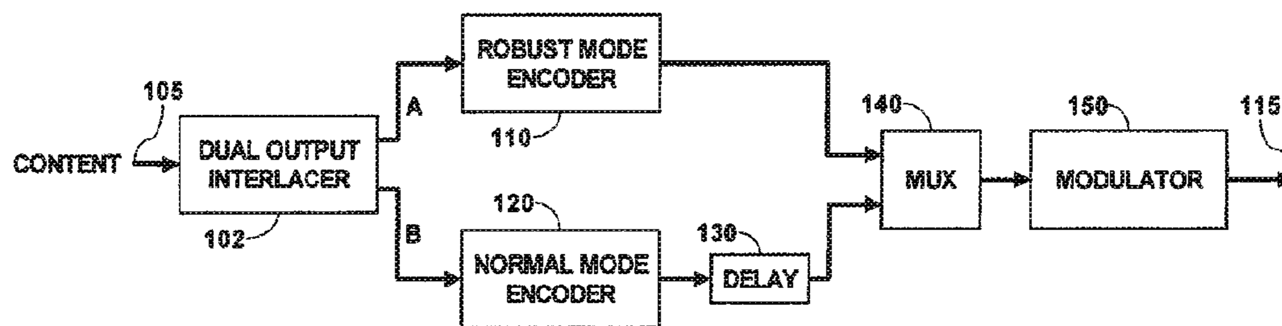
Fig. 11 Dual interlace transmitter
