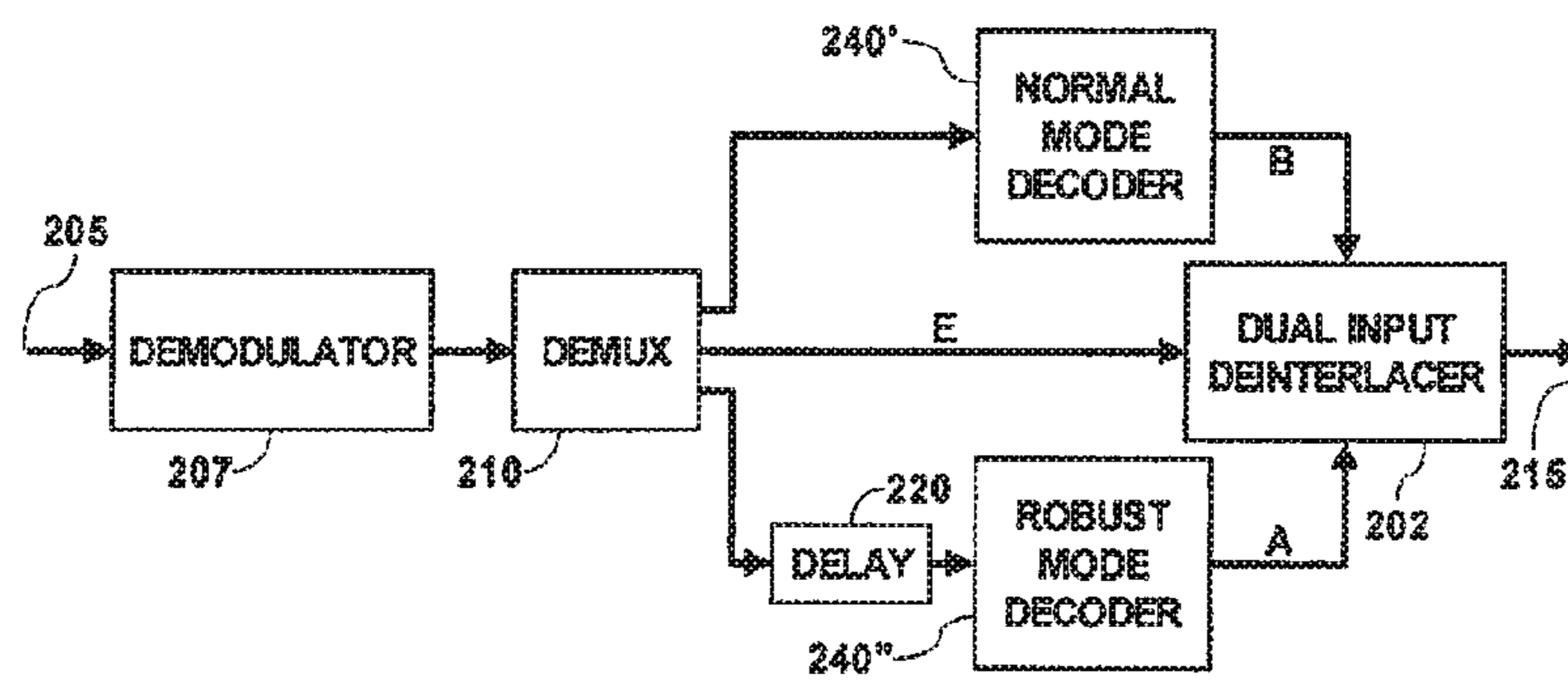
Fig. 12 Dual interlace receiver
