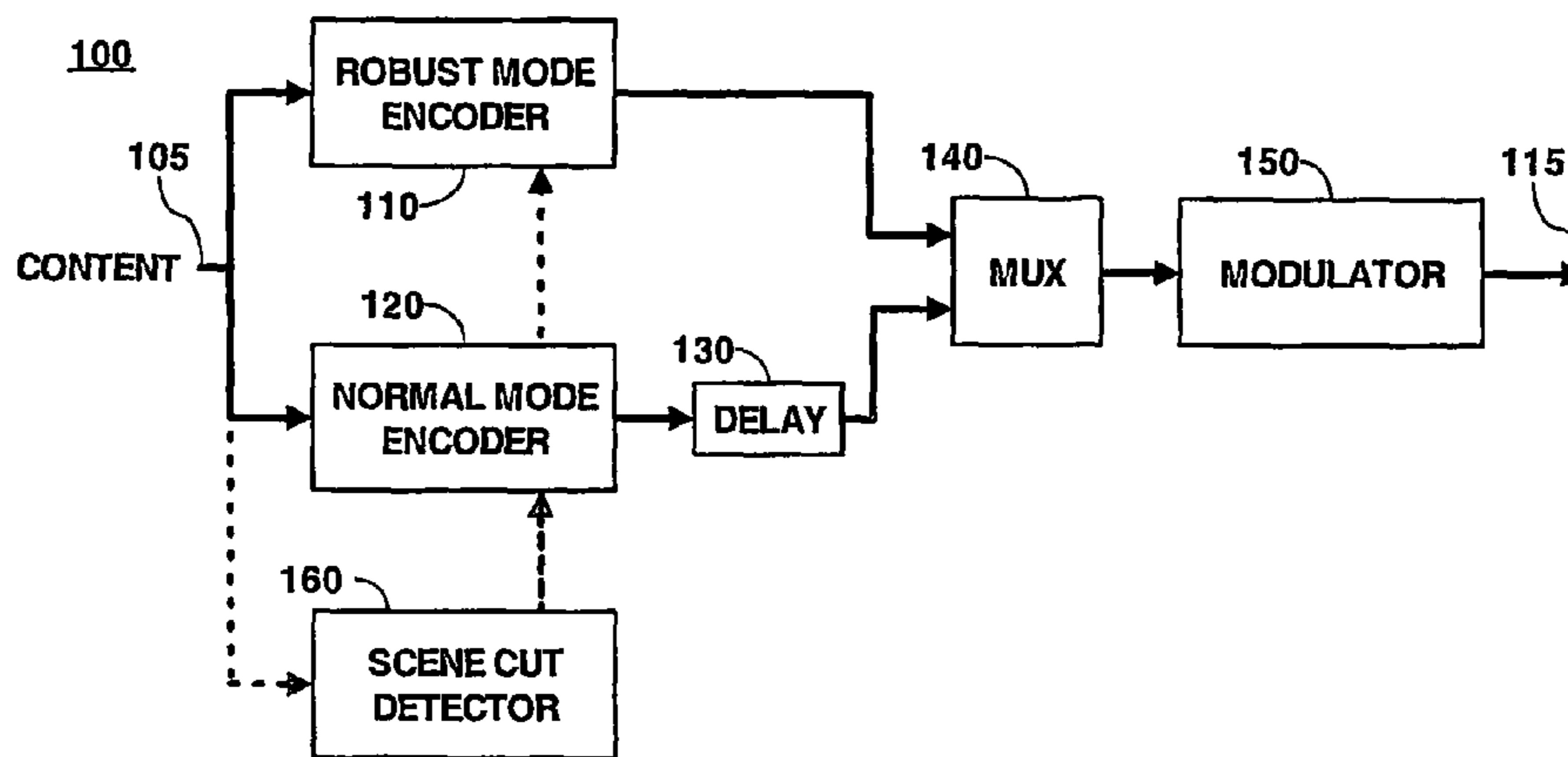
Transmitter
