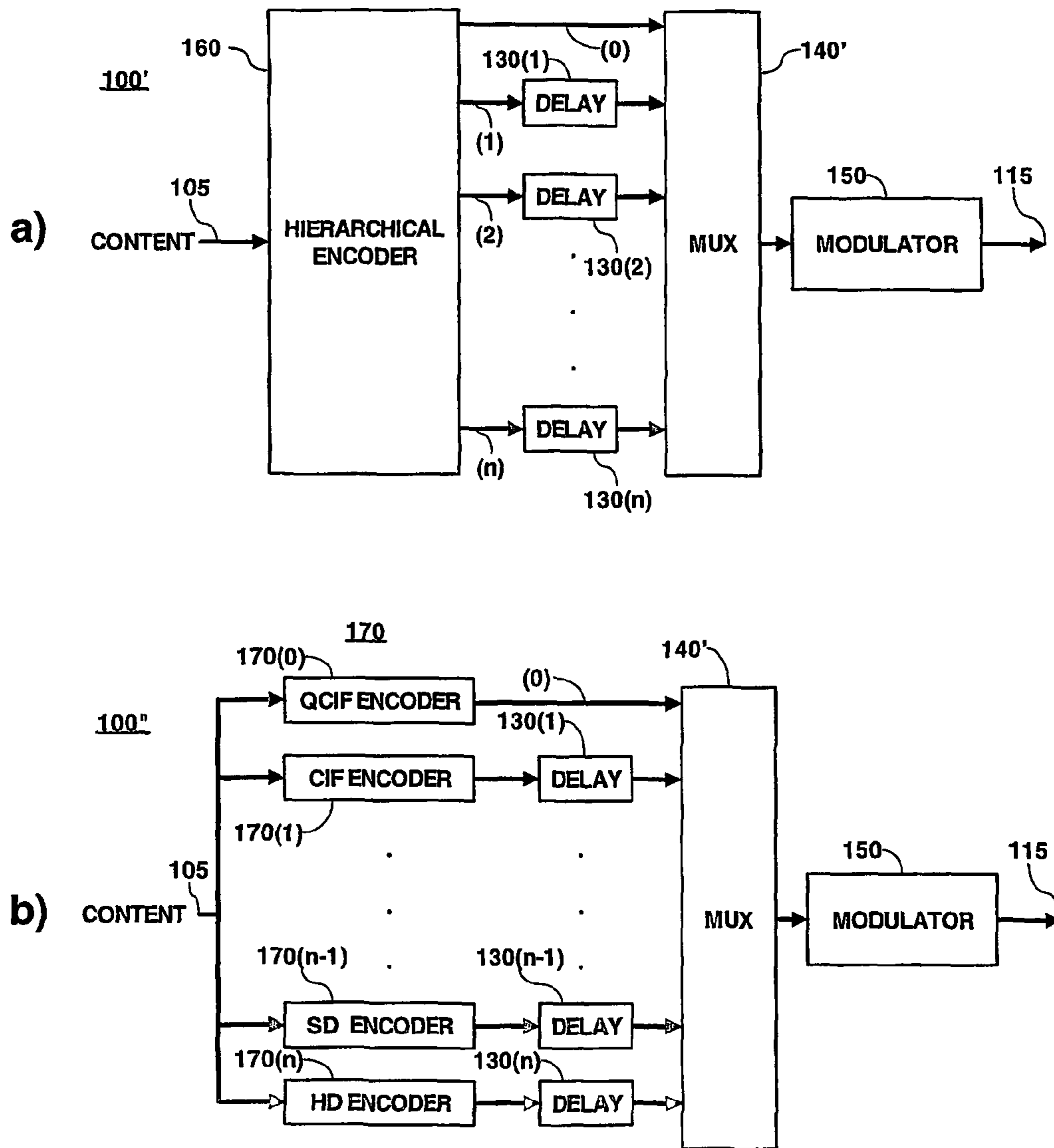
Fig. 9 Multiresolution transmitter
