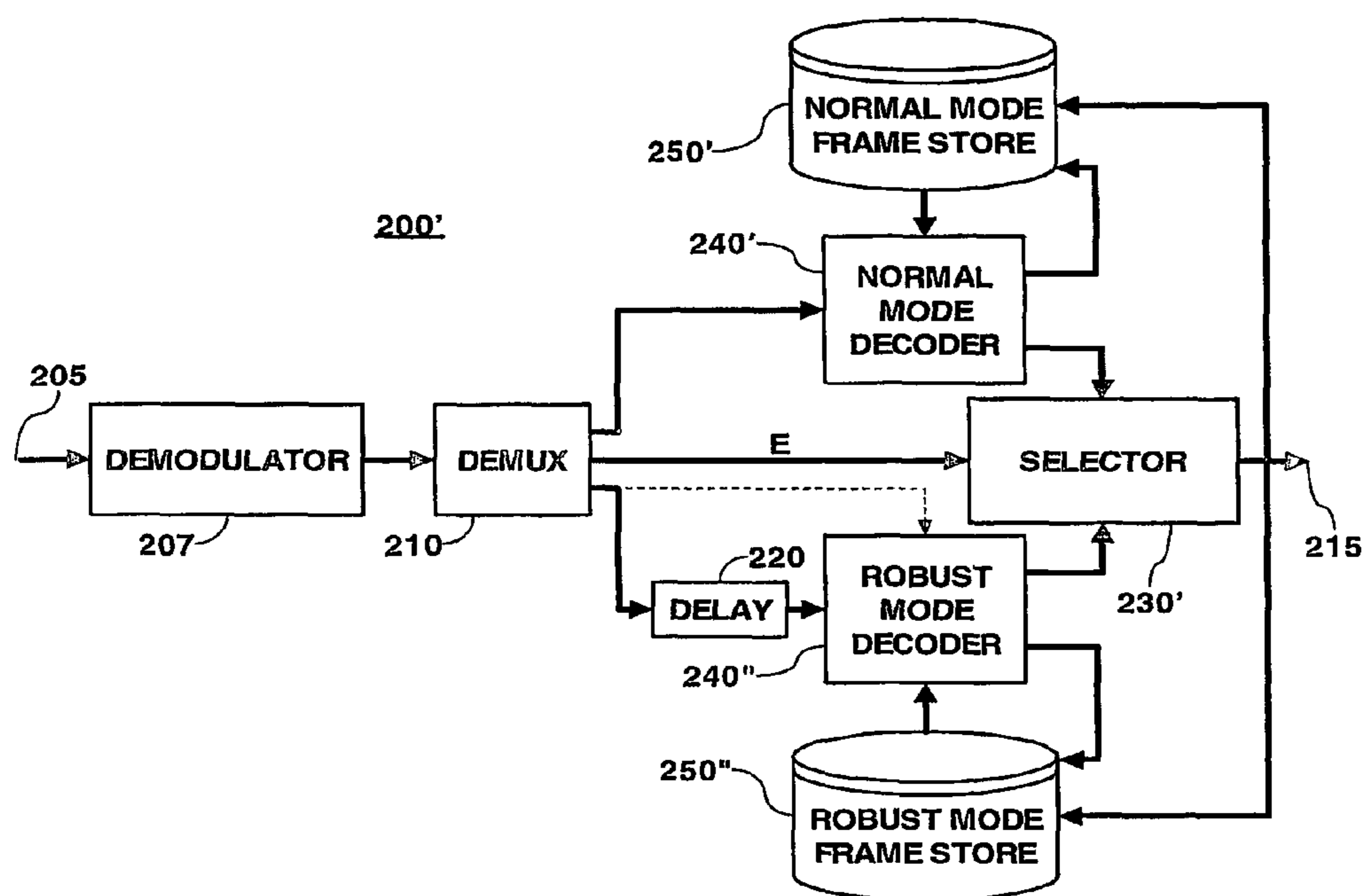
Fig. 6 Picture layer receiver
