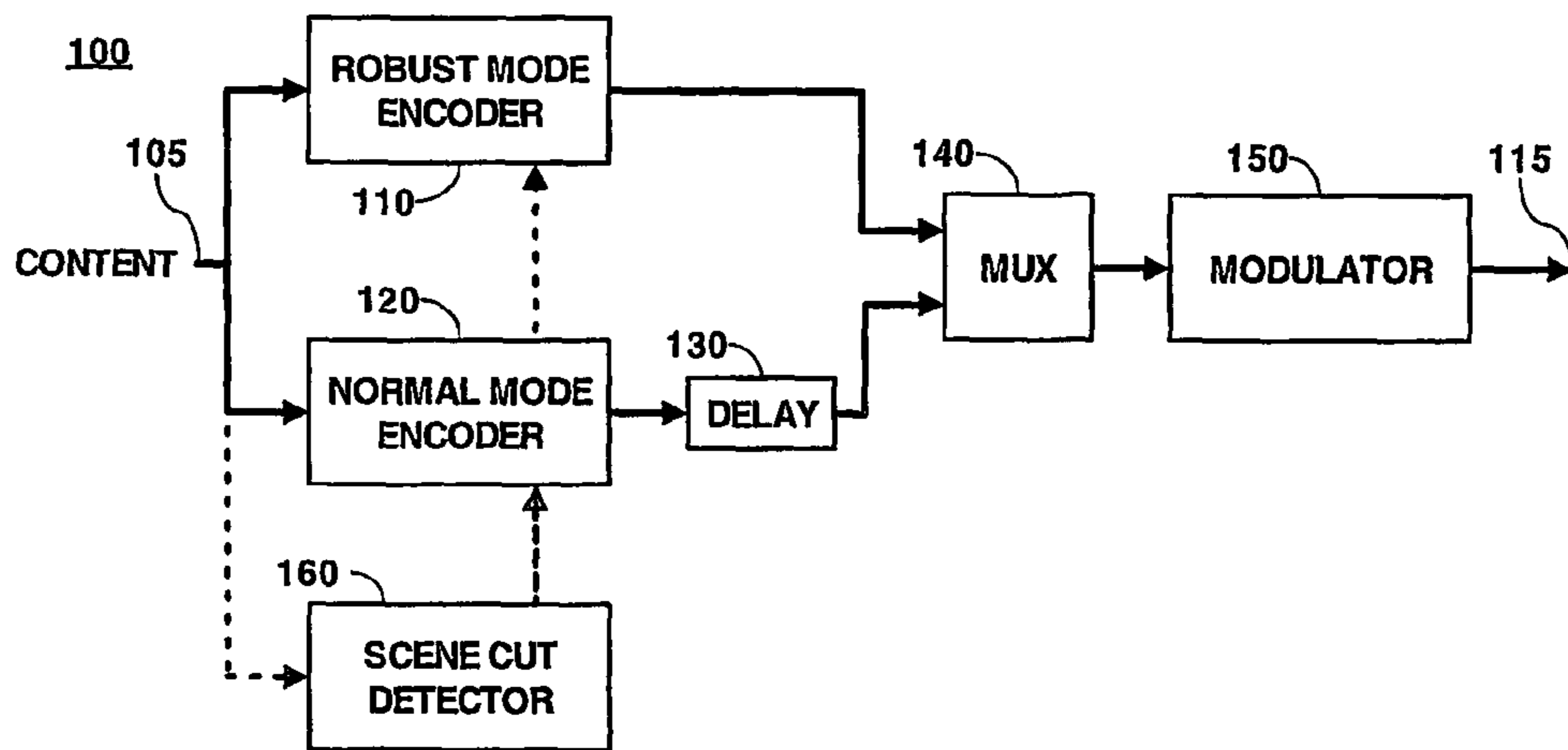
Fig. 1 Transmitter
