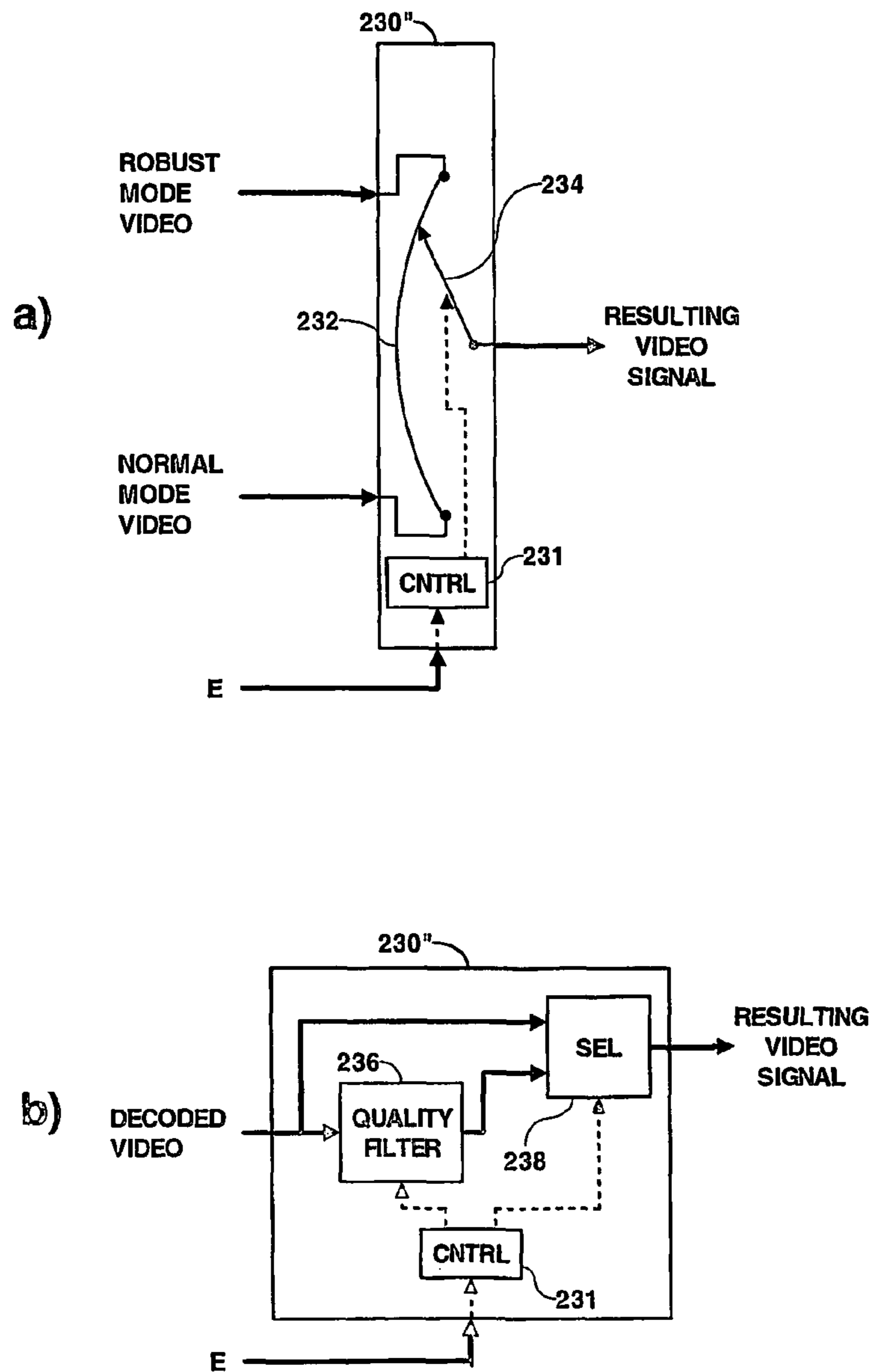
Fig. 5 Smoothing selector
