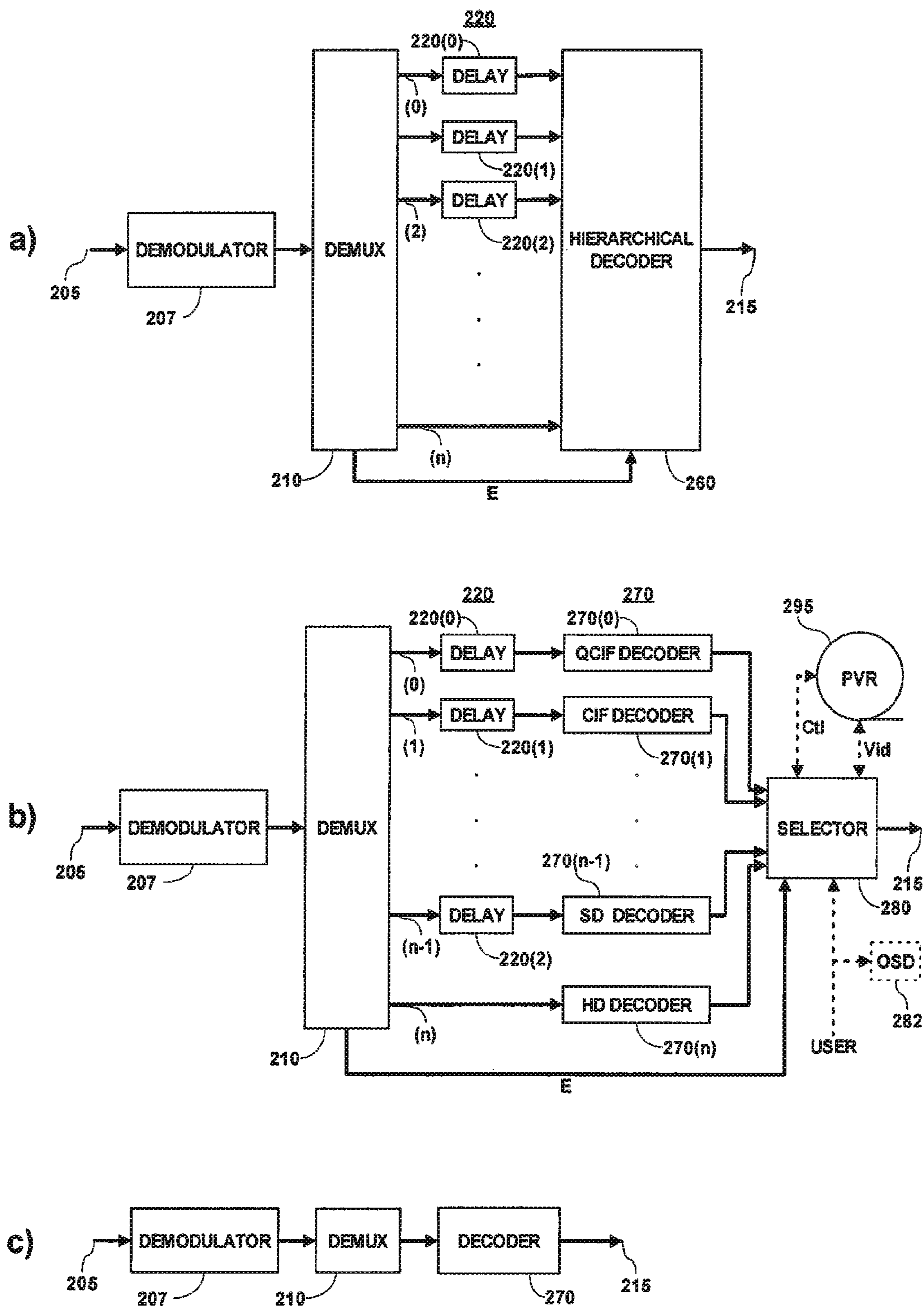
Fig. 10 Multiresolution receiver
