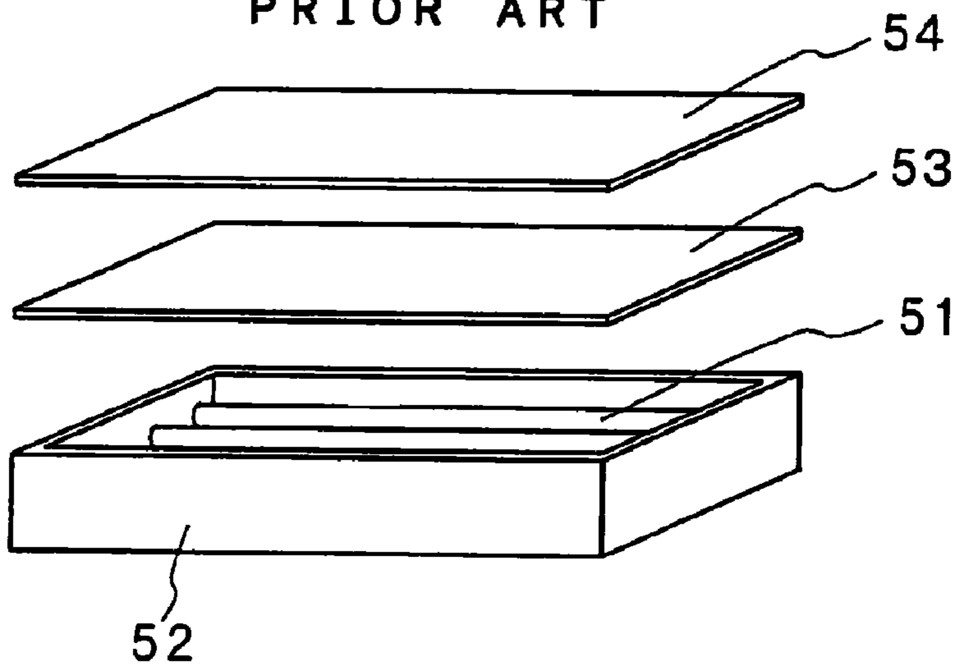
FIG. 8 PRIOR ART
