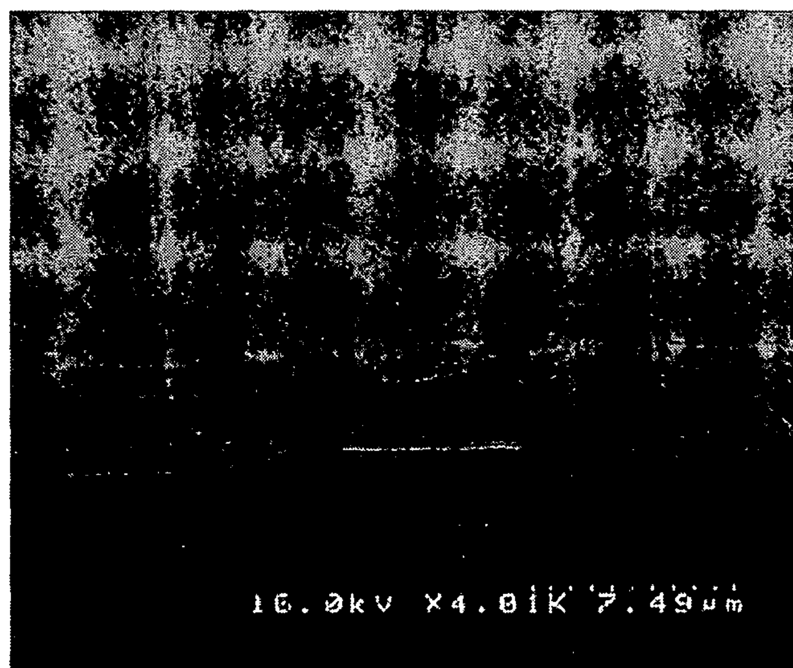
CROSS-SECTIONAL SEM PICTURE OF POSITIONING MARK IN PERIPHERY (W IS OXIDIZED)
