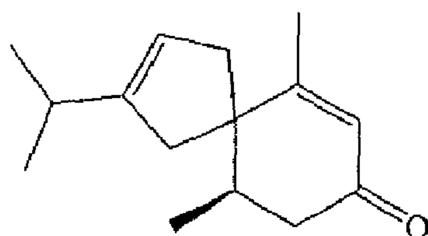
2-isopropyl-6,10-dimethyl-spiro[4.5]deca-2,6-dien-8-one (3)
