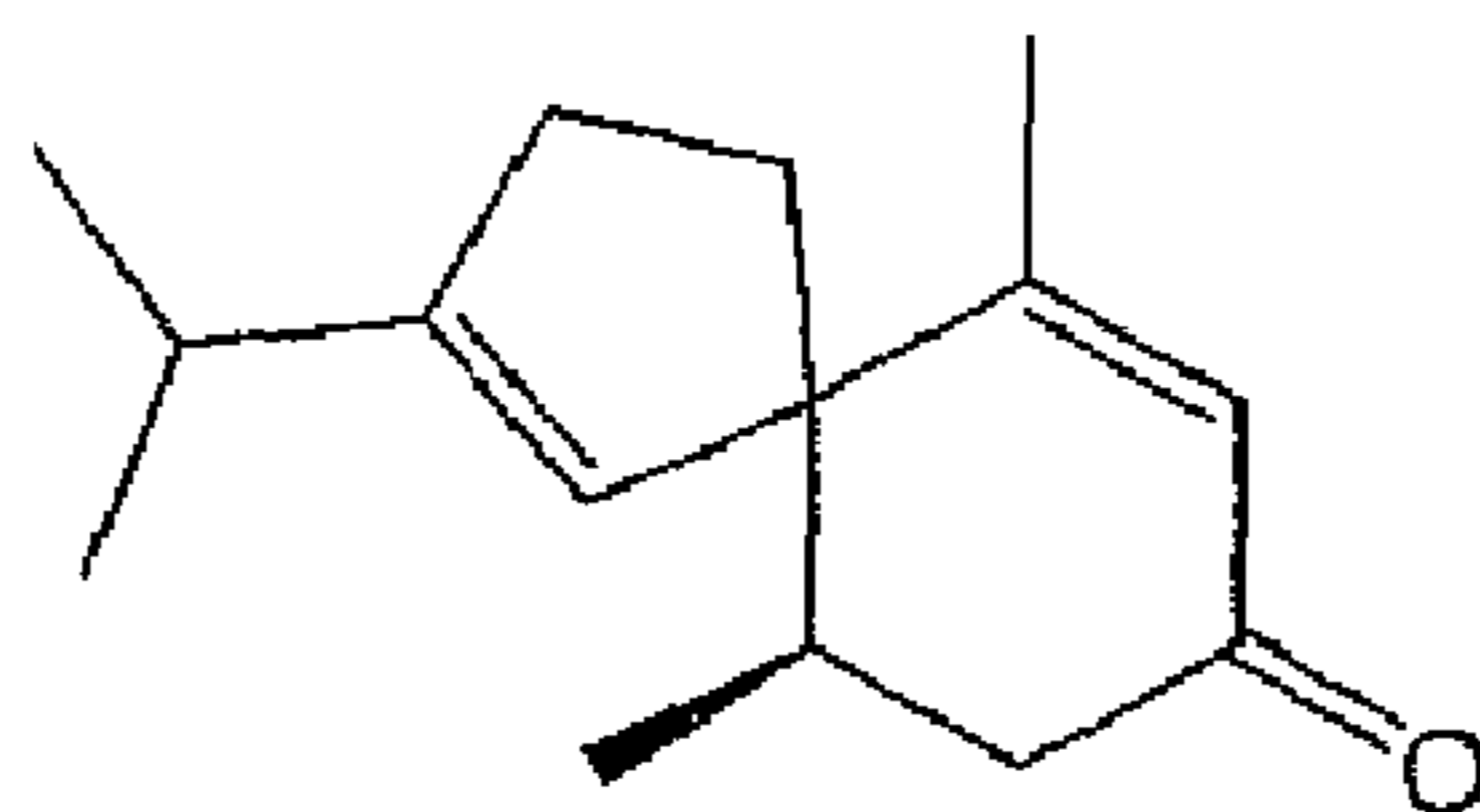
2-isopropyl-6,10-dimethyl-spiro[4.5]deca-1,6-dien-8-one (4)
