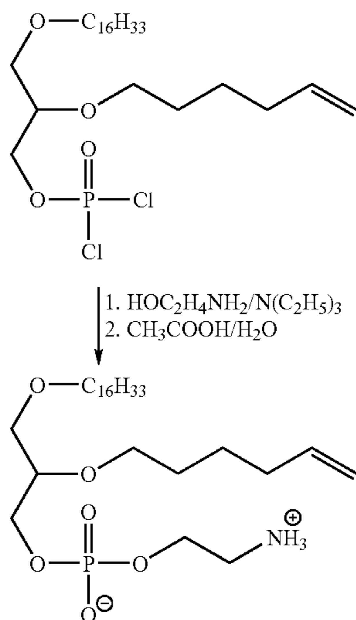
Scheme XIII
