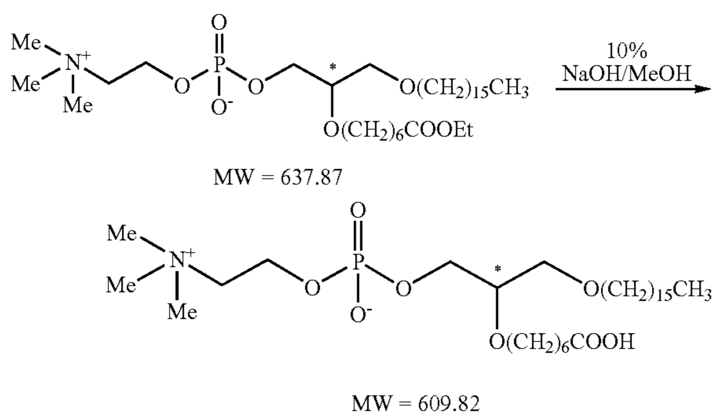
Scheme XX
