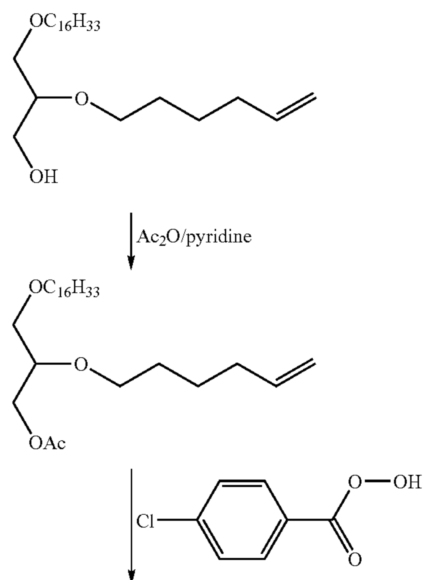
Scheme VII
