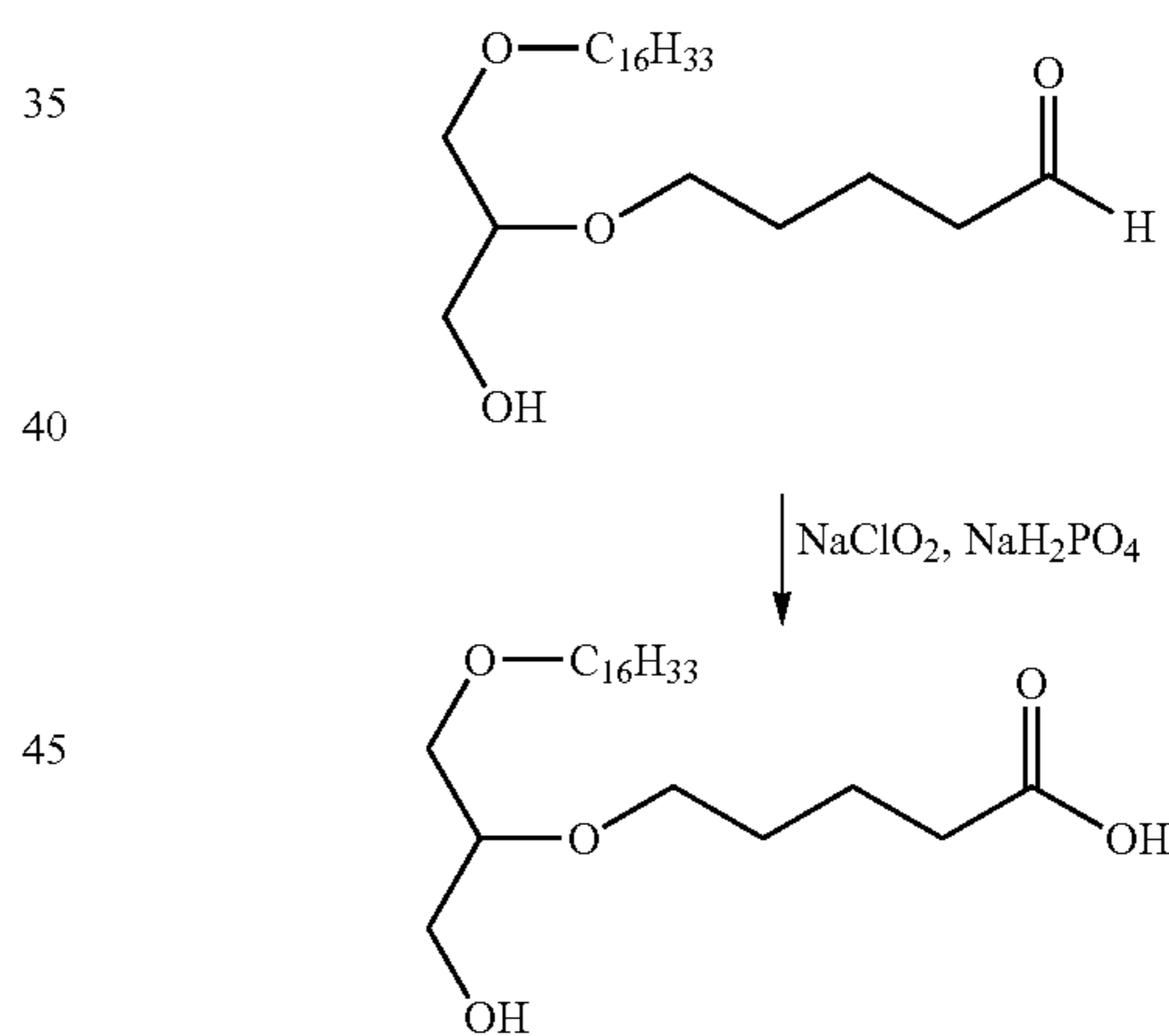
Scheme IV
