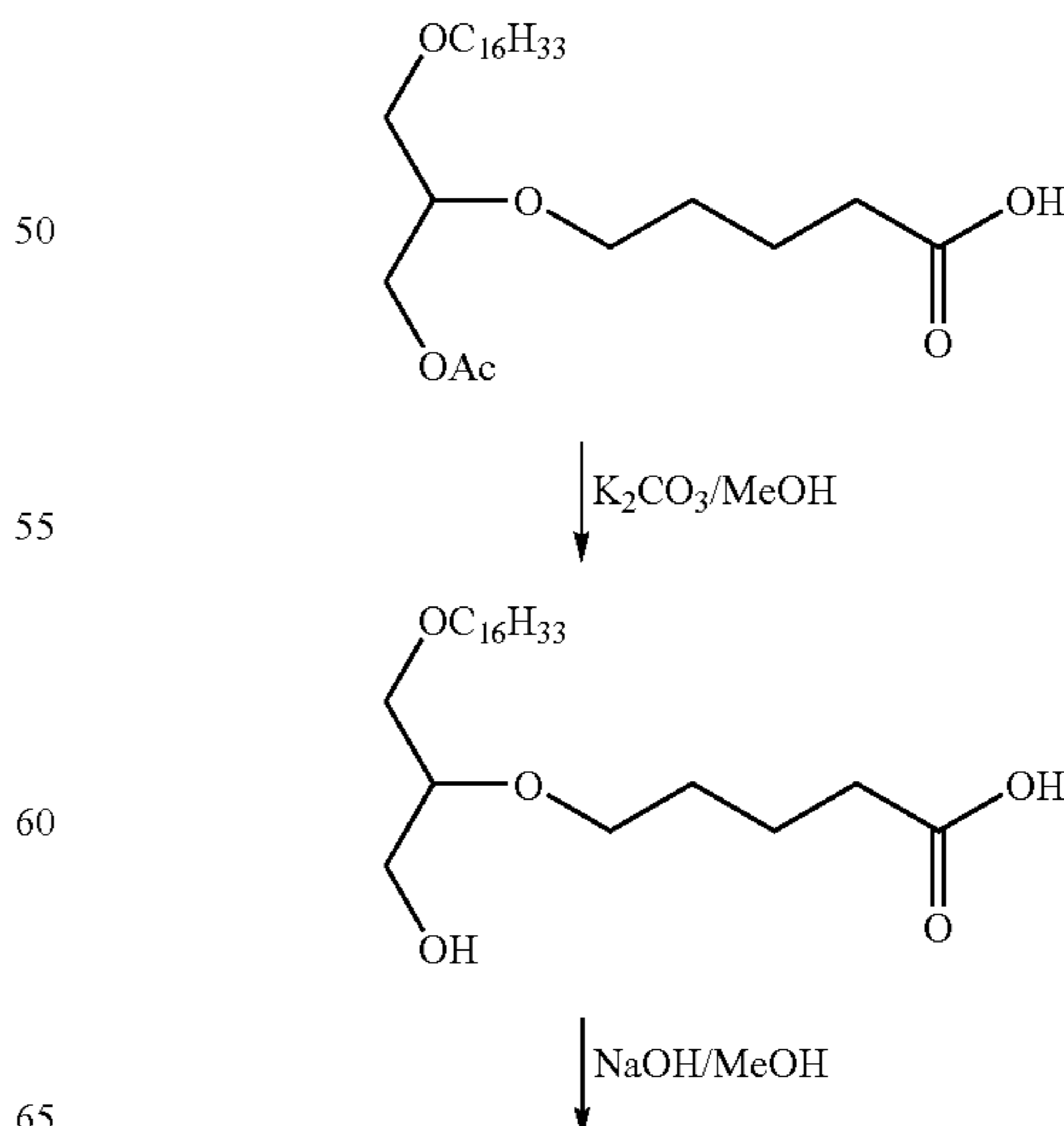
Scheme X
