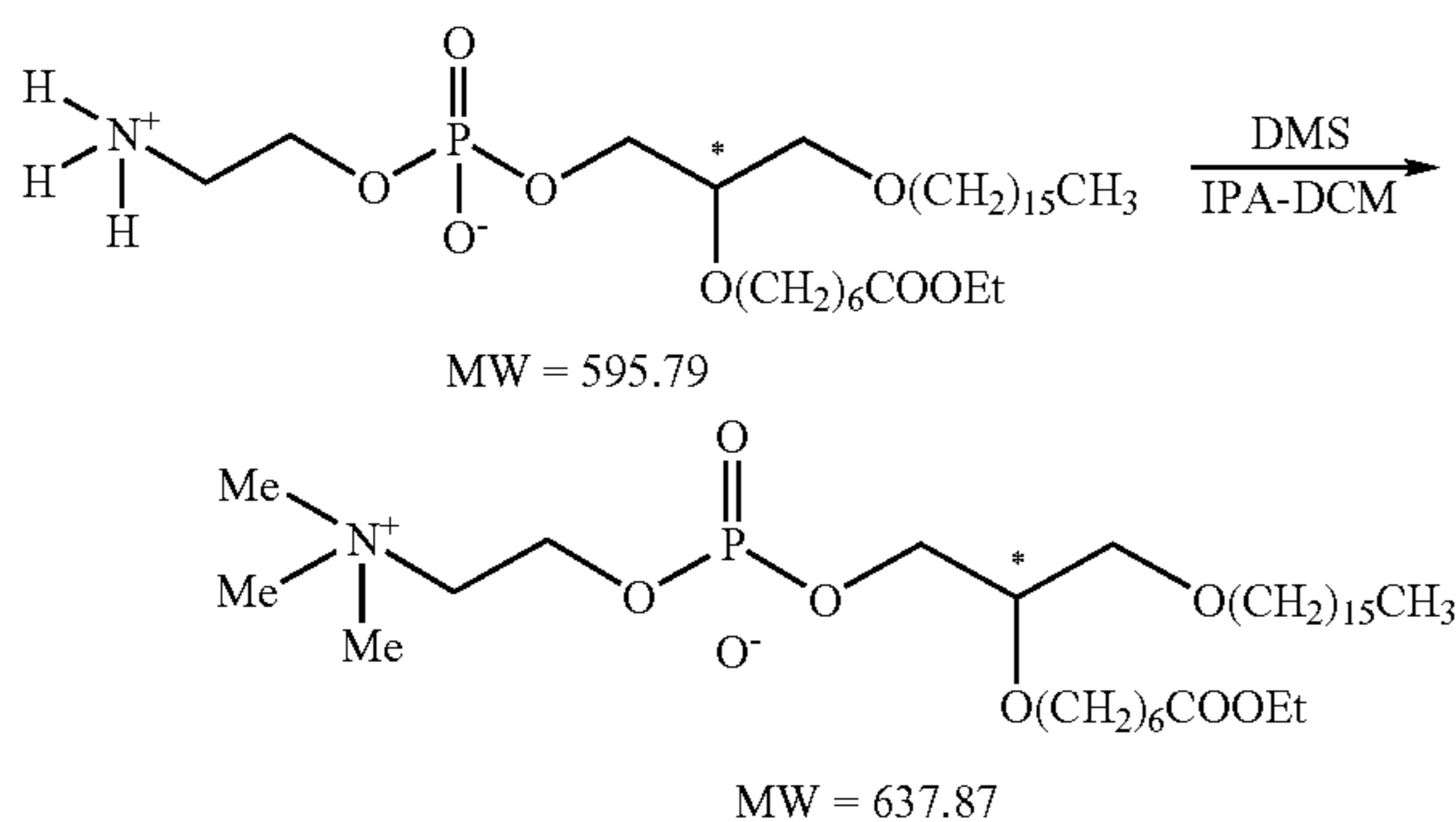
Scheme XIX
