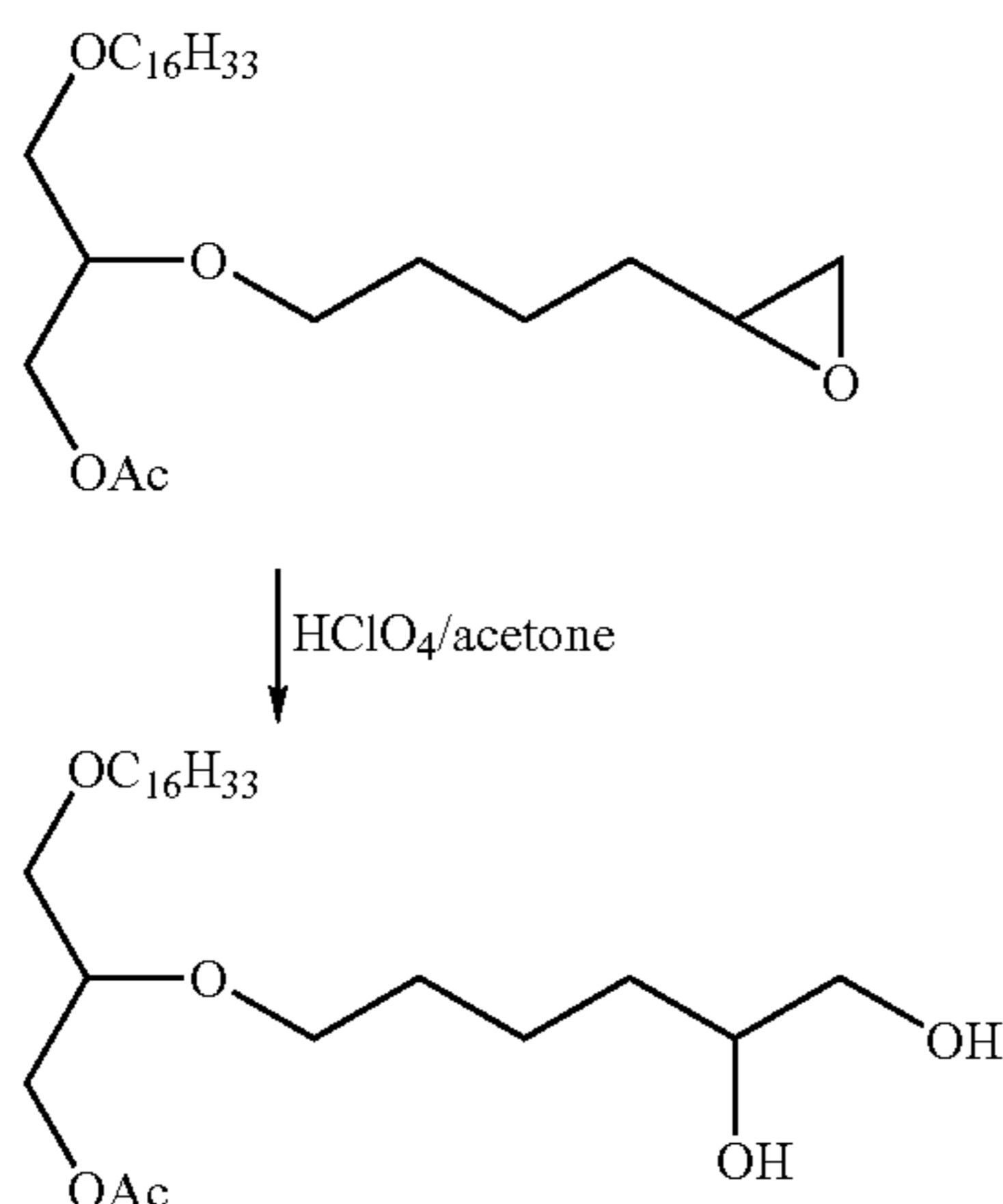
Scheme VIII
