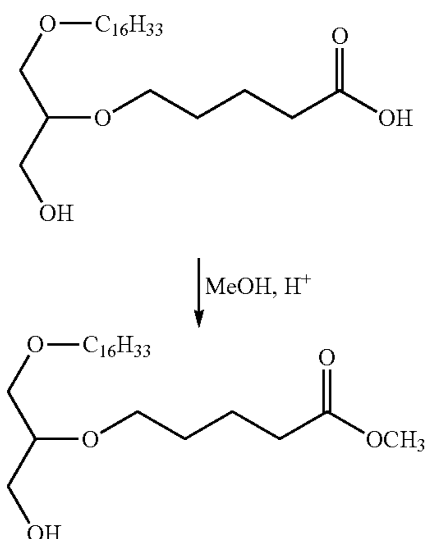
Scheme V
