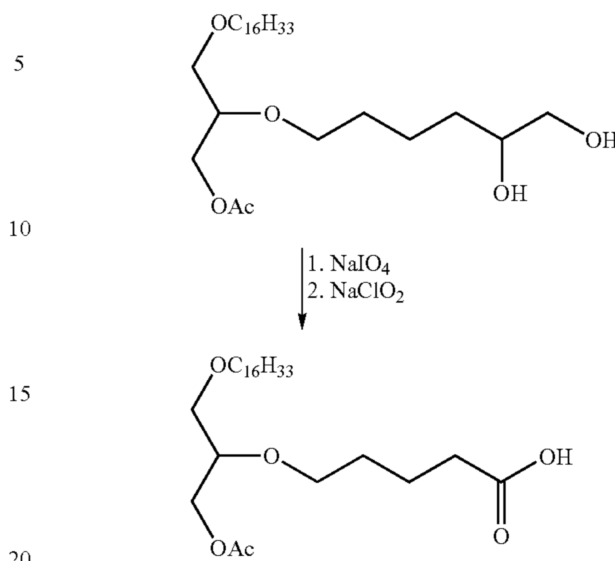
Scheme IX
