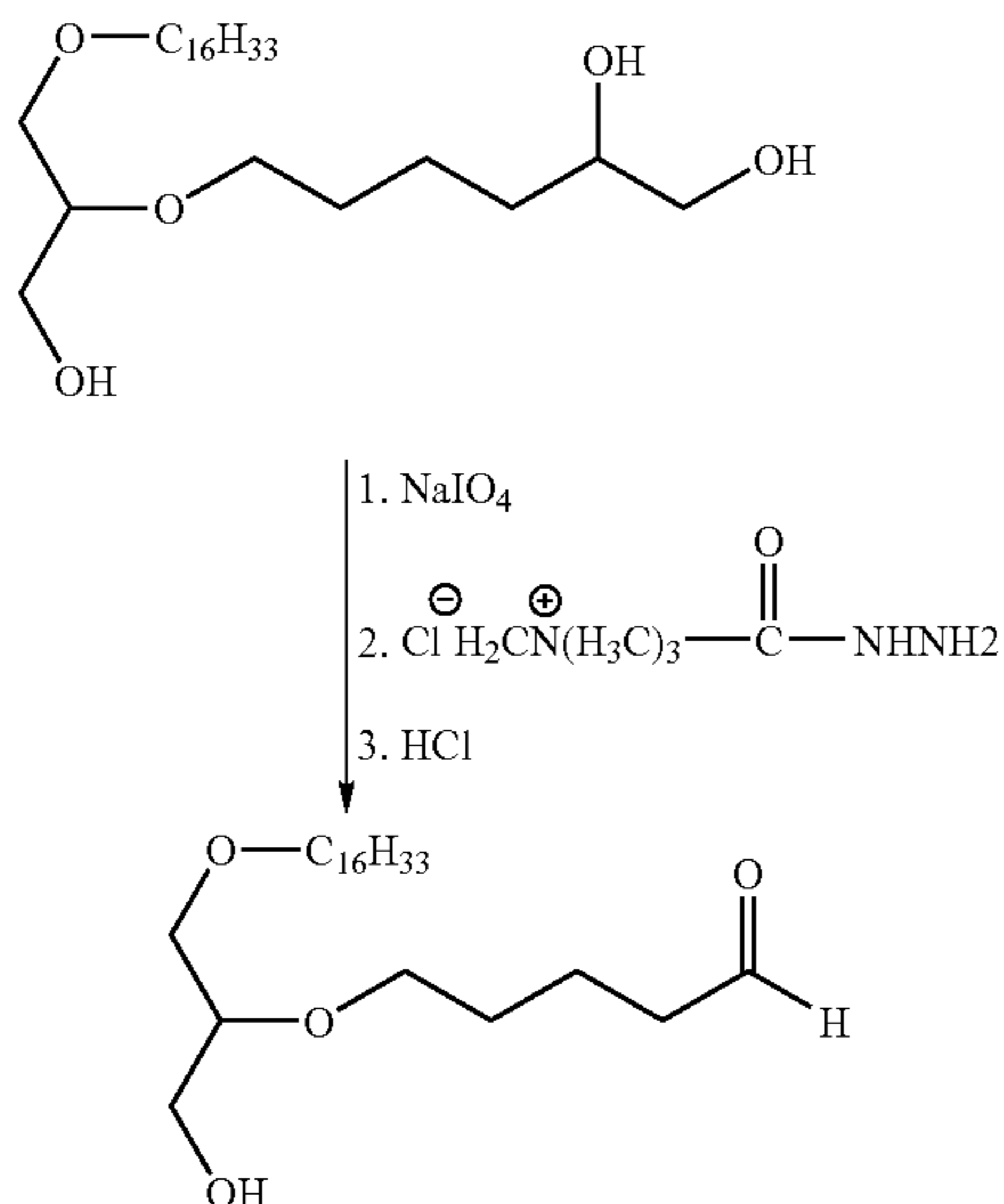
Scheme III
