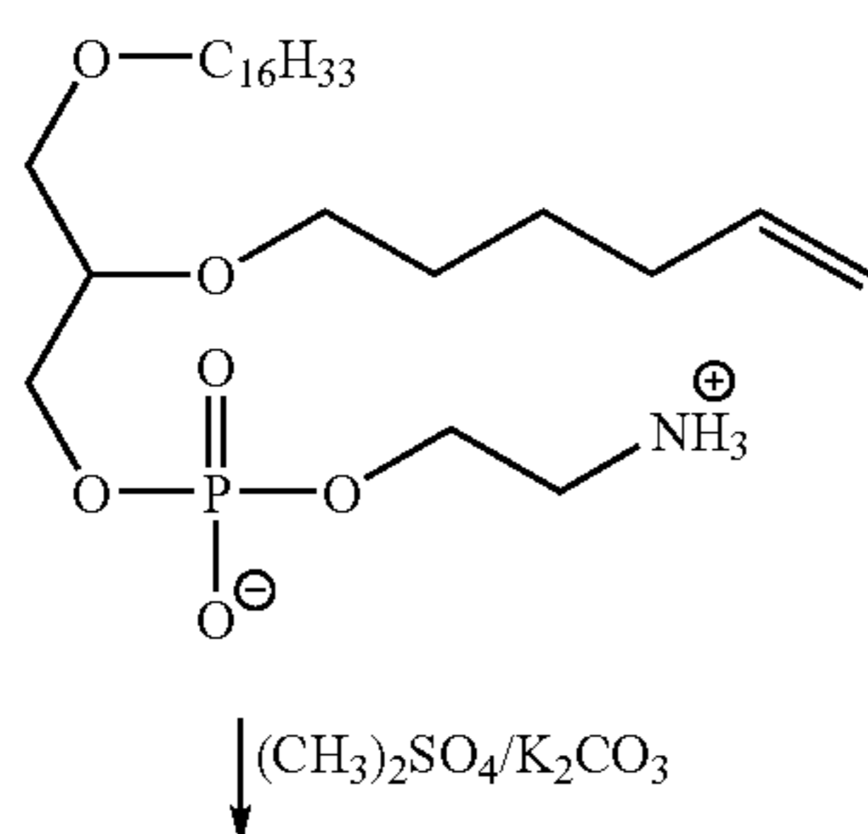
Scheme XIV
