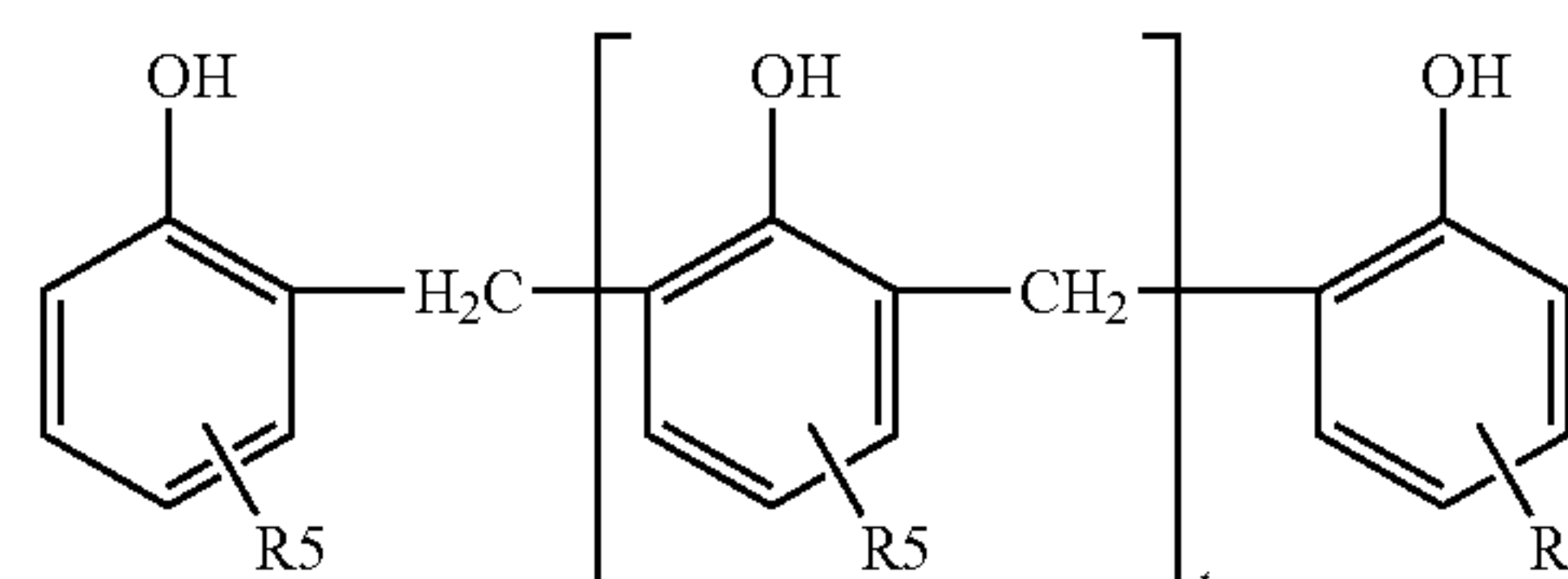
Formula (XXXII)
