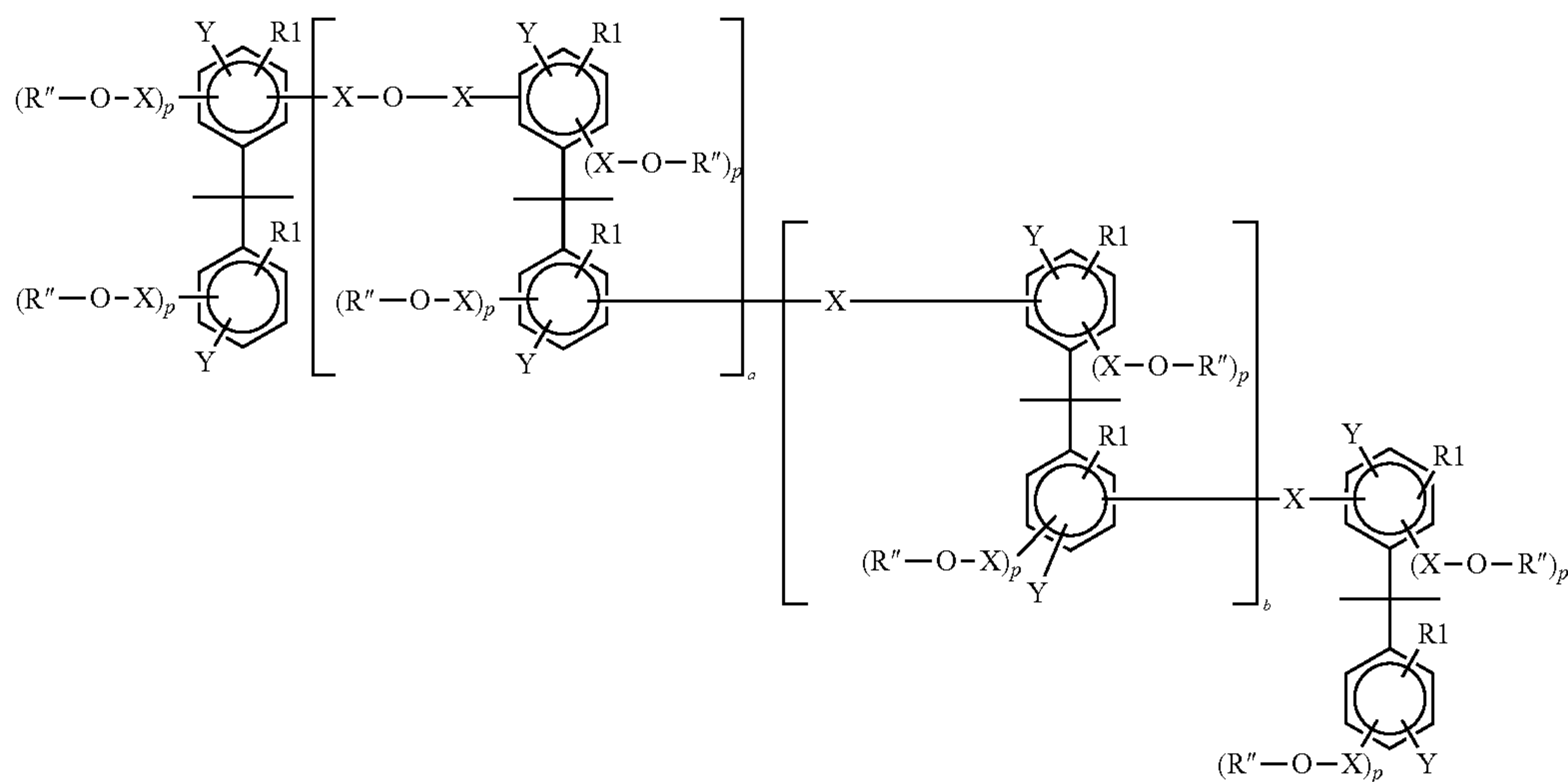
Formula (VI)
