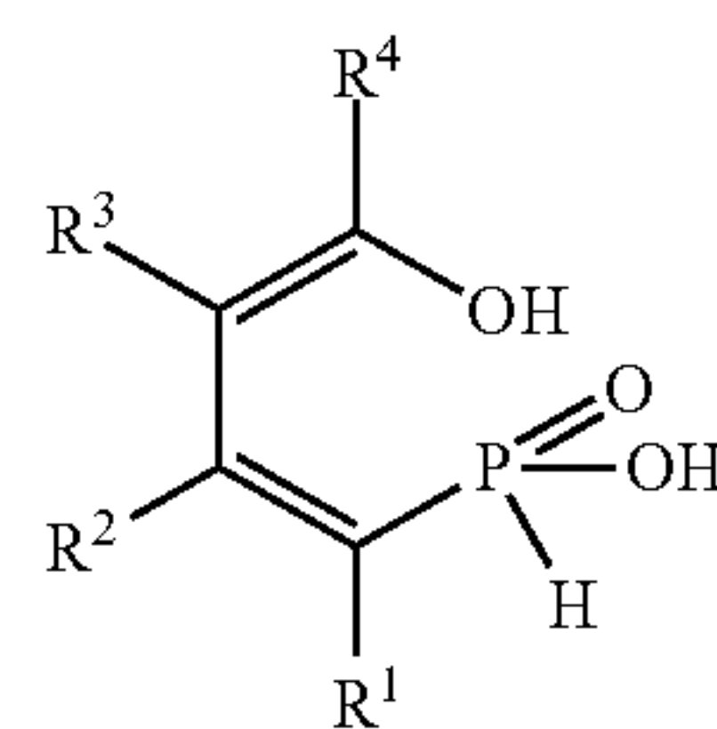
Formula (X) 5
