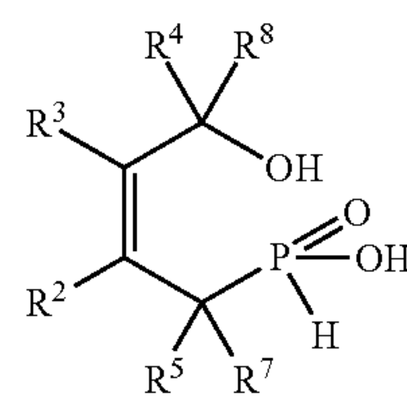
Formula (XIII) 20
