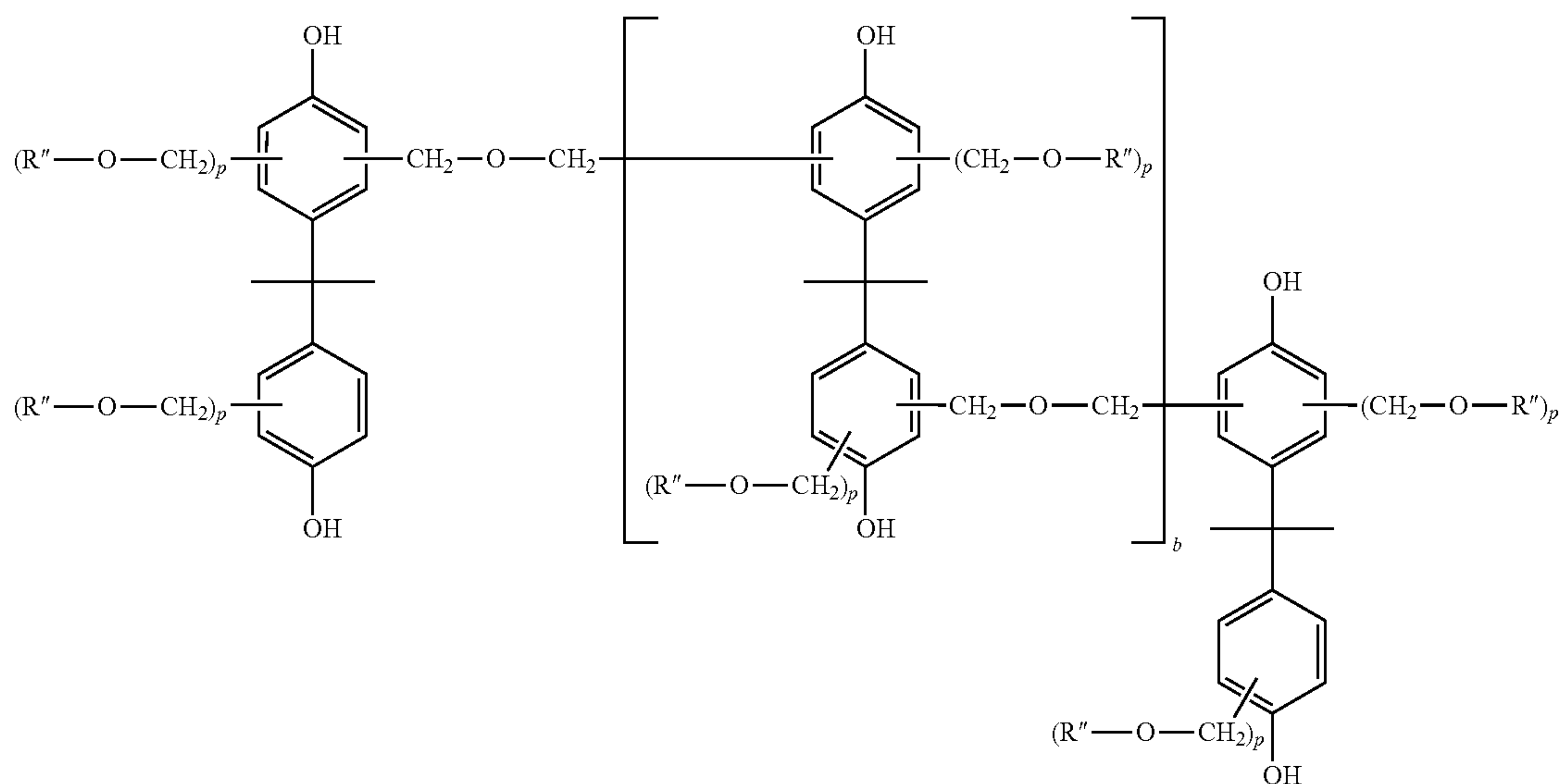
Formula (IXa)
