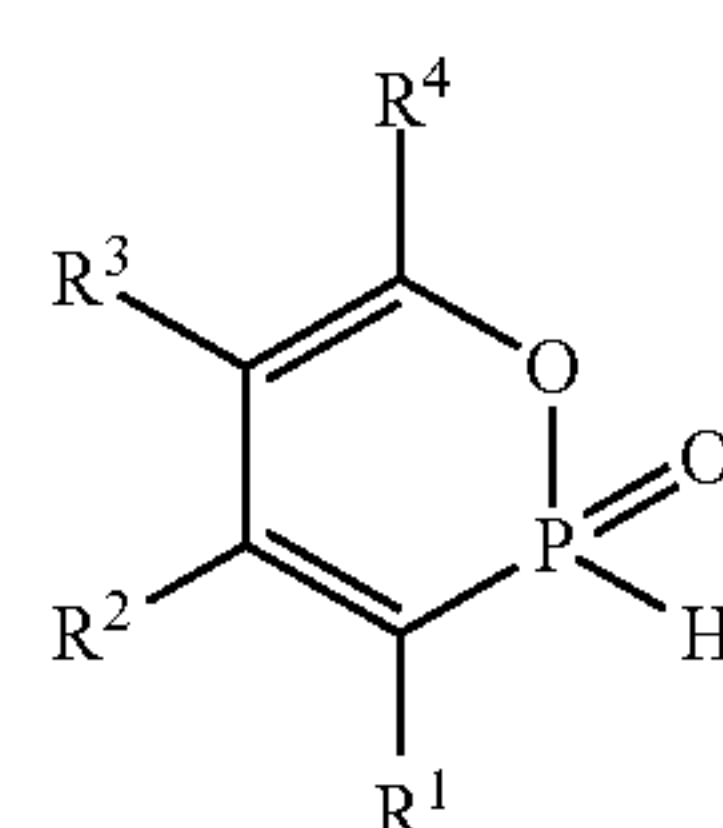
Formula (XII) 15
