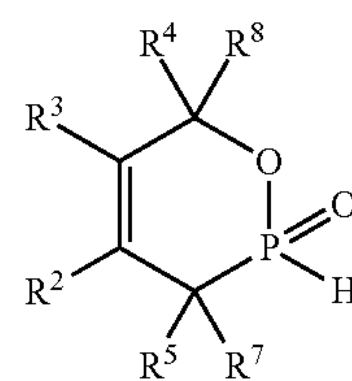
Formula (XV) 30
