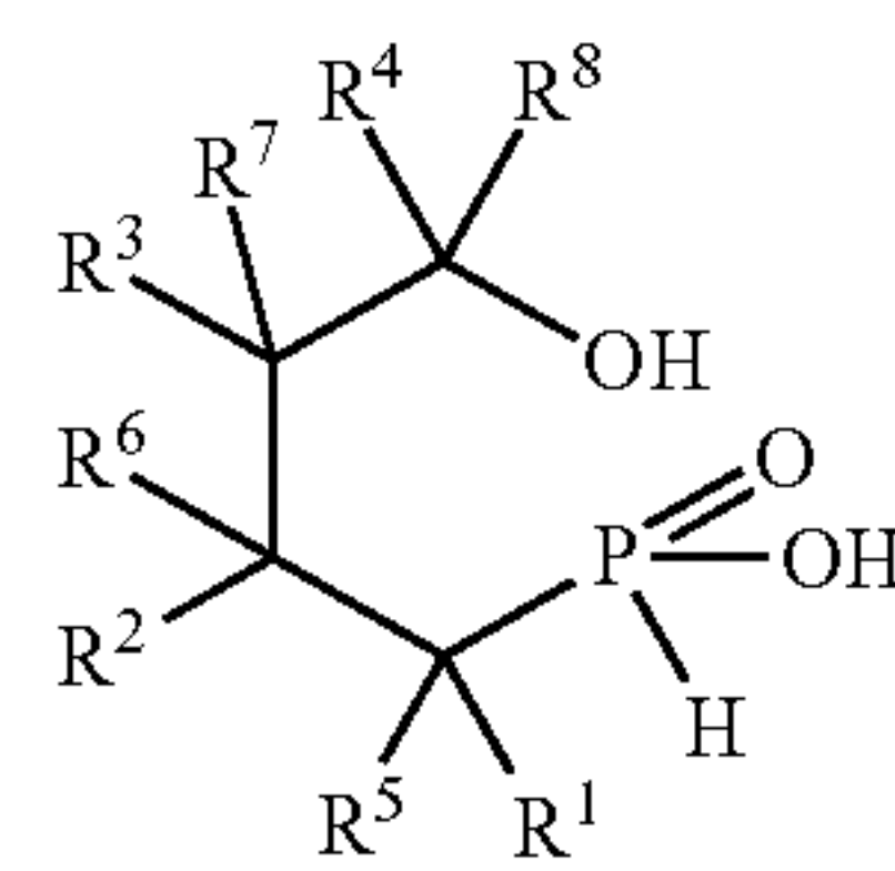
Formula (XIX) 50
