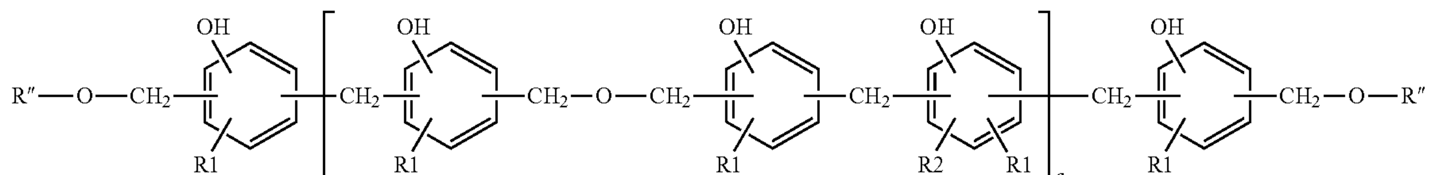
Formula (VIII)
