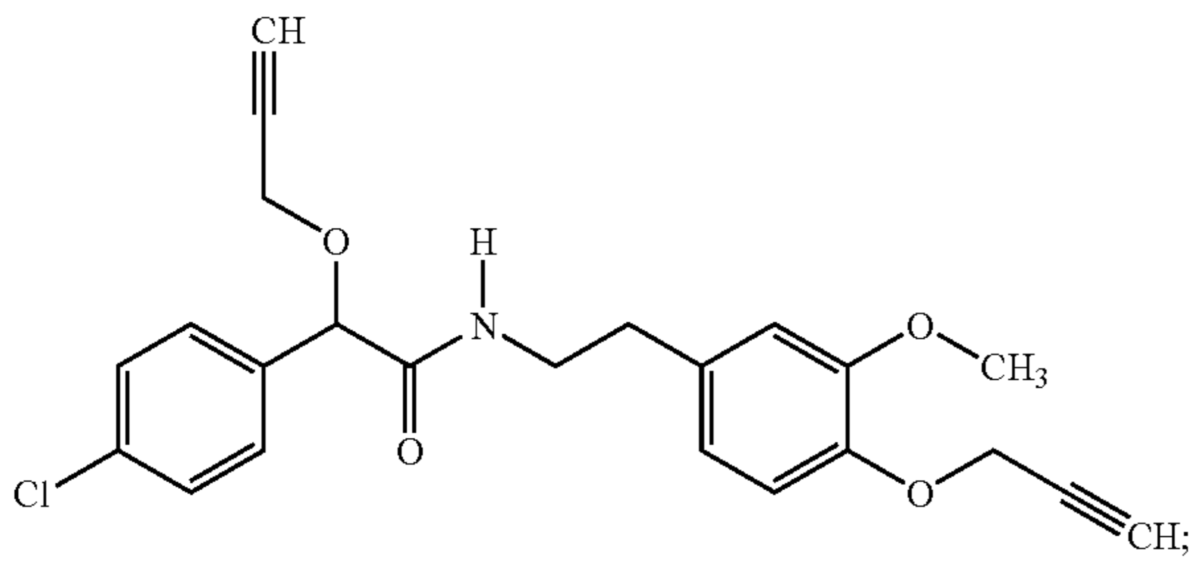
a compound of formula B-1
