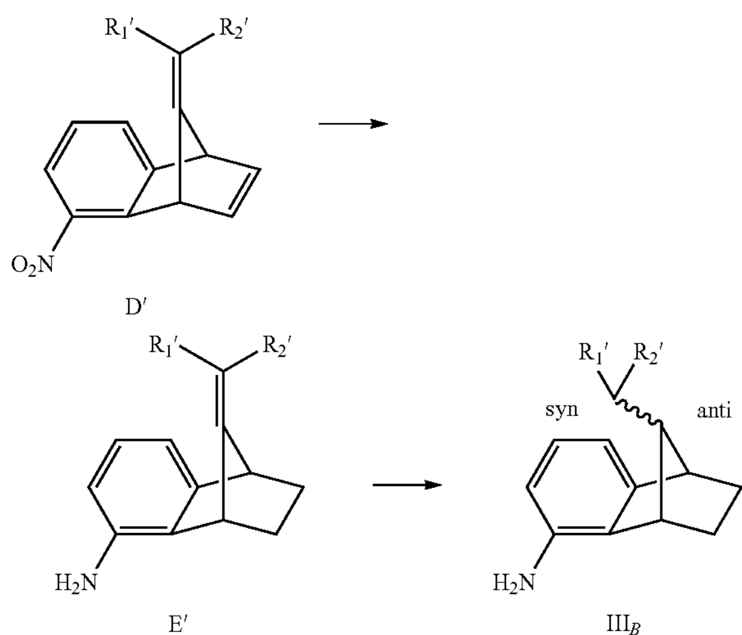
Scheme 2: Two-step hydrogenation
