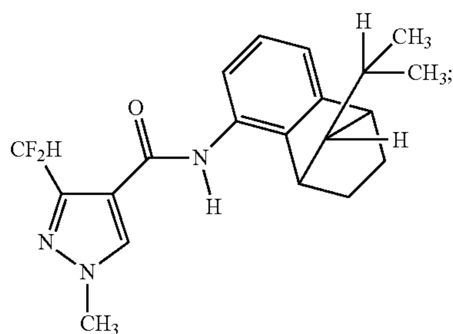
a racemic compound of formula Ib (anti)
