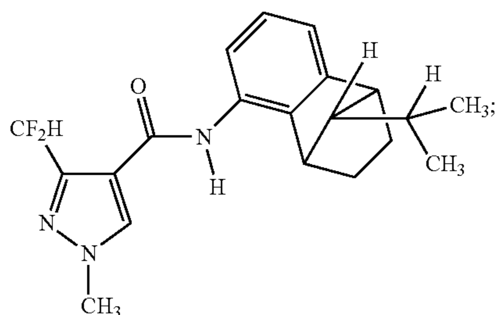
a racemic compound of formula Ib (anti)
