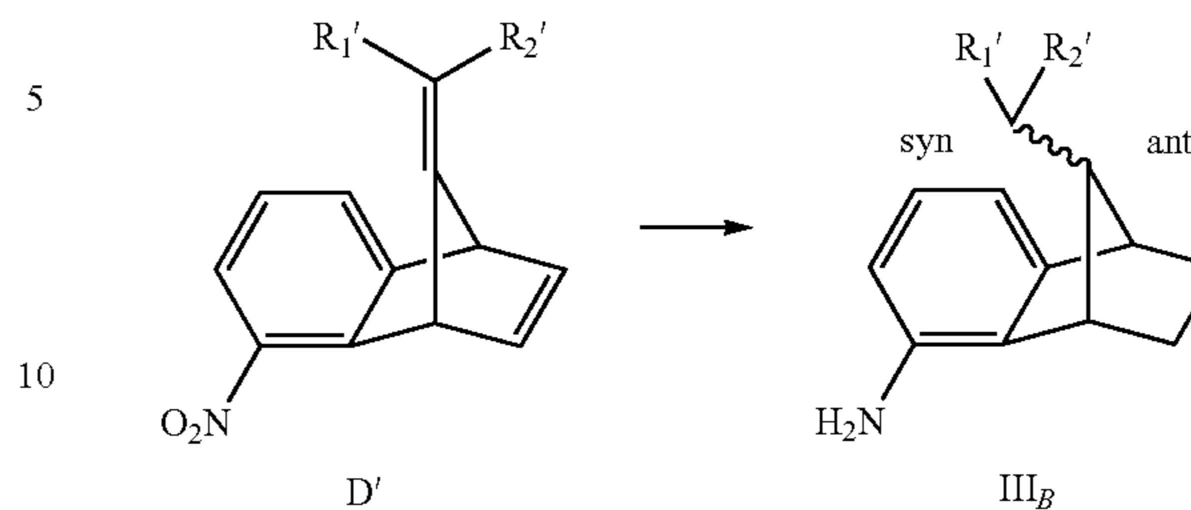
Scheme 3: One-pot hydrogenation
