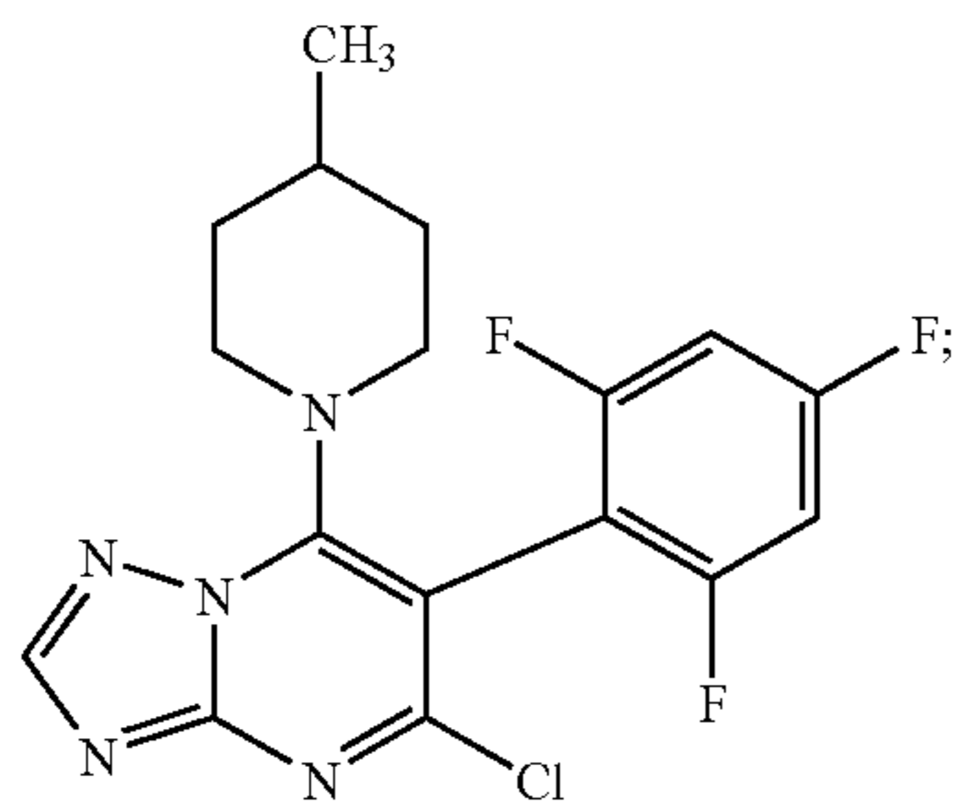
a compound of formula B-1
