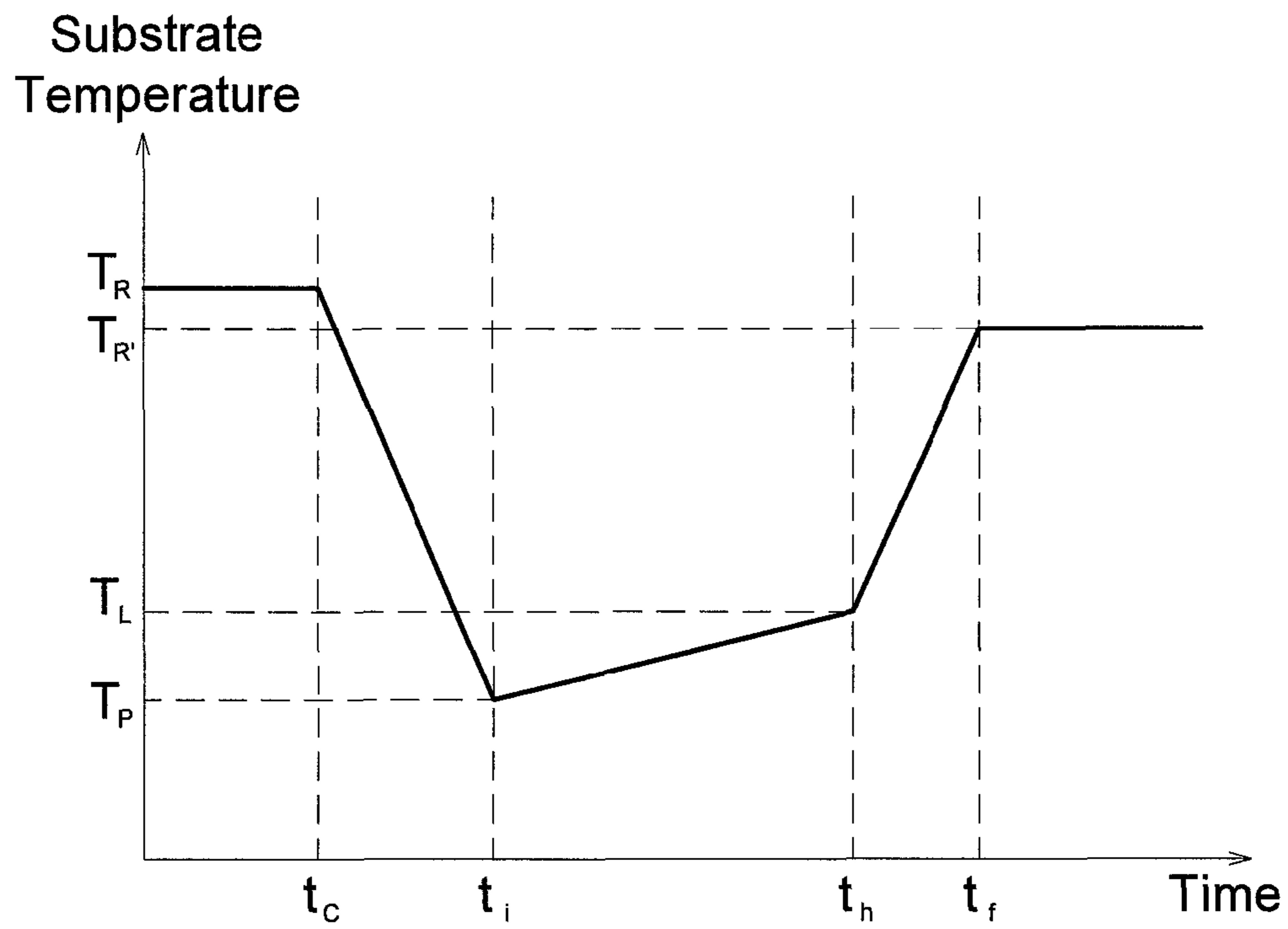
Fig. 1a(Prior Art)
