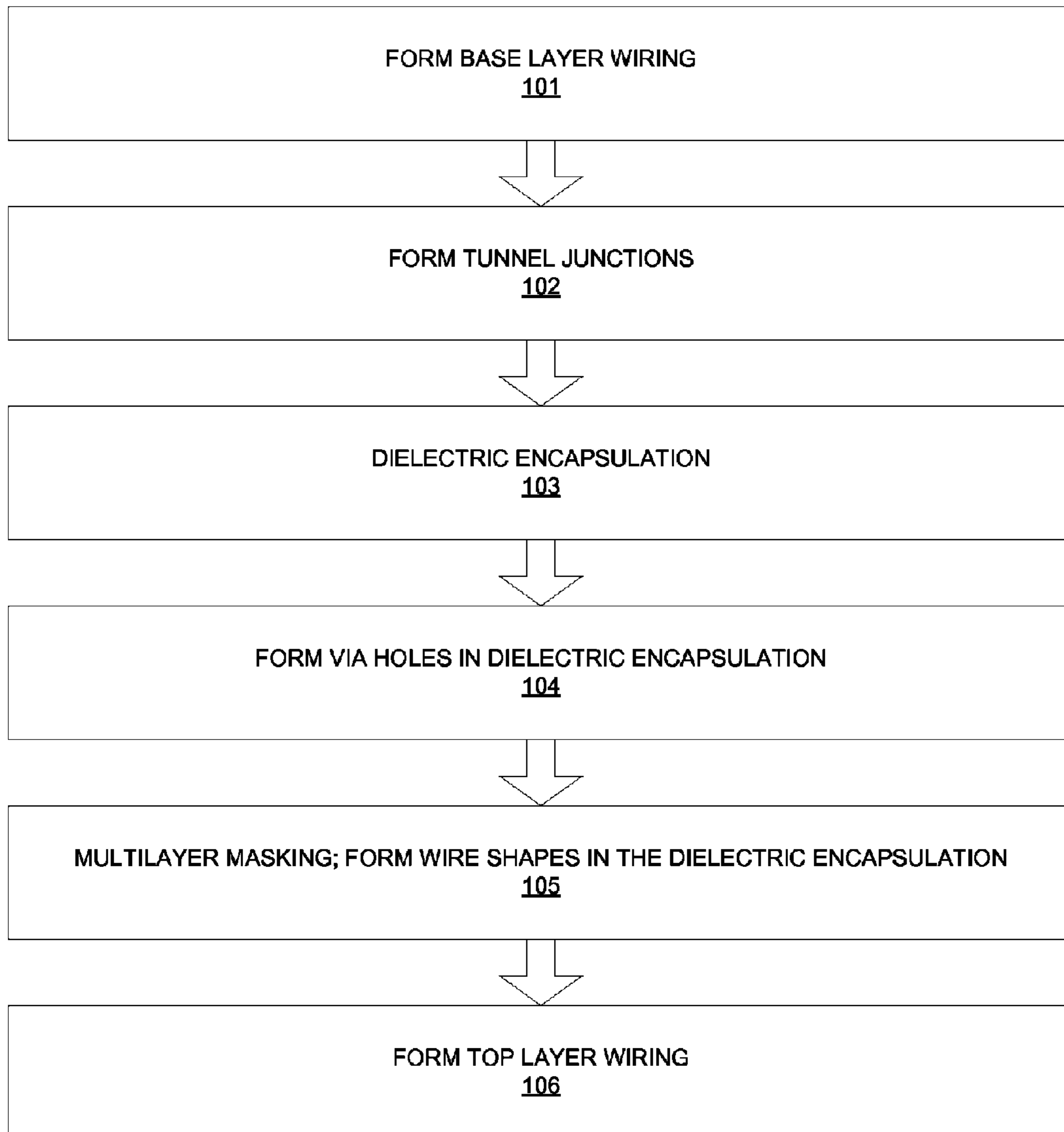
FIG. 1 PRIOR ART
