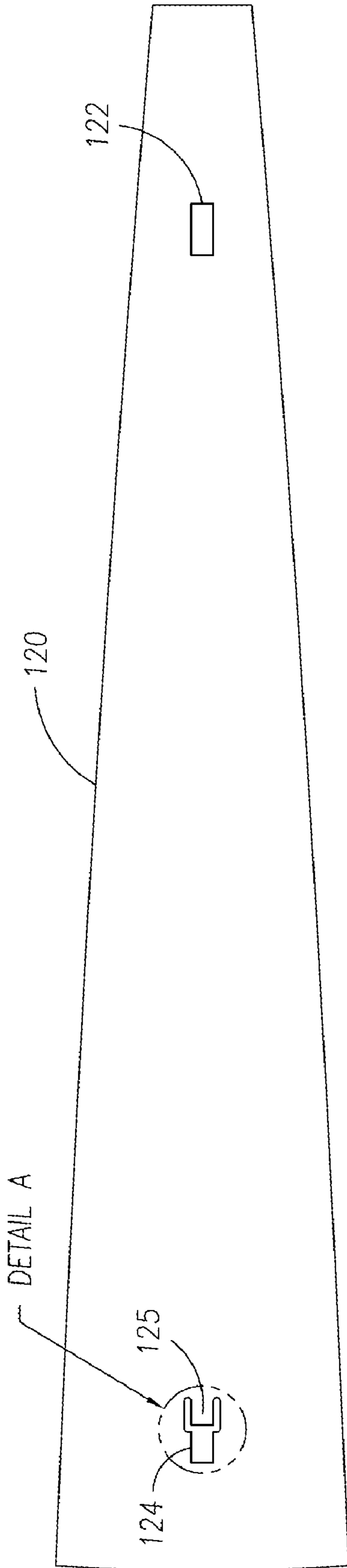
FLAT PATTERN
