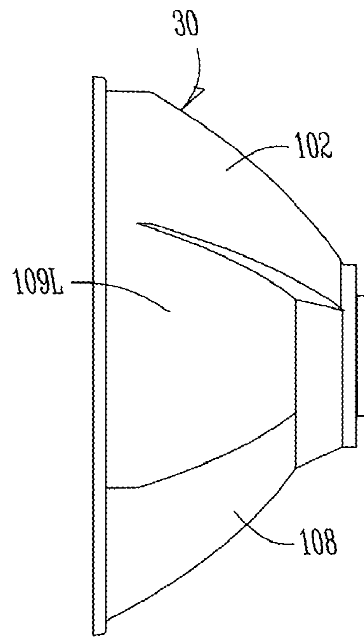
RIGHT SIDE VIEW Fig. 8C
