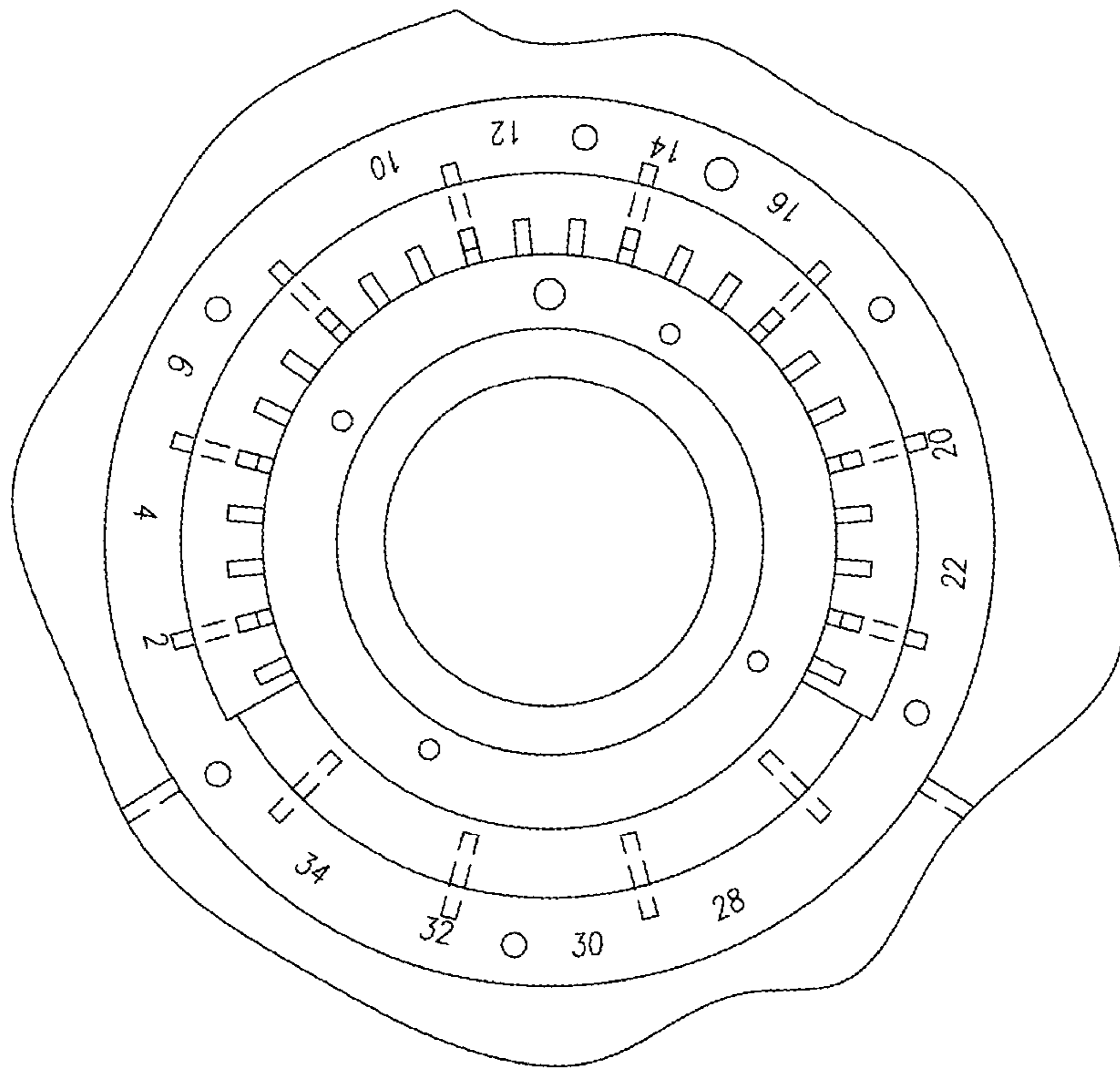
SECTION J-J
