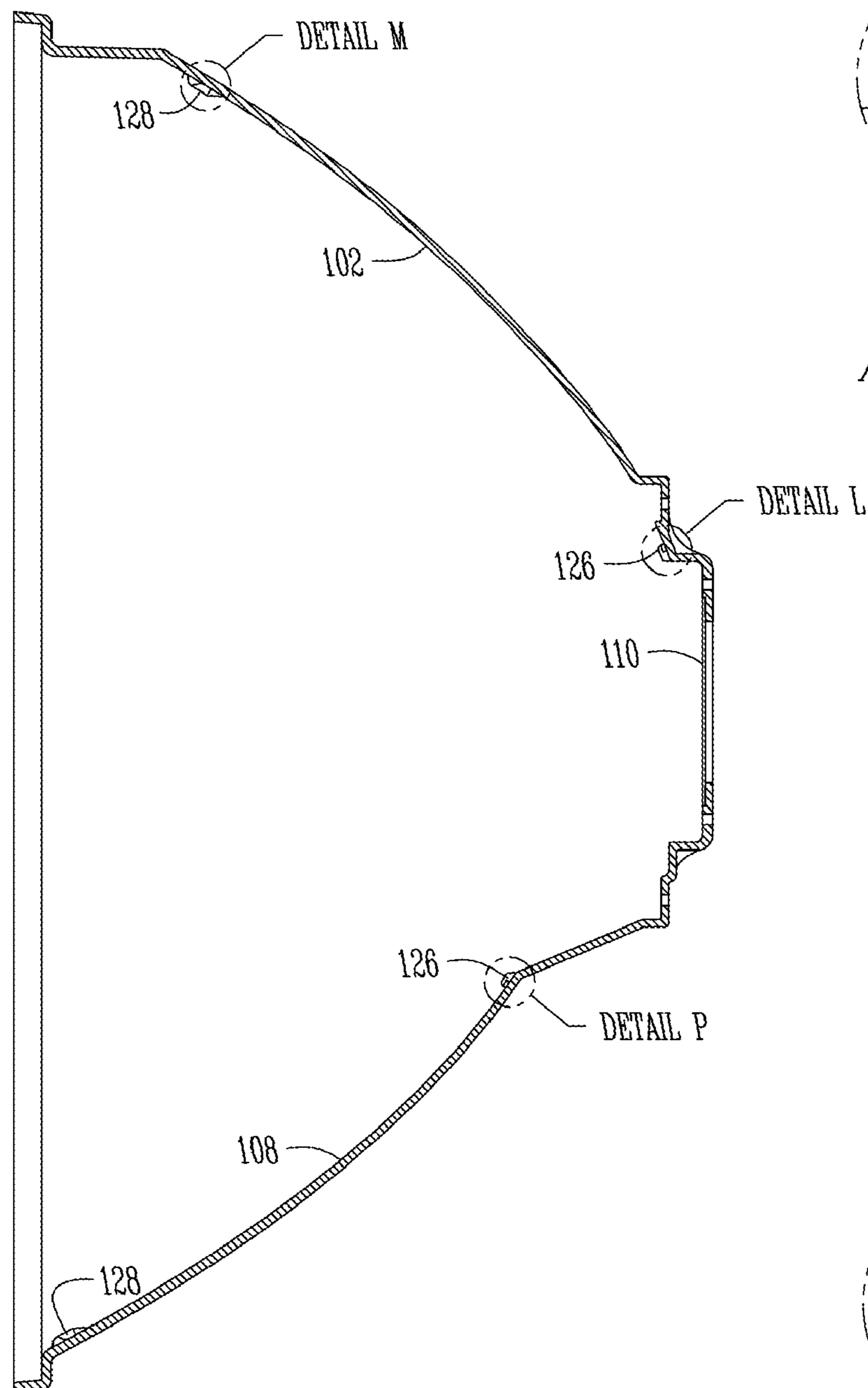
SECTION L-L ROTATED 90° CCW Fig. 6Q
