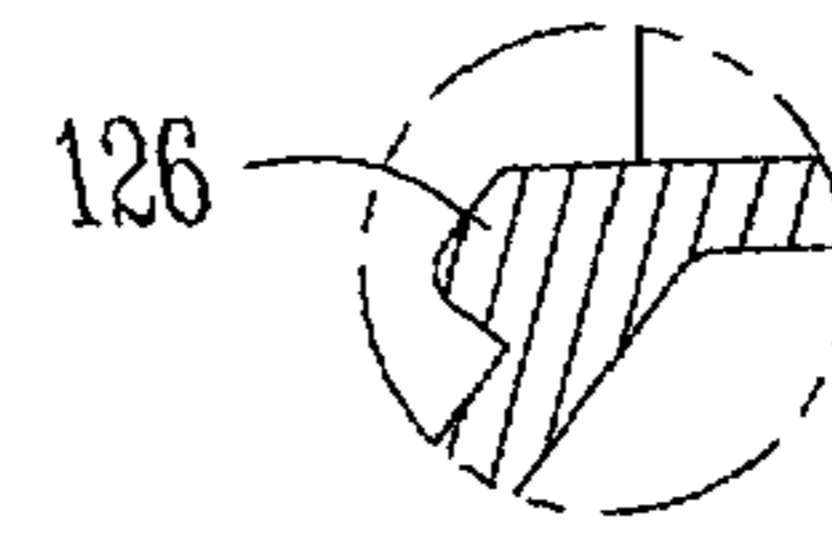
DETAIL G AS CAST Fig. 6L
