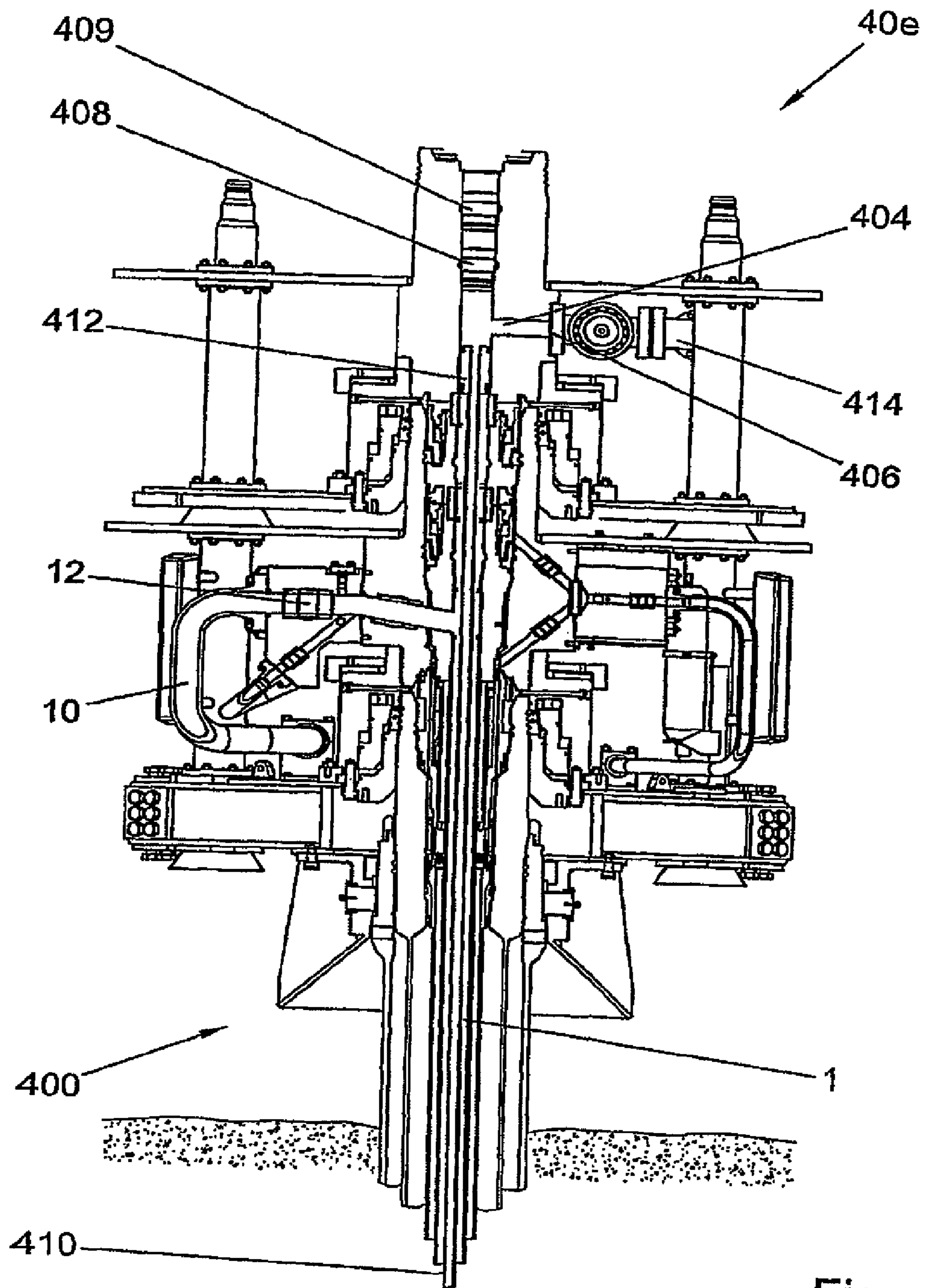
TYPICAL SECTION
