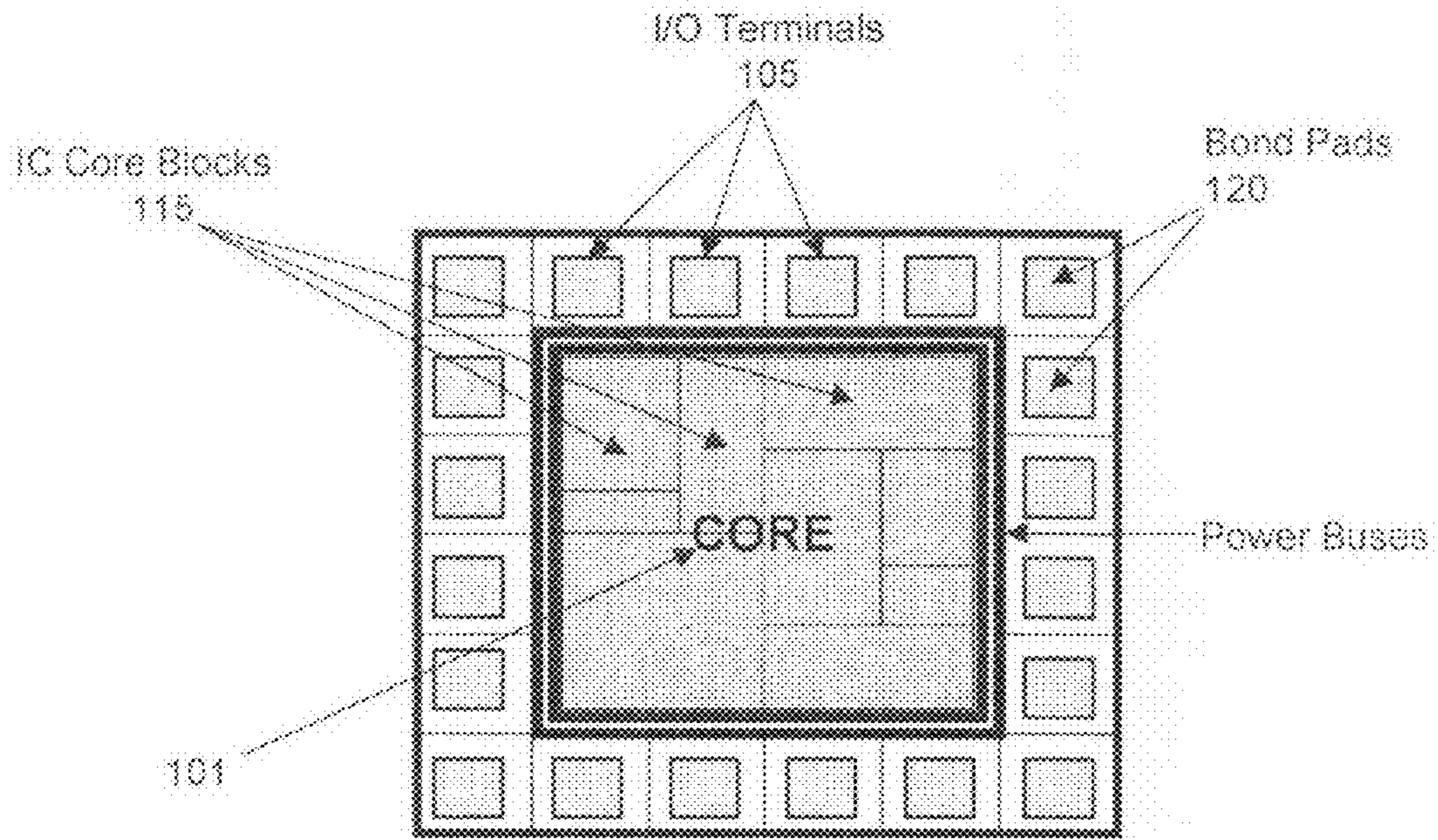
FIG. 1 (PRIOR ART)
