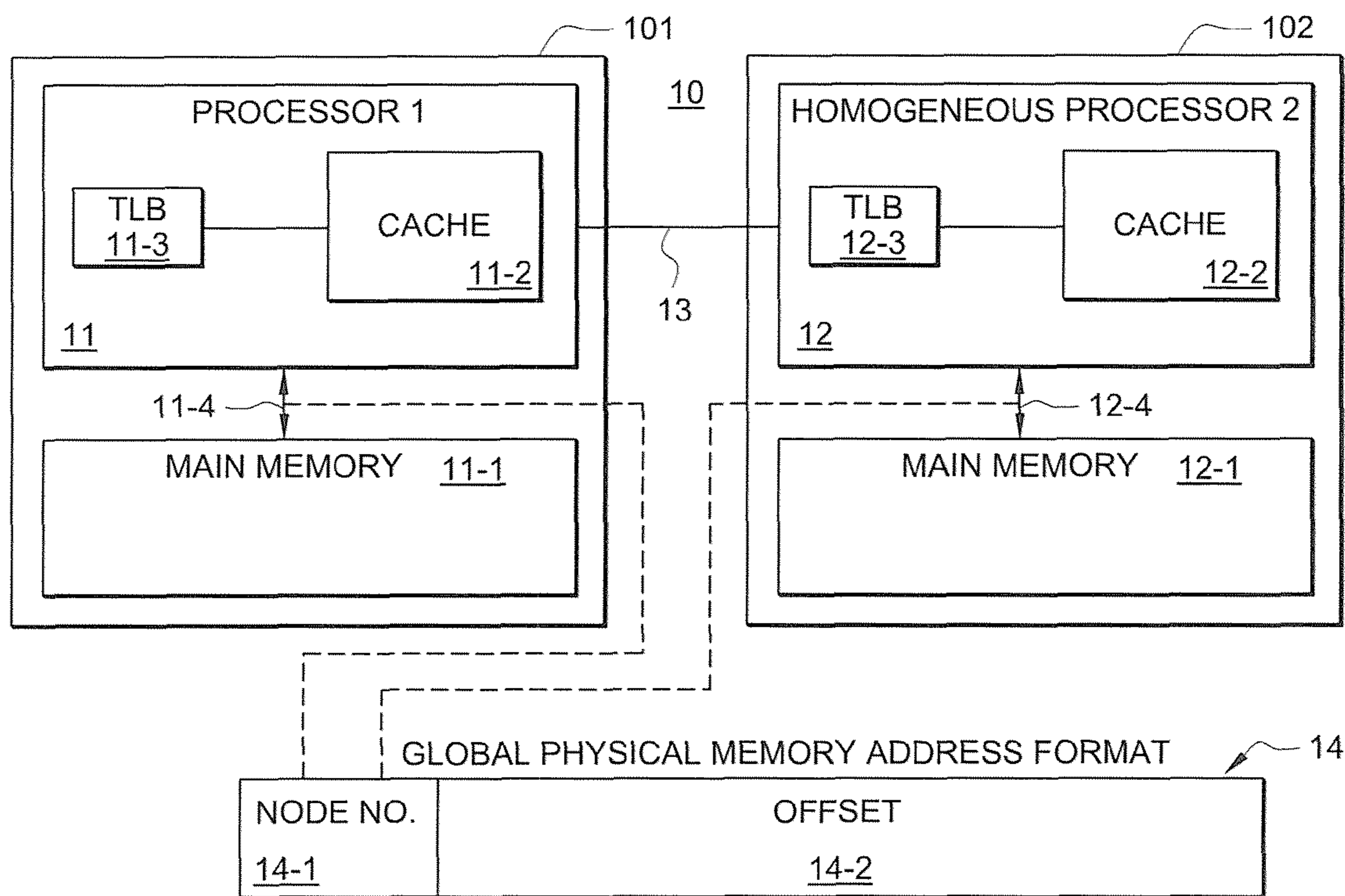
FIG. 1 (Prior Art)
