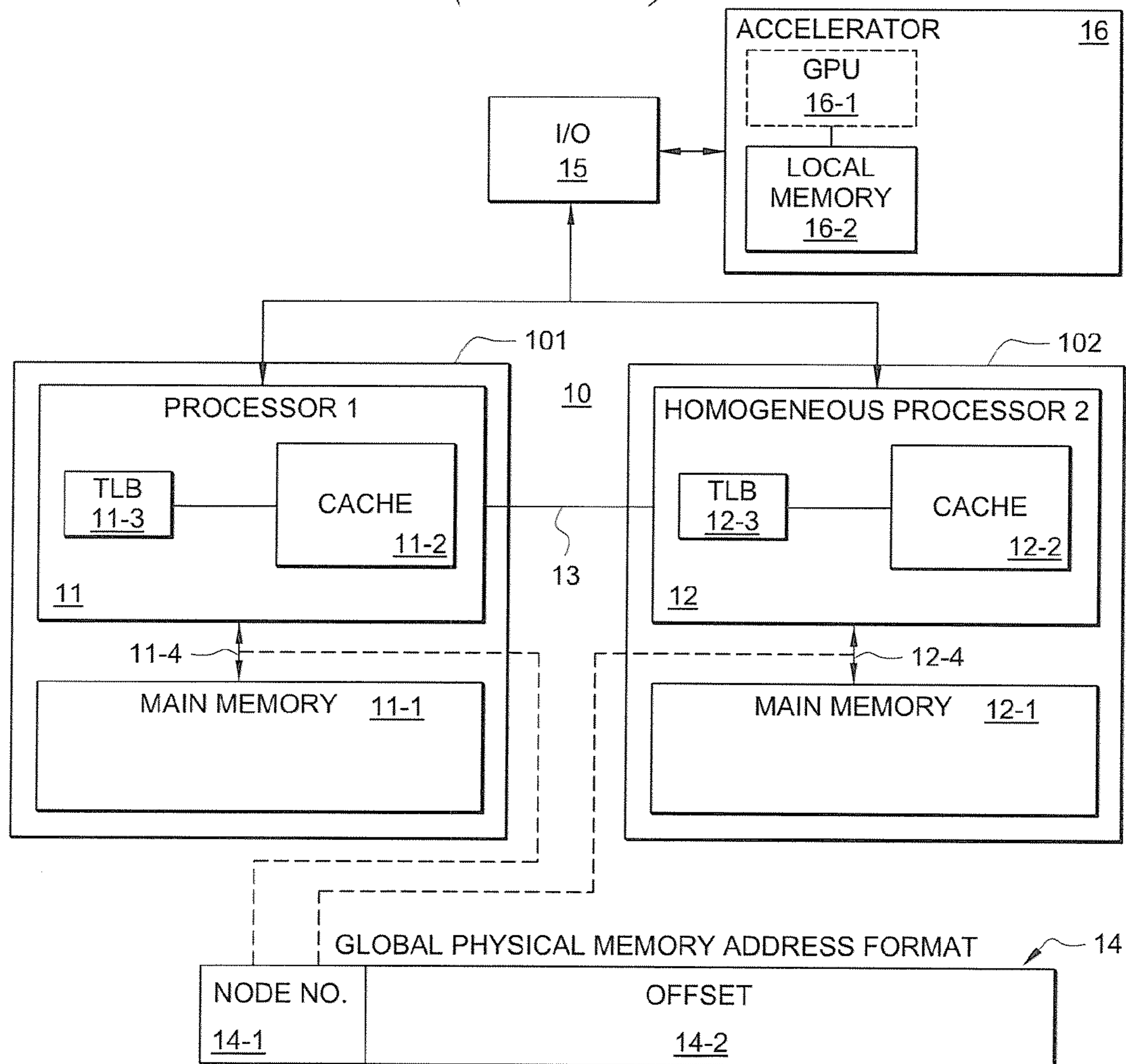
FIG. 2 (Prior Art)
