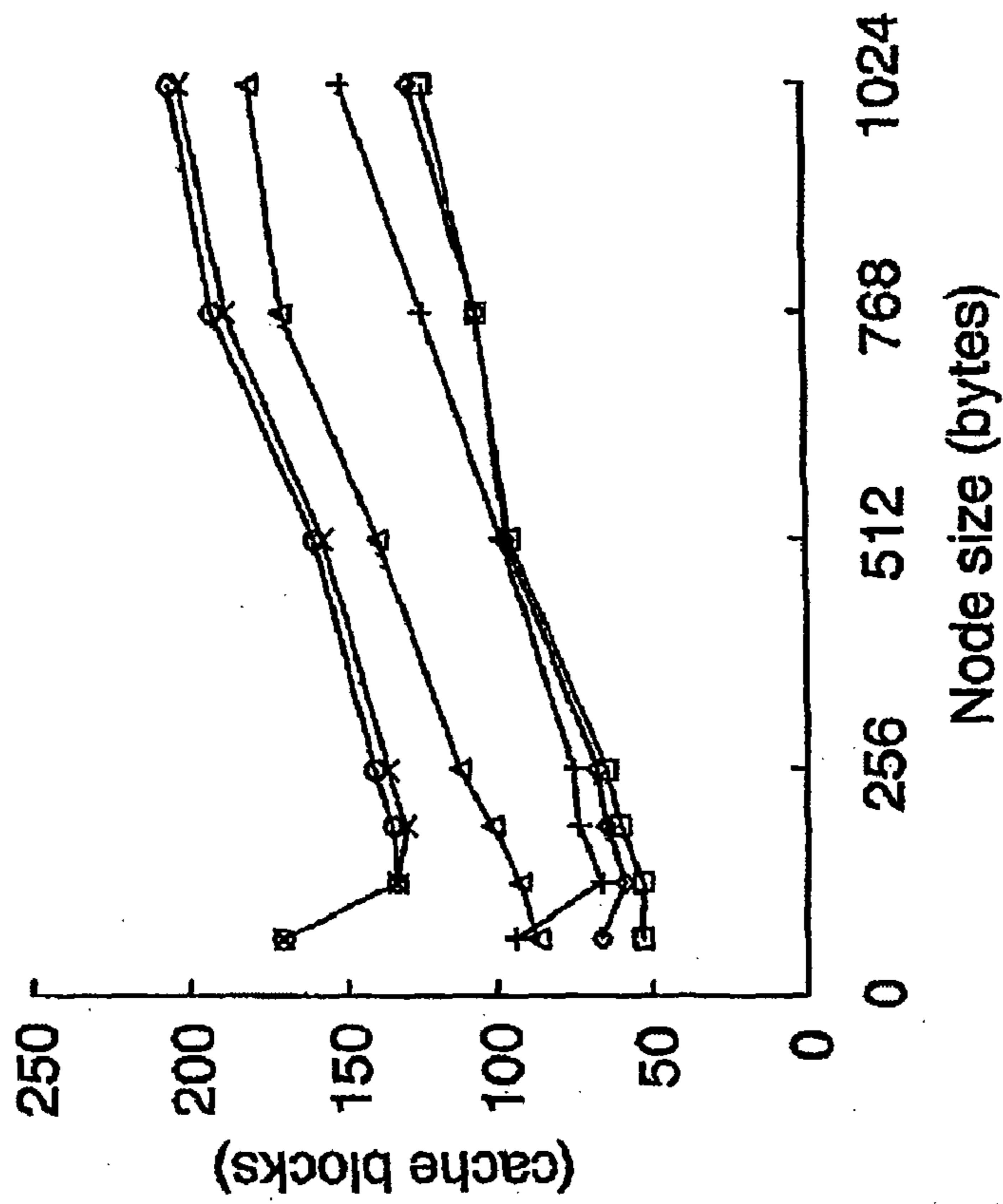
(a) Selectivity = 0.01%
