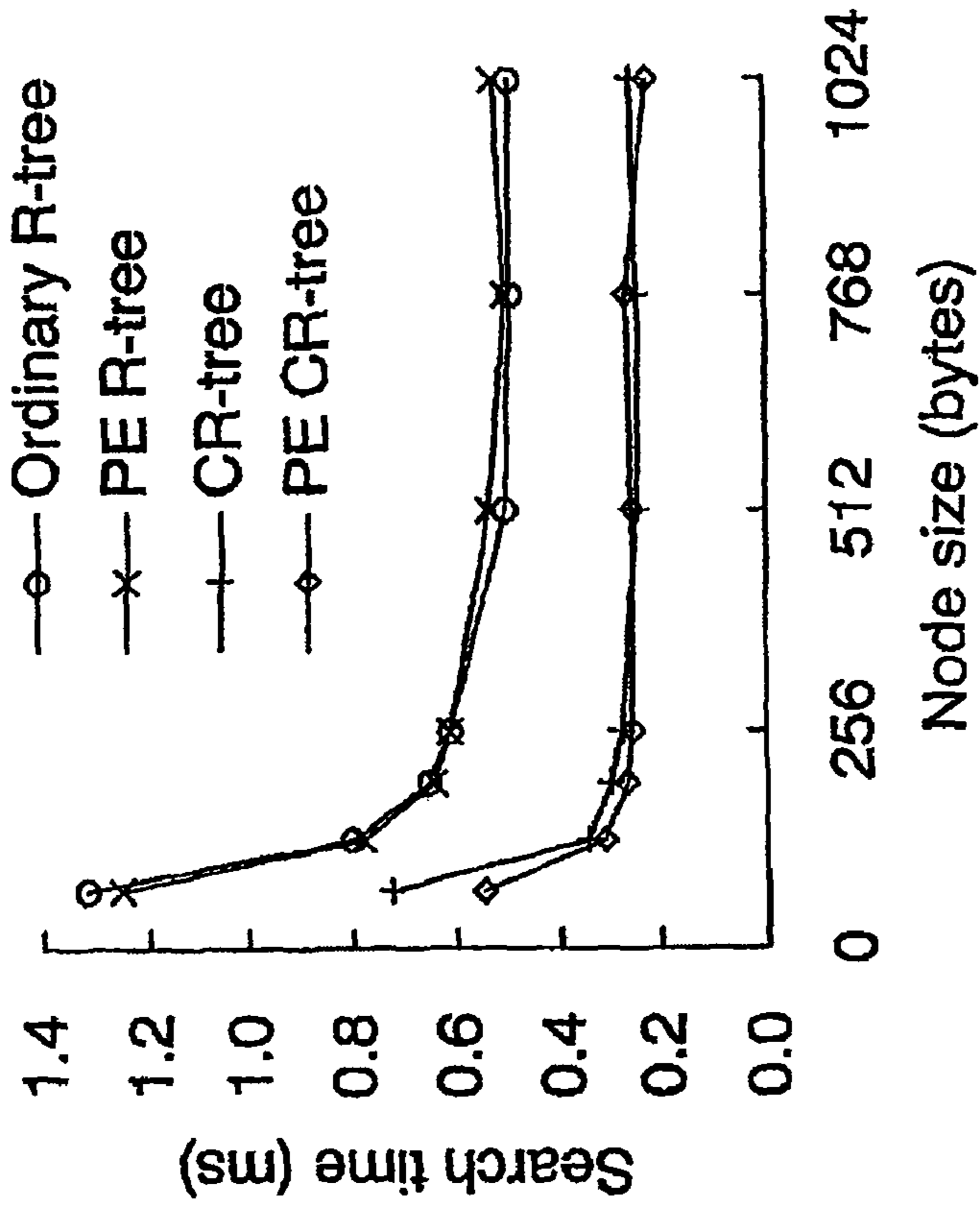
(b) Selectivity = 0.25%
