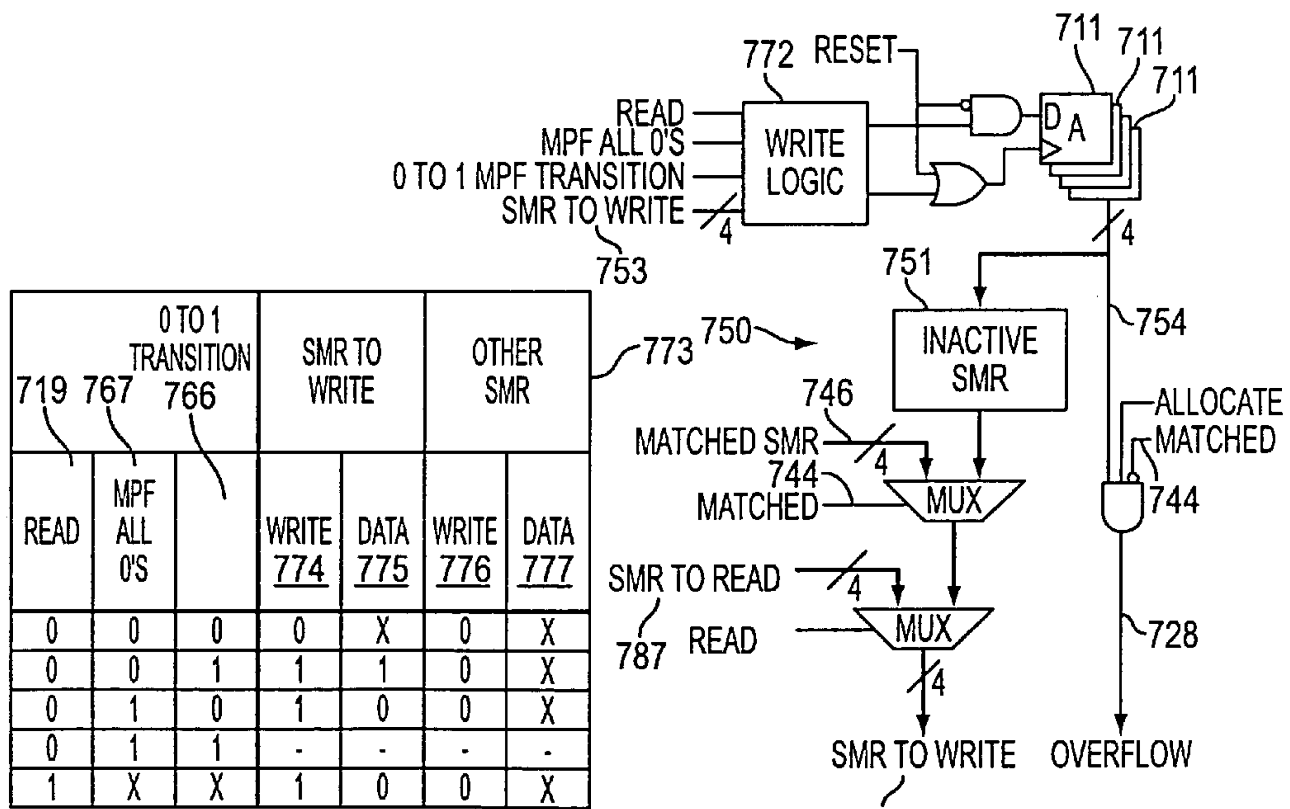
SMR Allocation logic FIG. 7F
