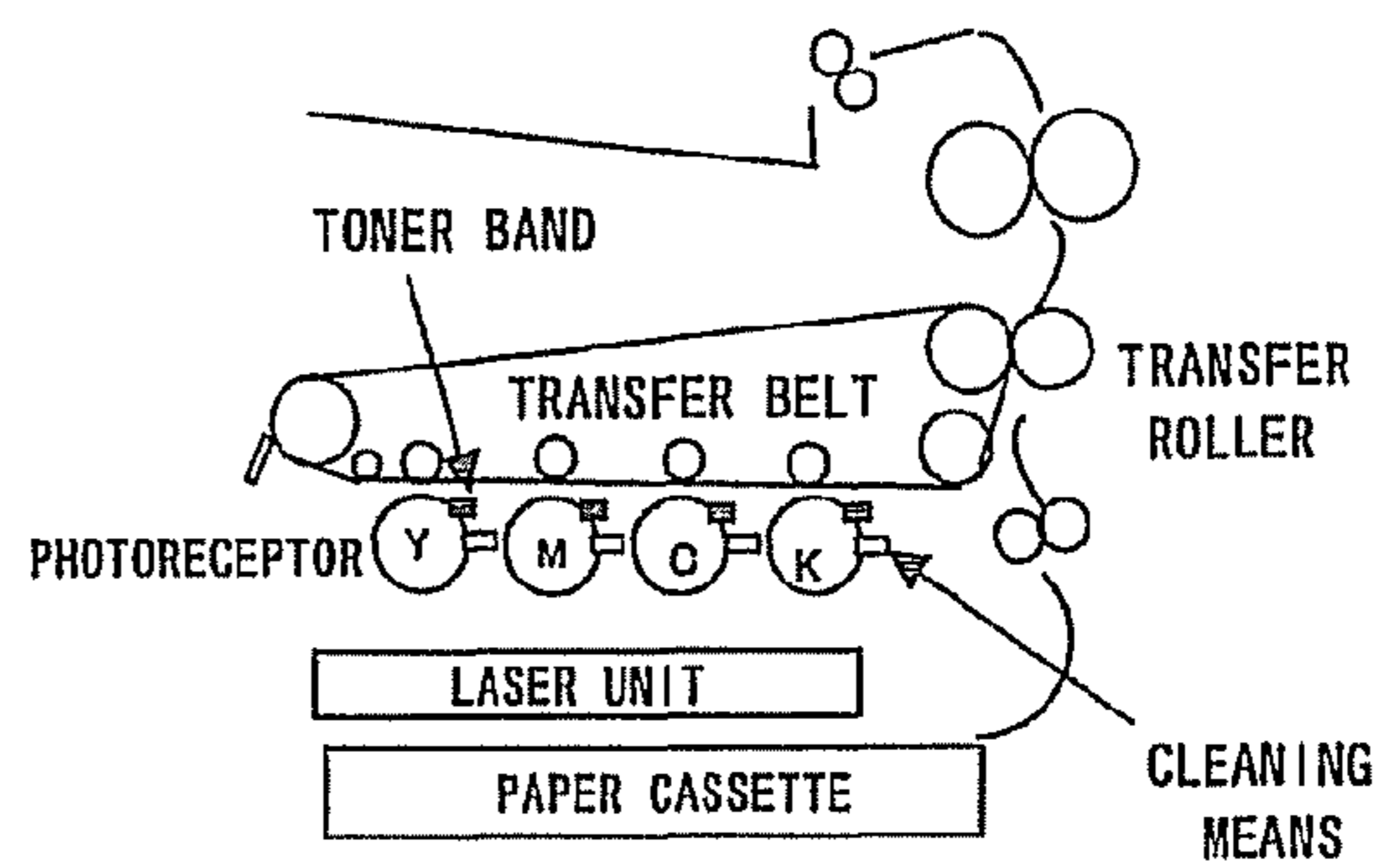
TONER BAND AVOIDING TIMING AT STOPPAGE
