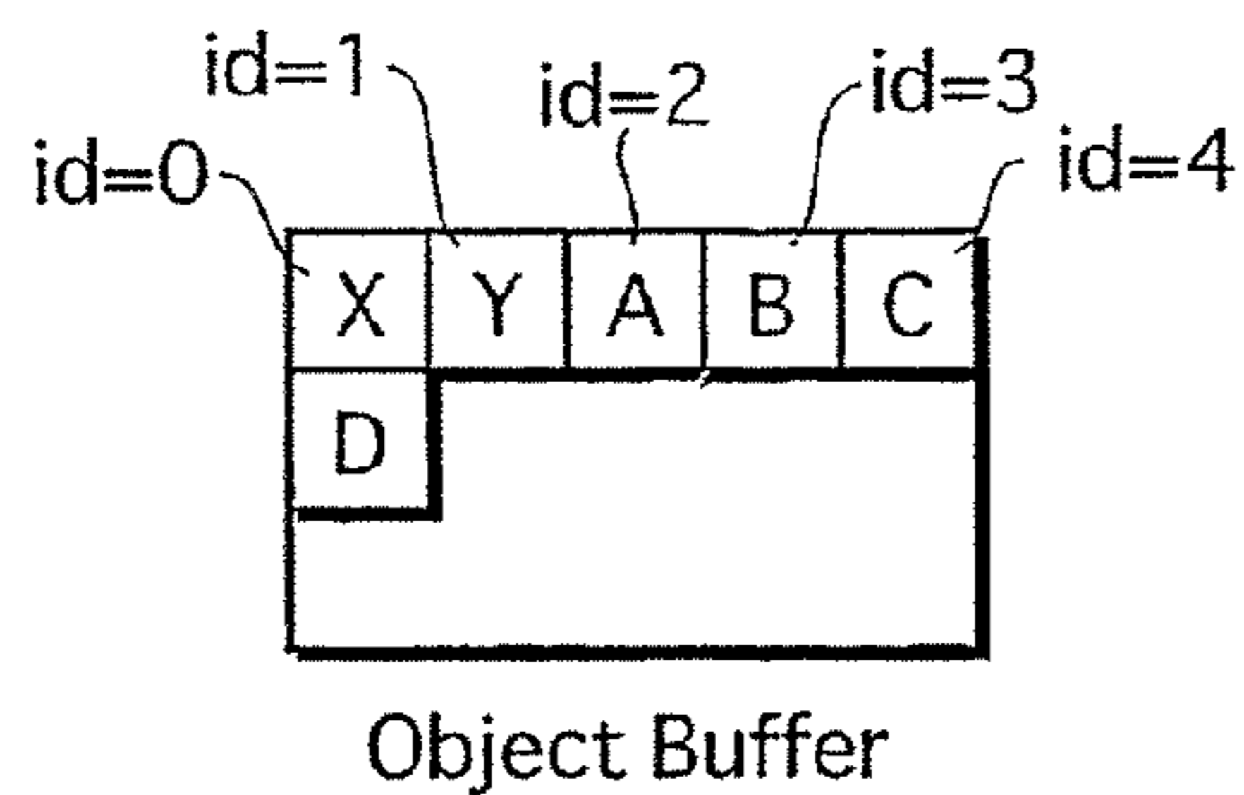
FIG.27C ARRANGEMENT IN OBJECT BUFFER
