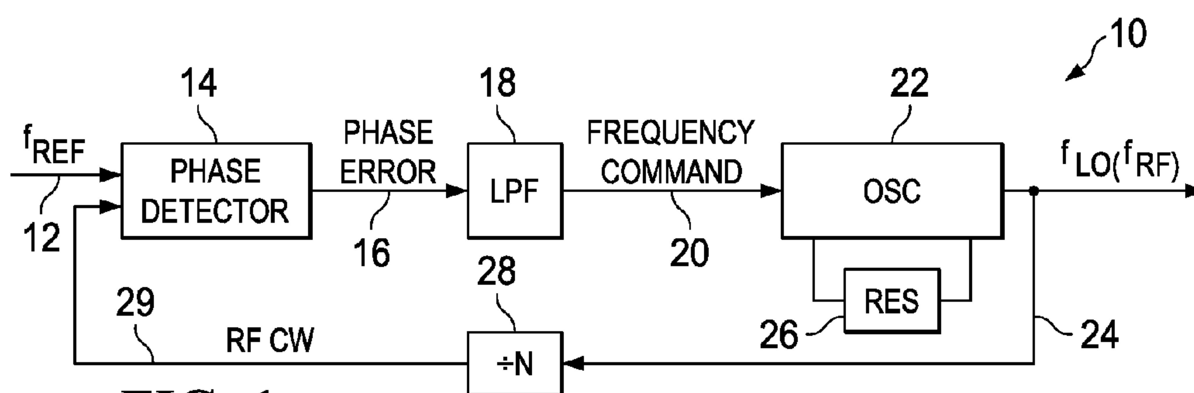
FIG. 1 (PRIOR ART)
