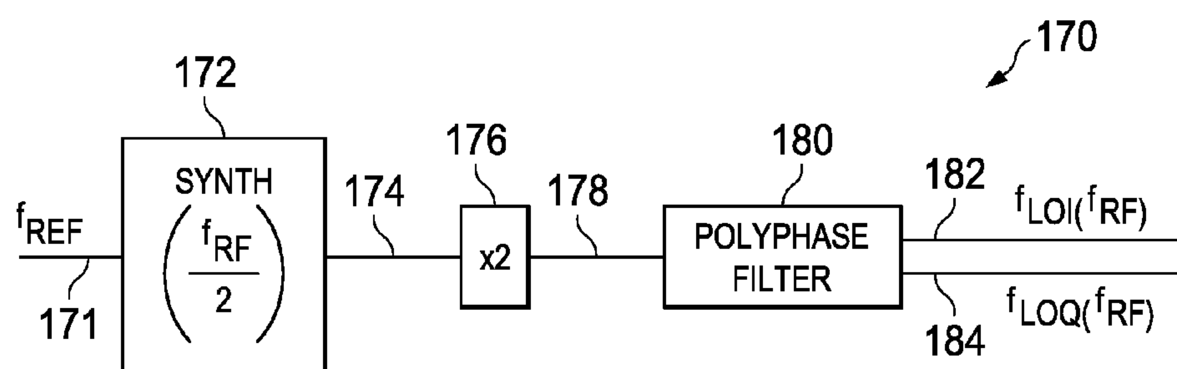
FIG. 2 (PRIOR ART)
