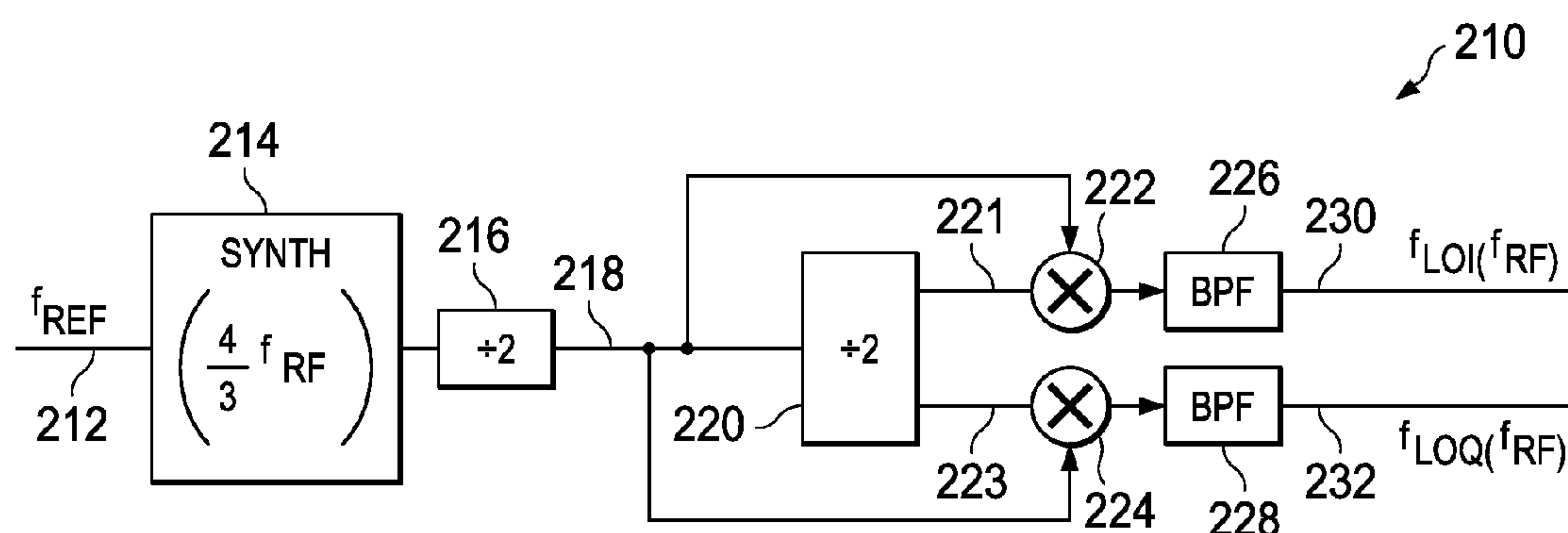
FIG. 4 (PRIOR ART)
