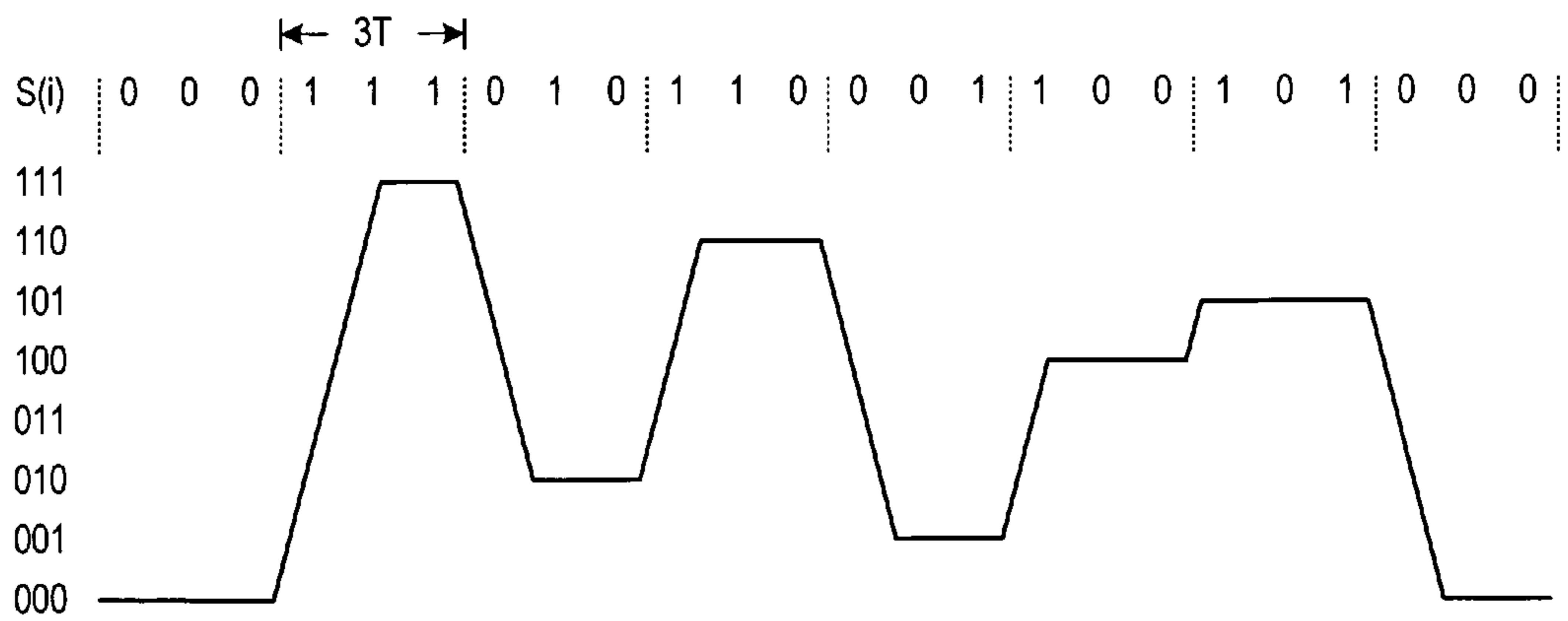
Fig. 1C (Prior Art)
