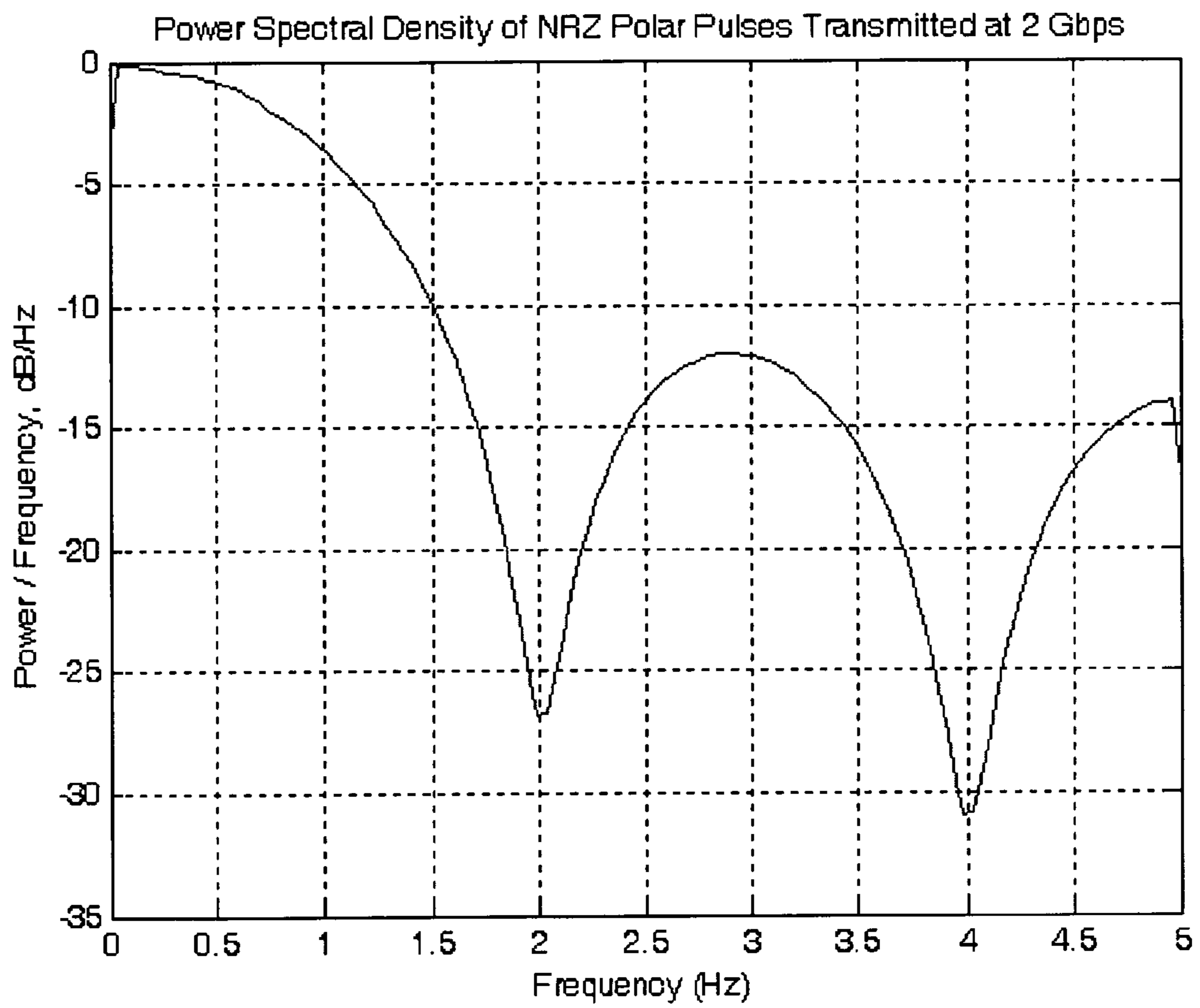
Fig. 2 (Prior Art)
