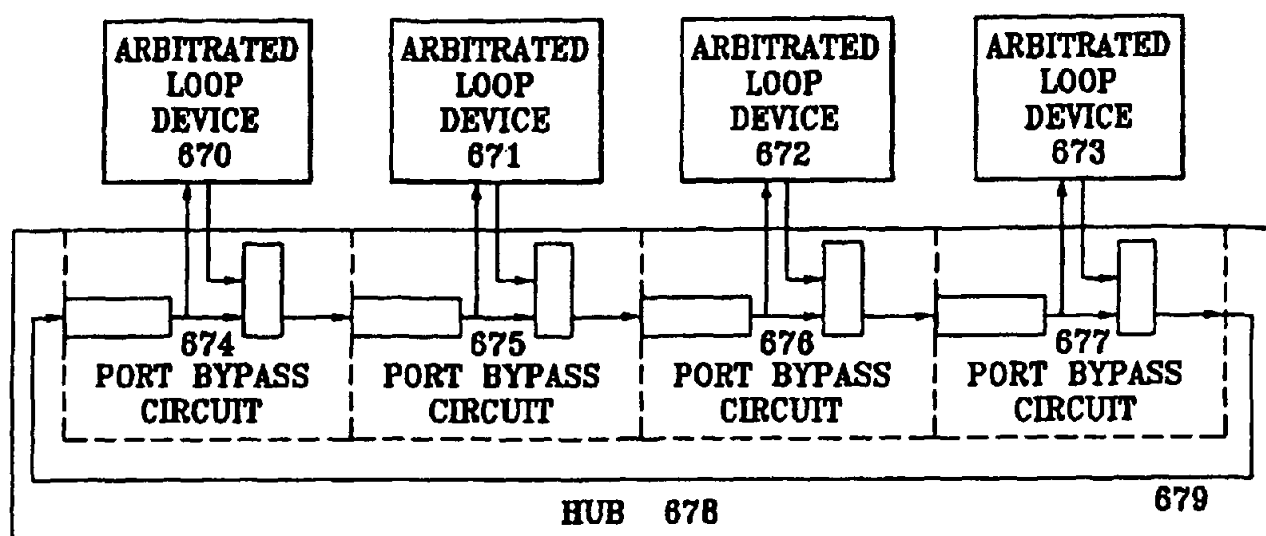
Fig. 22 (PRIOR ART)
