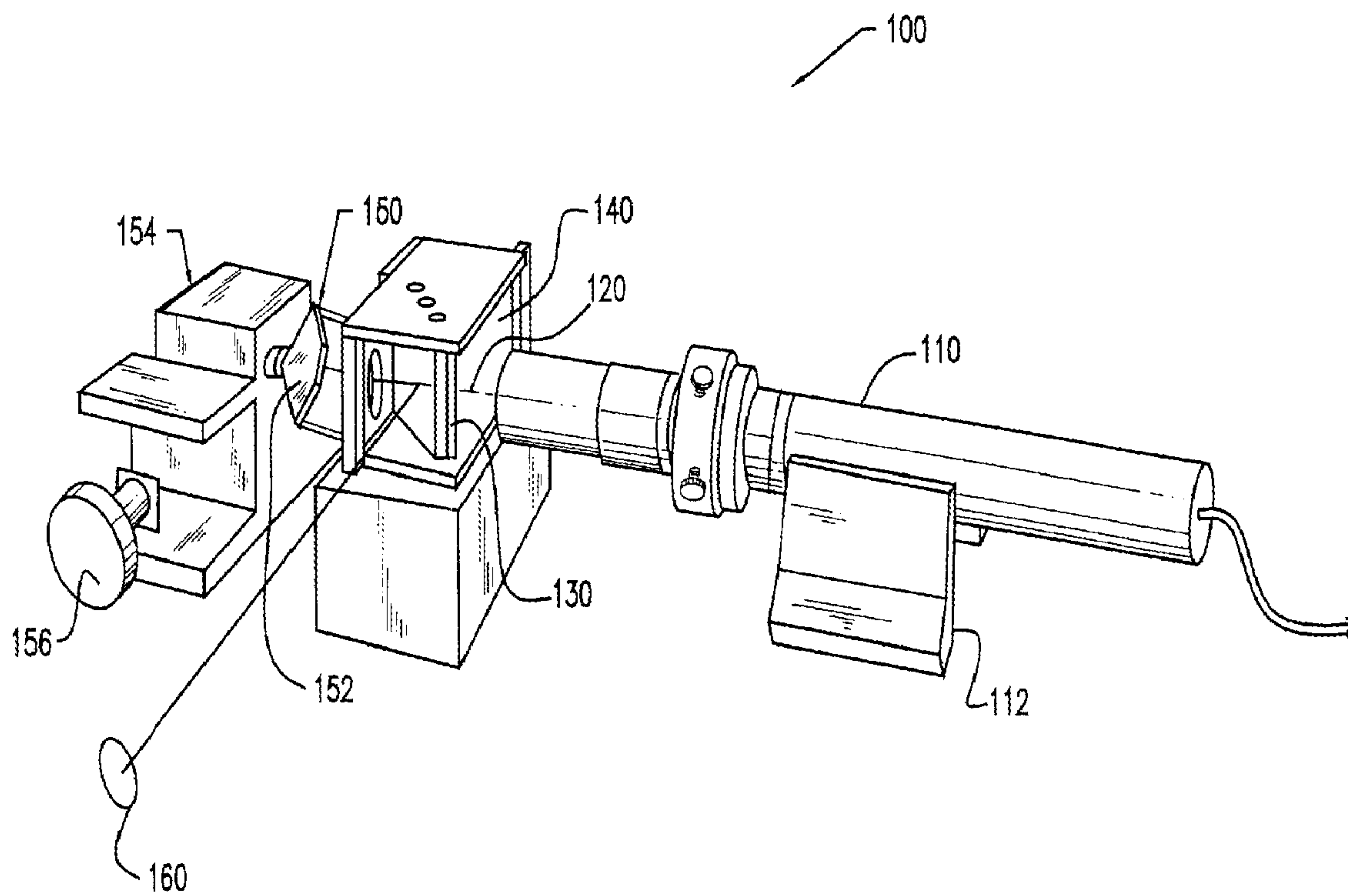
FIG. 2 (PRIOR ART)
