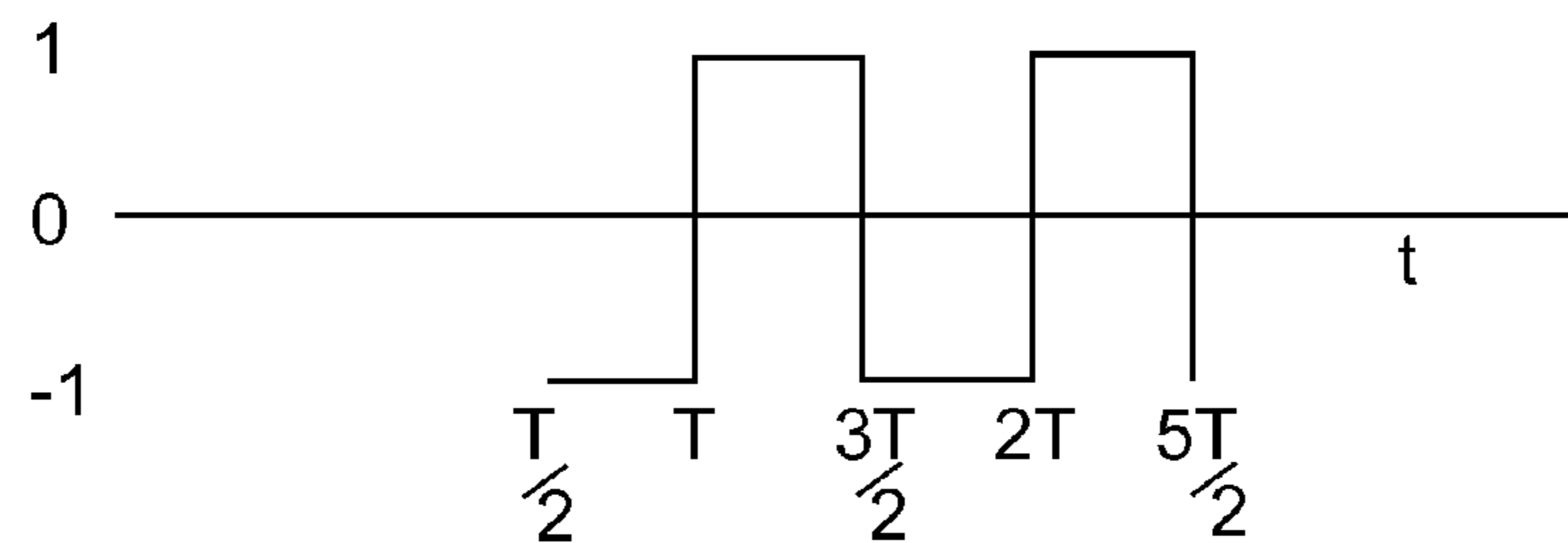
S_0 Reference Waveform-Even (data=0)
