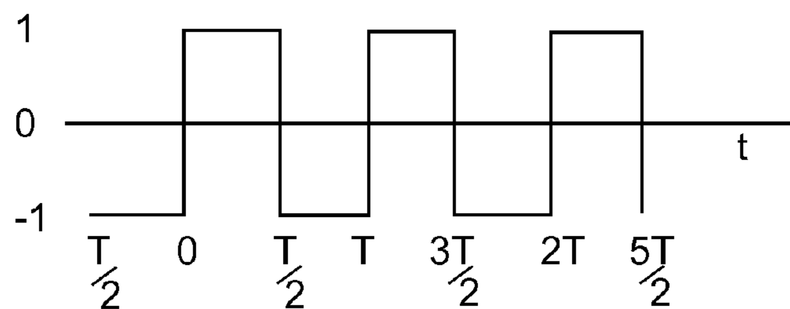
Composite S_0 Reference Waveform (data=0)
