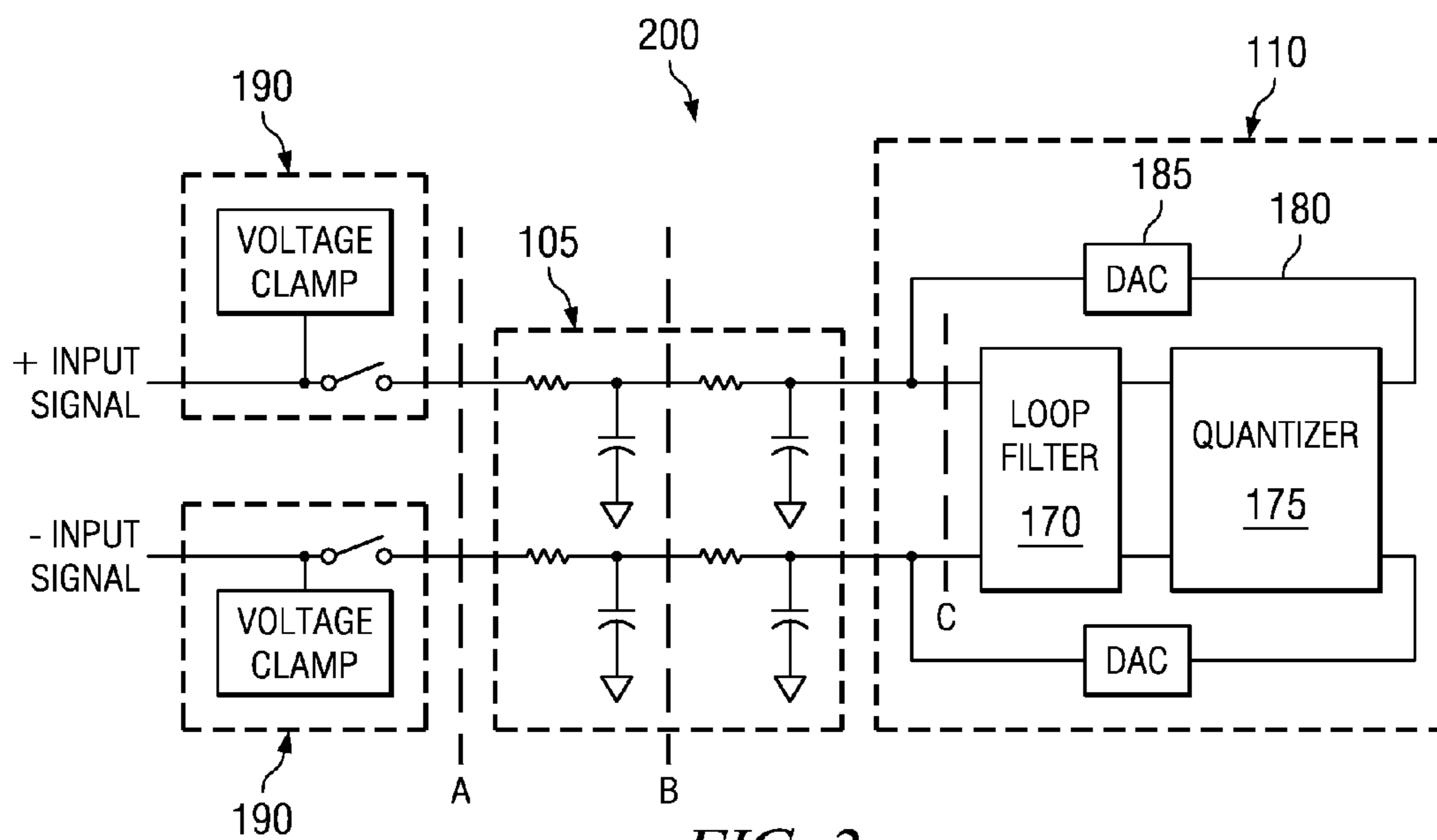
FIG. 2 (PRIOR ART)
