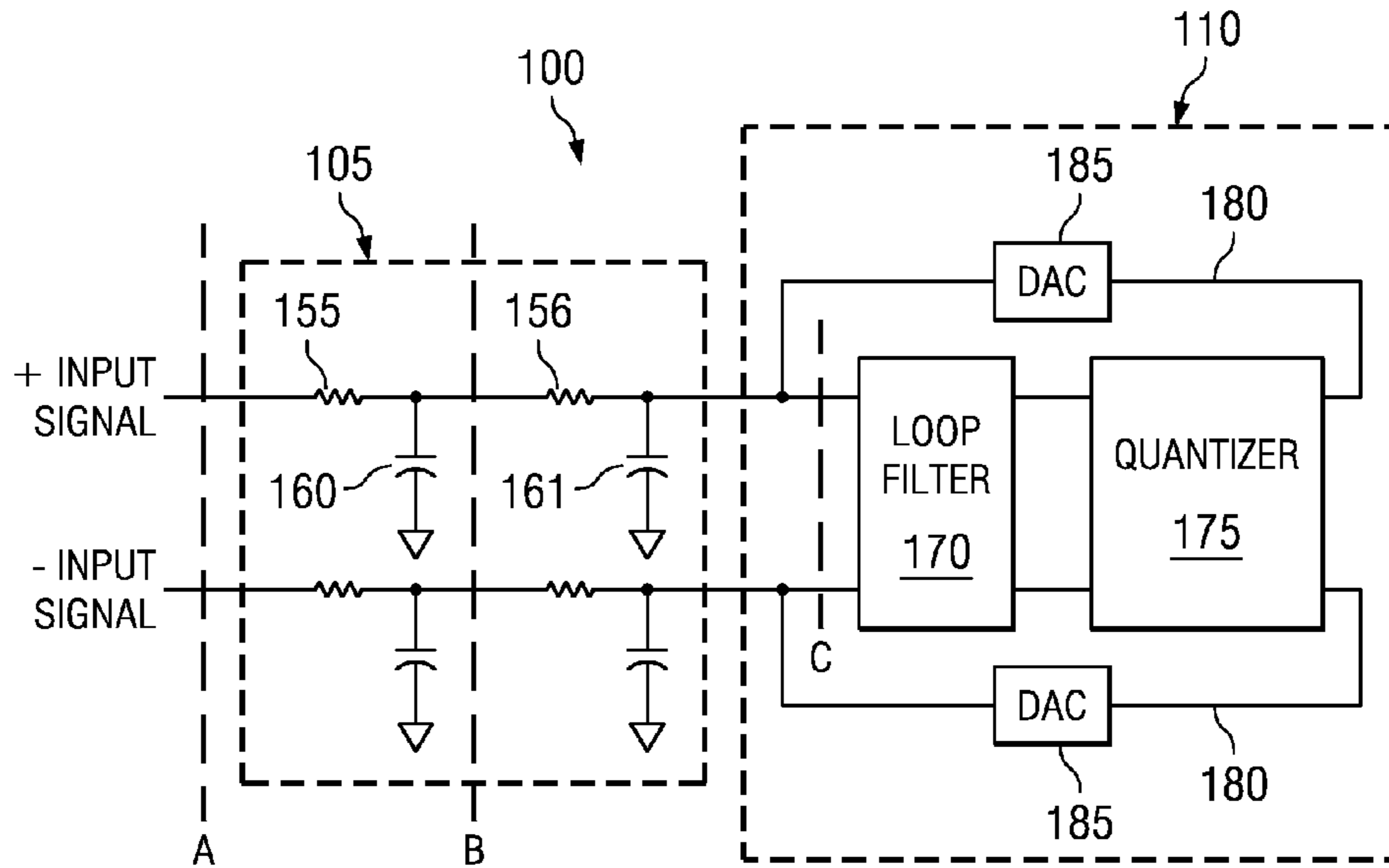
FIG. 1 (PRIOR ART)
