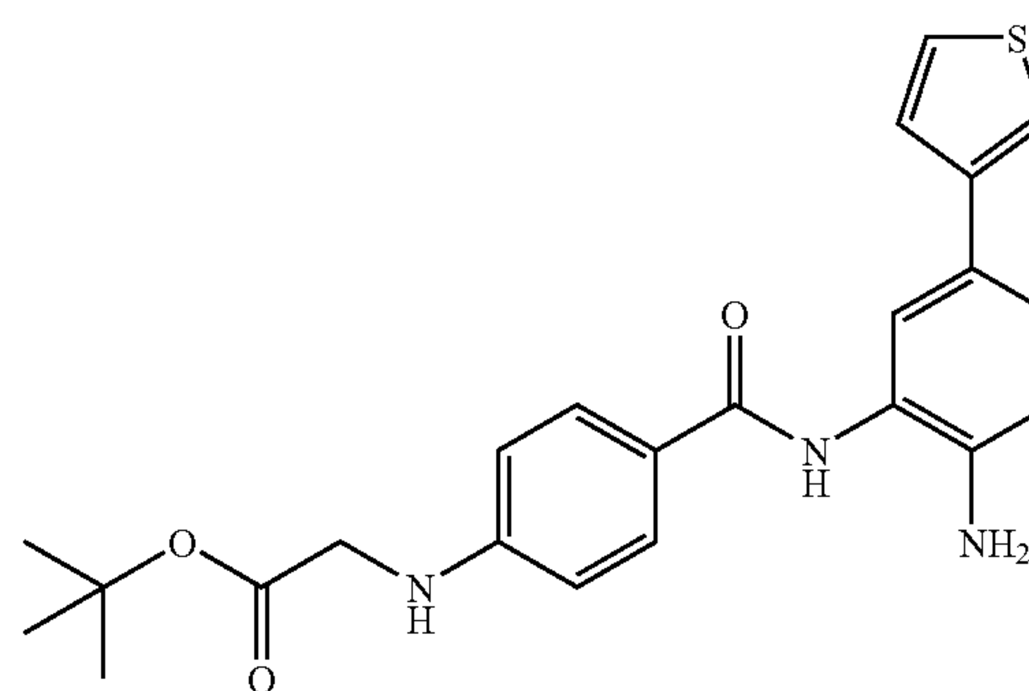
tert-Butyl [(4-([2-amino-5-(3-thienyl)phenyl]amino)carbonyl]phenyl]amino]acetate
