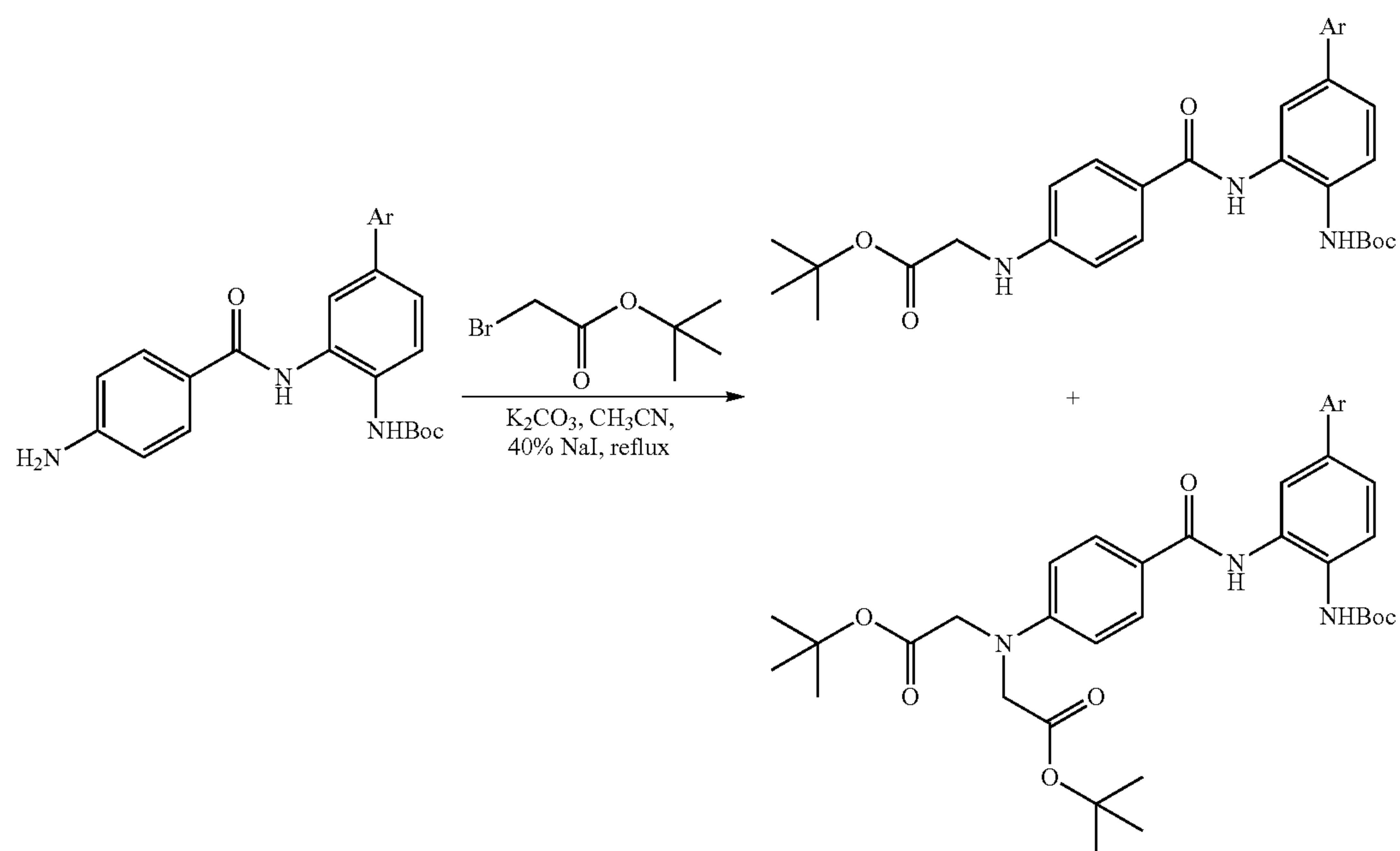
SCHEME 5
