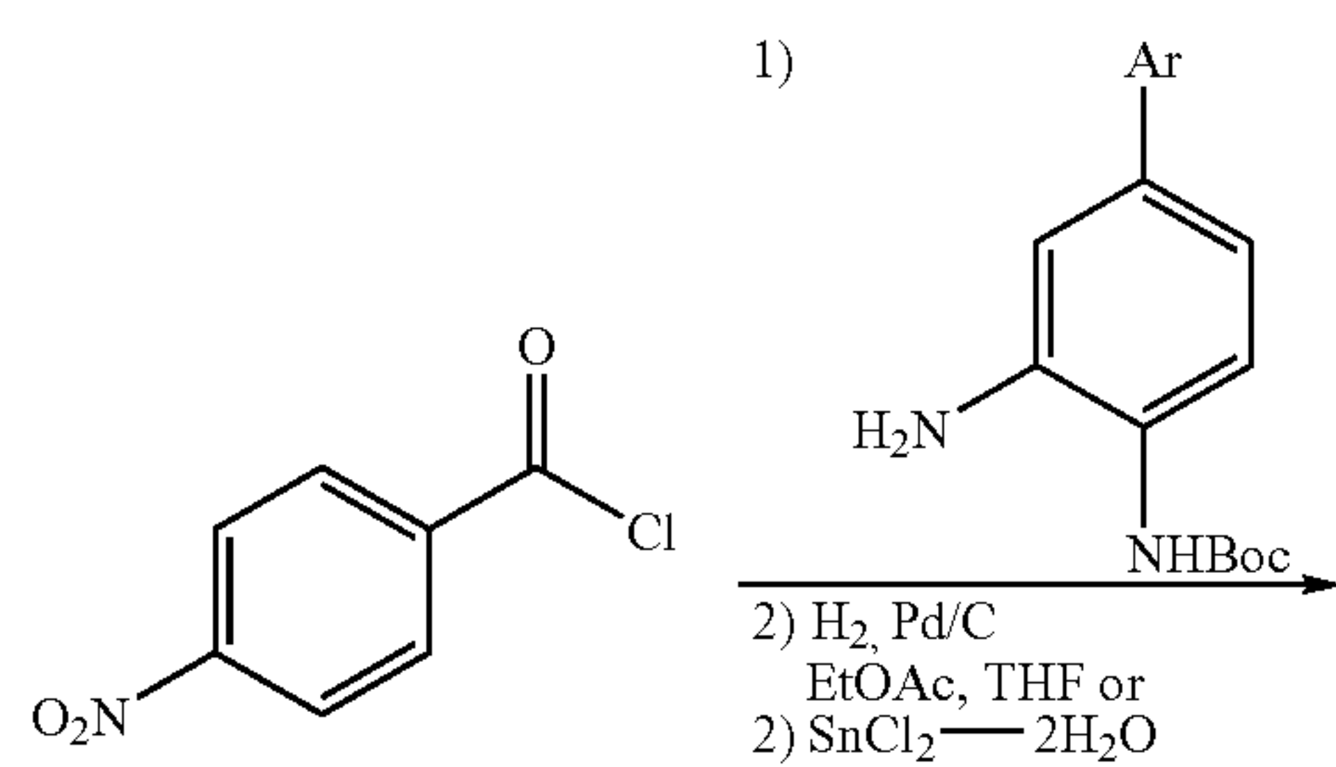
SCHEME 4
