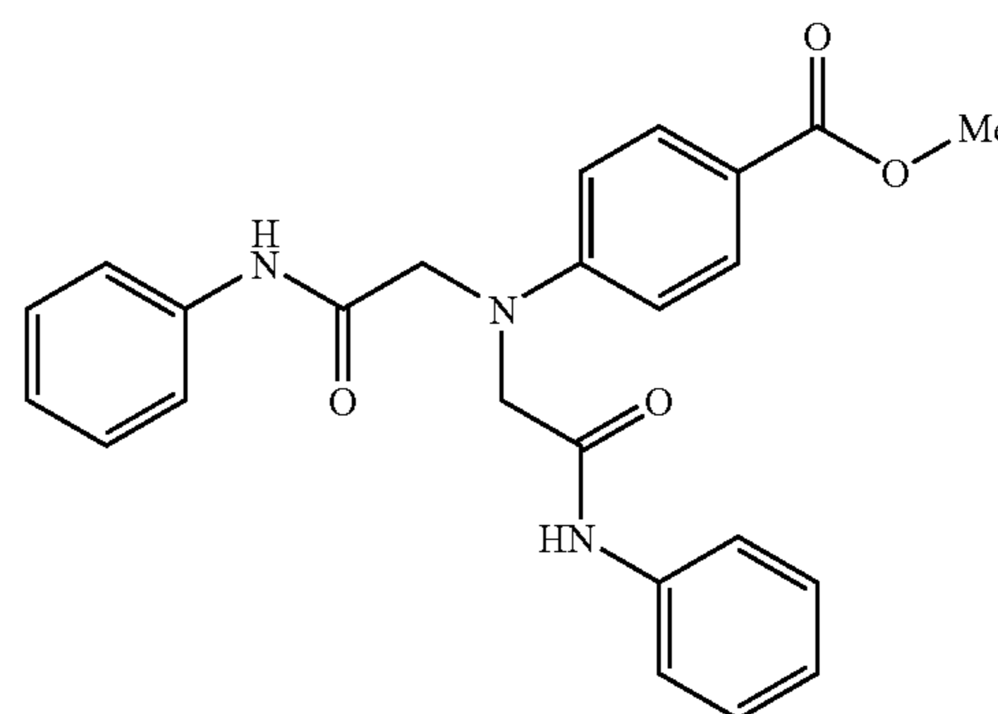
Methyl 4-[bis(2-anilino-2-oxoethyl)amino]benzoate
