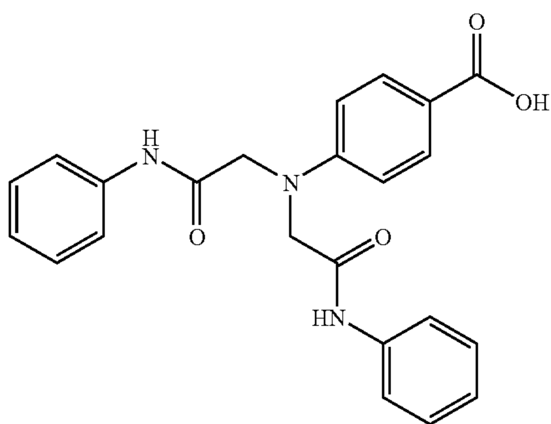
4-[bis(2-anilino-2-oxoethyl)amino]benzoic acid
