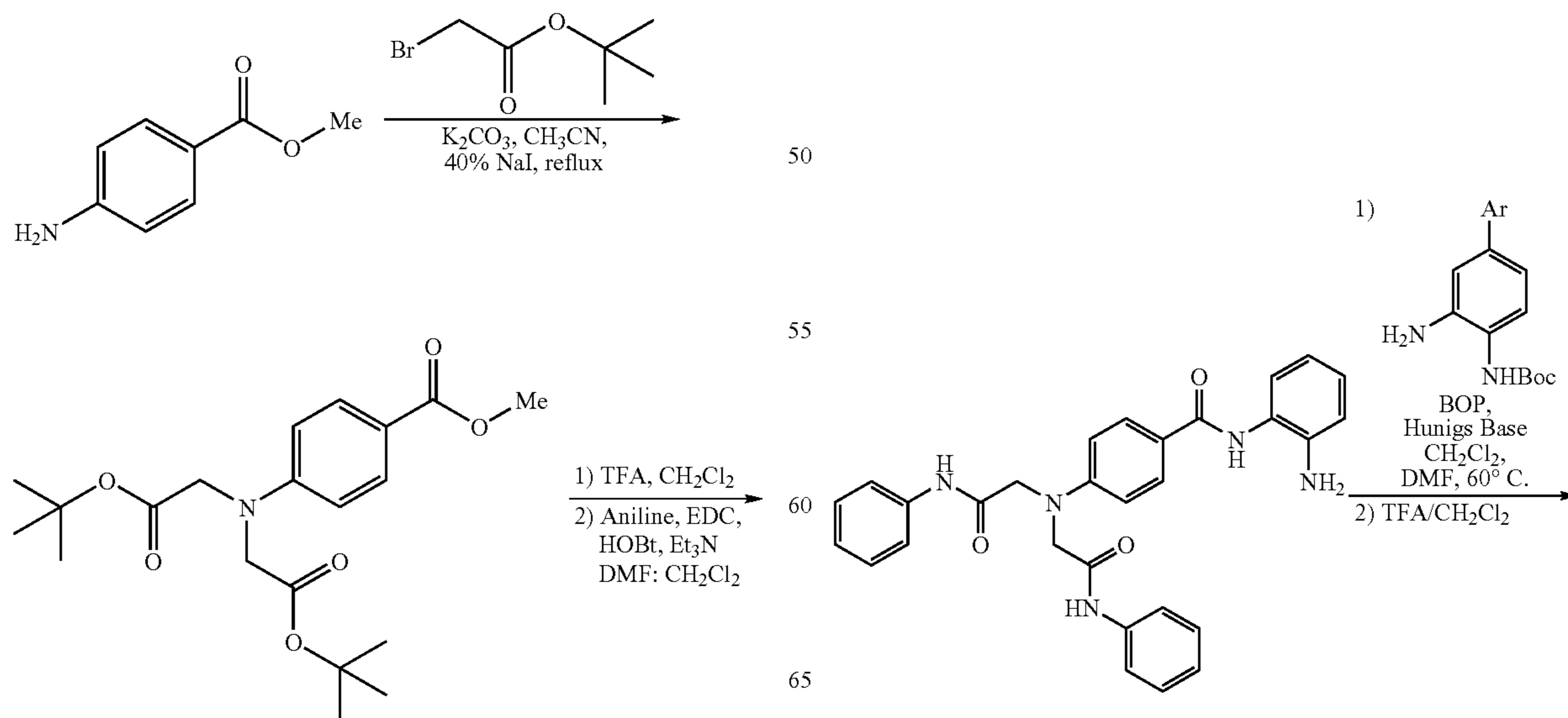
SCHEME 3
