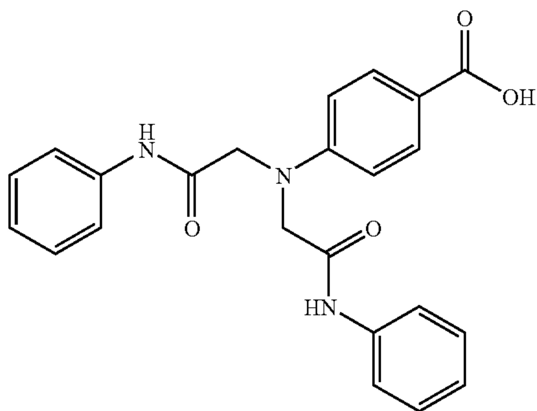
4-[bis(2-anilino-2-oxoethyl)amino]benzoic acid
