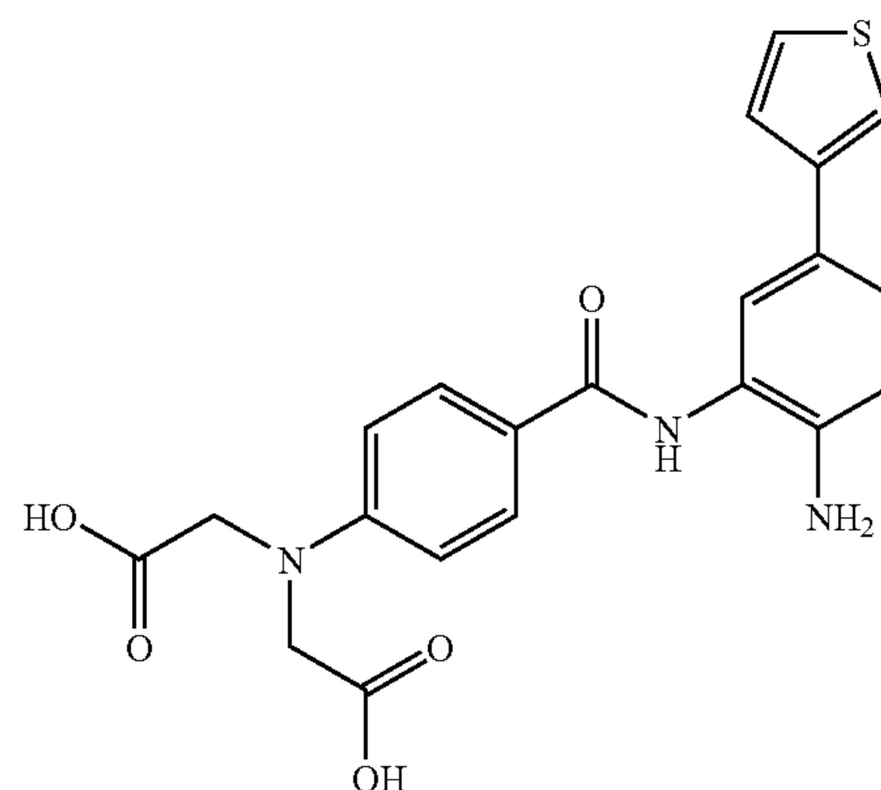
2,2'-[4-([2-amino-5-(3-thienyl)phenyl]amino)carbonyl]phenyl]imino}diacetic acid
