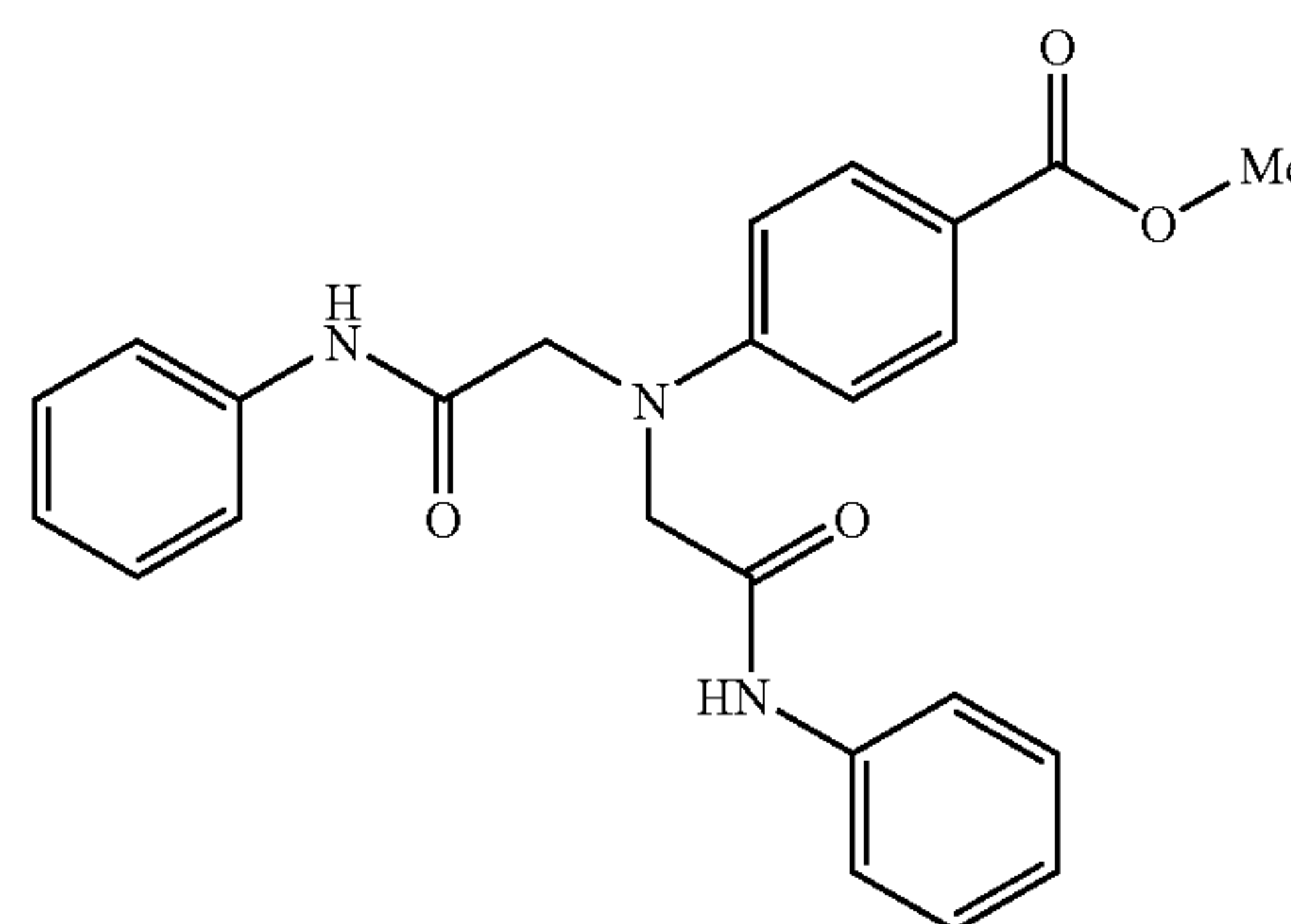
Methyl 4-[bis(2-anilino-2-oxoethyl)amino]benzoate
