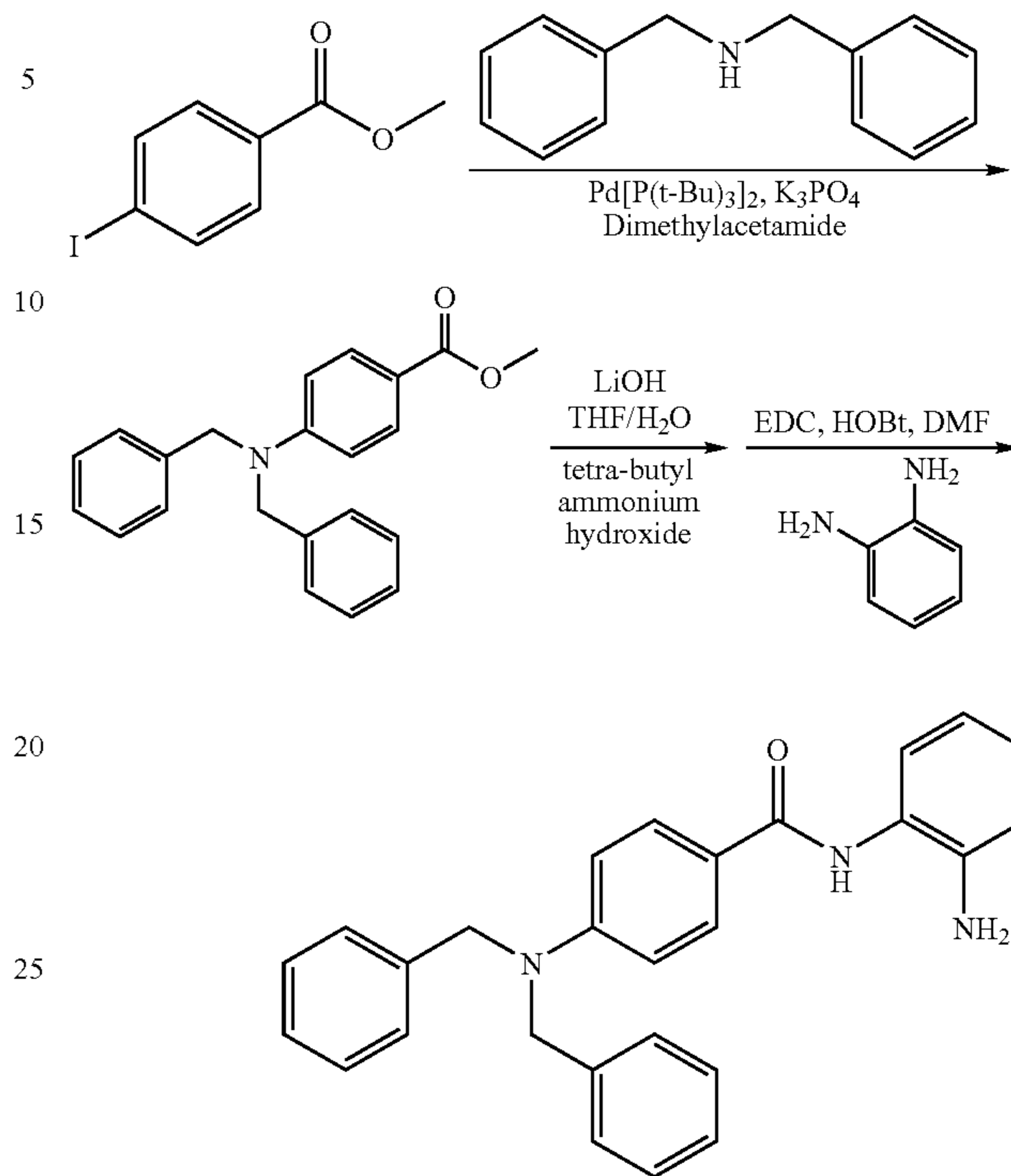
SCHEME 1
