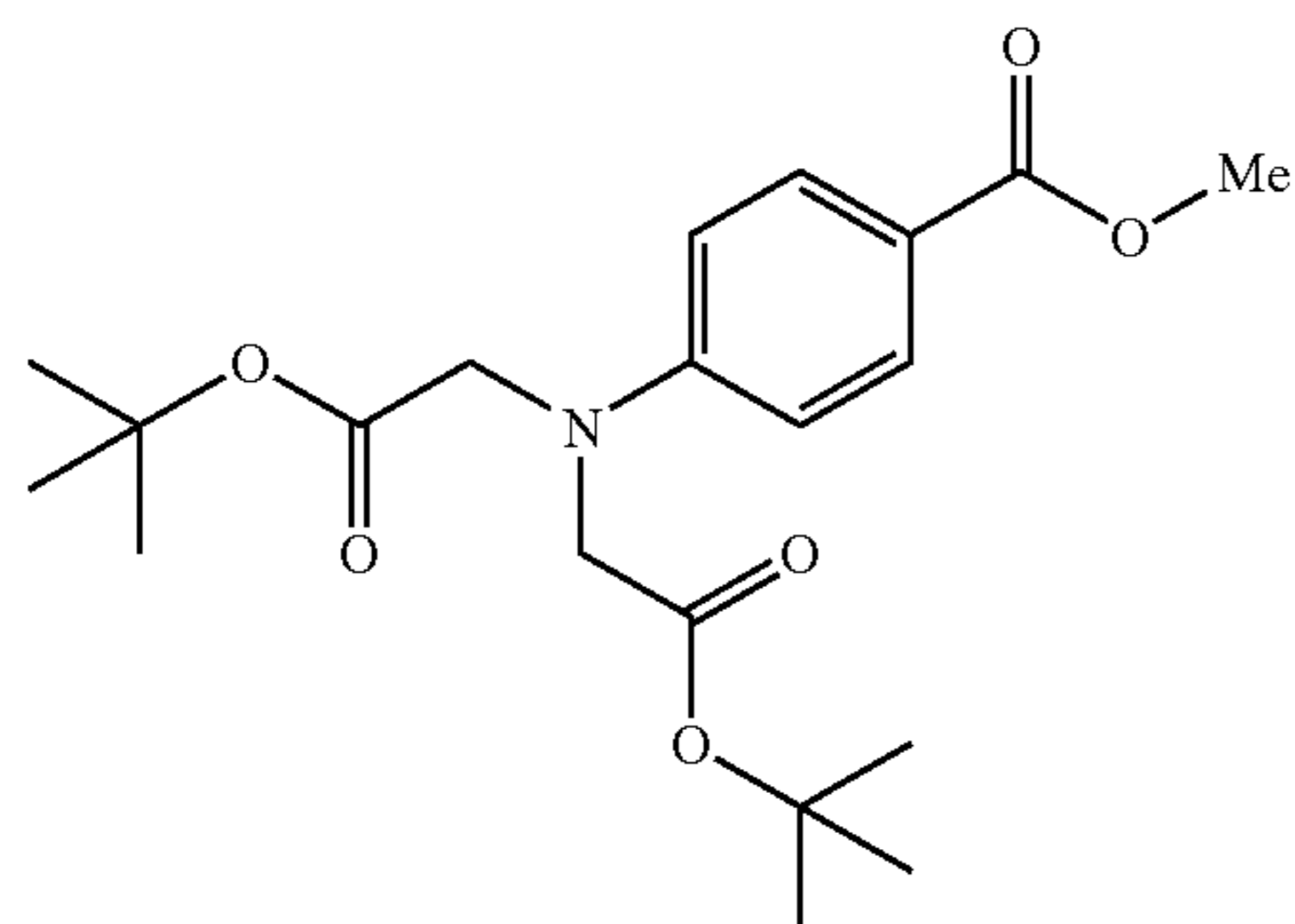
Methyl 4-[bis(2-tert-butoxy-2-oxoethyl)amino]benzoate
