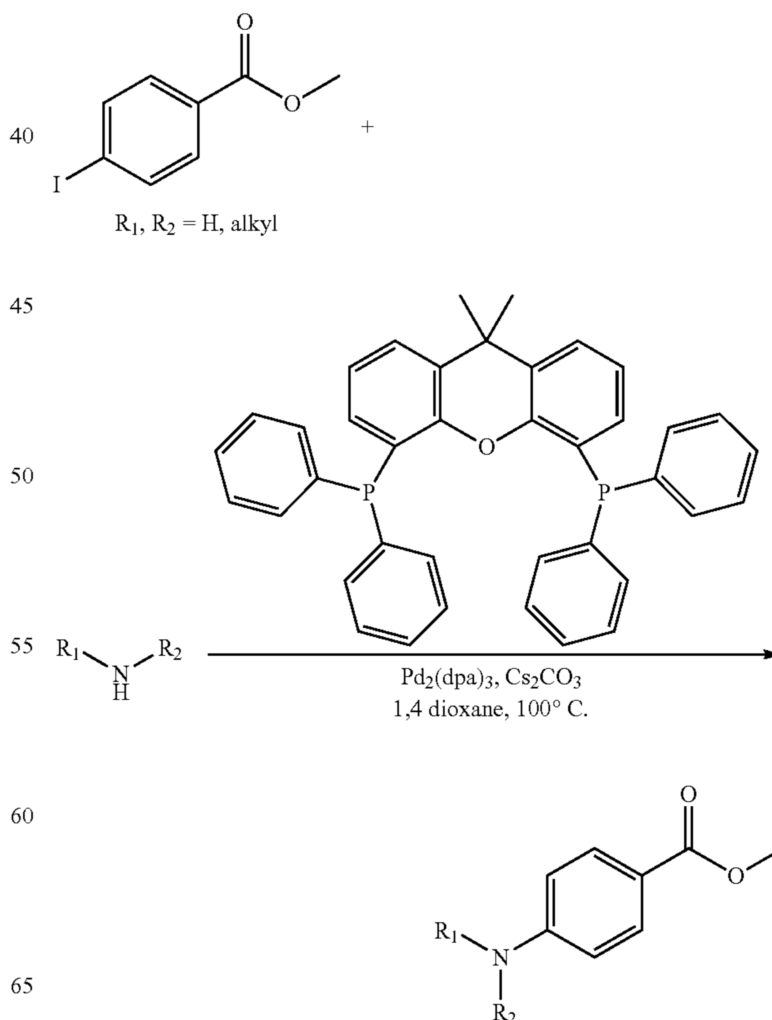
SCHEME 2
