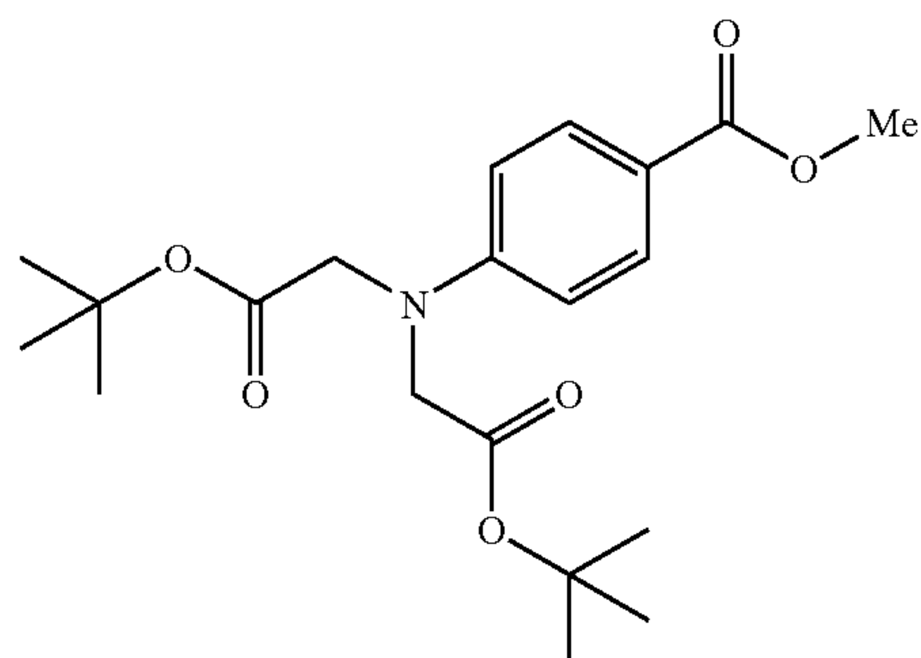
Methyl 4-[bis(2-tert-butoxy-2-oxoethyl)amino]benzoate
