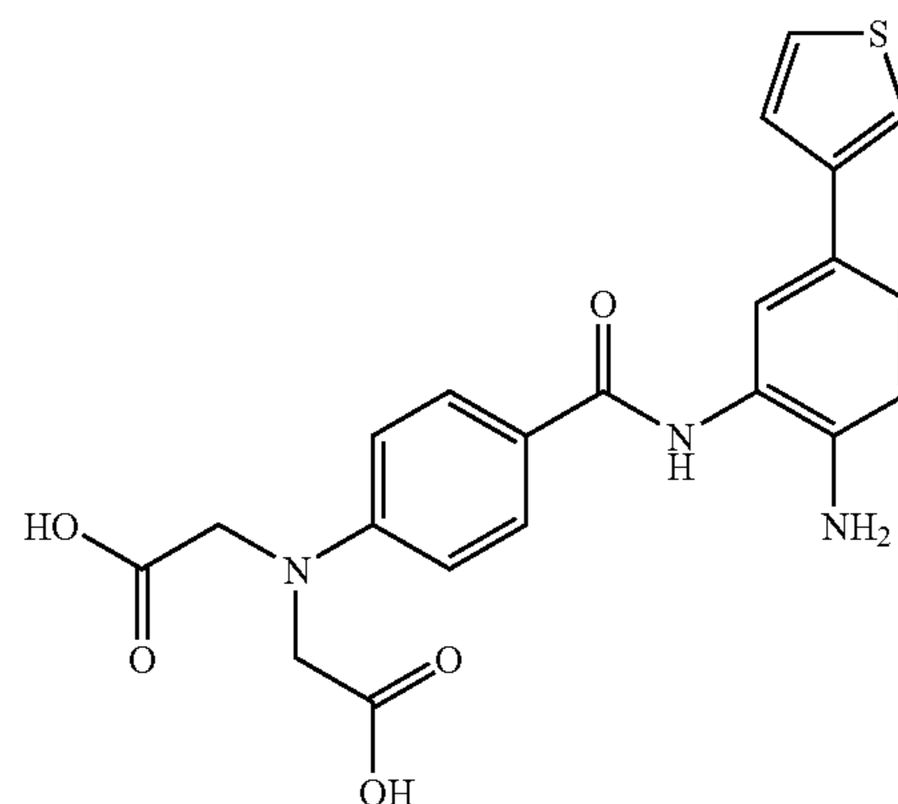
2,2'-[4-([2-amino-5-(3-thienyl)phenyl]amino)carbonyl]phenyl]imino}diacetic acid
