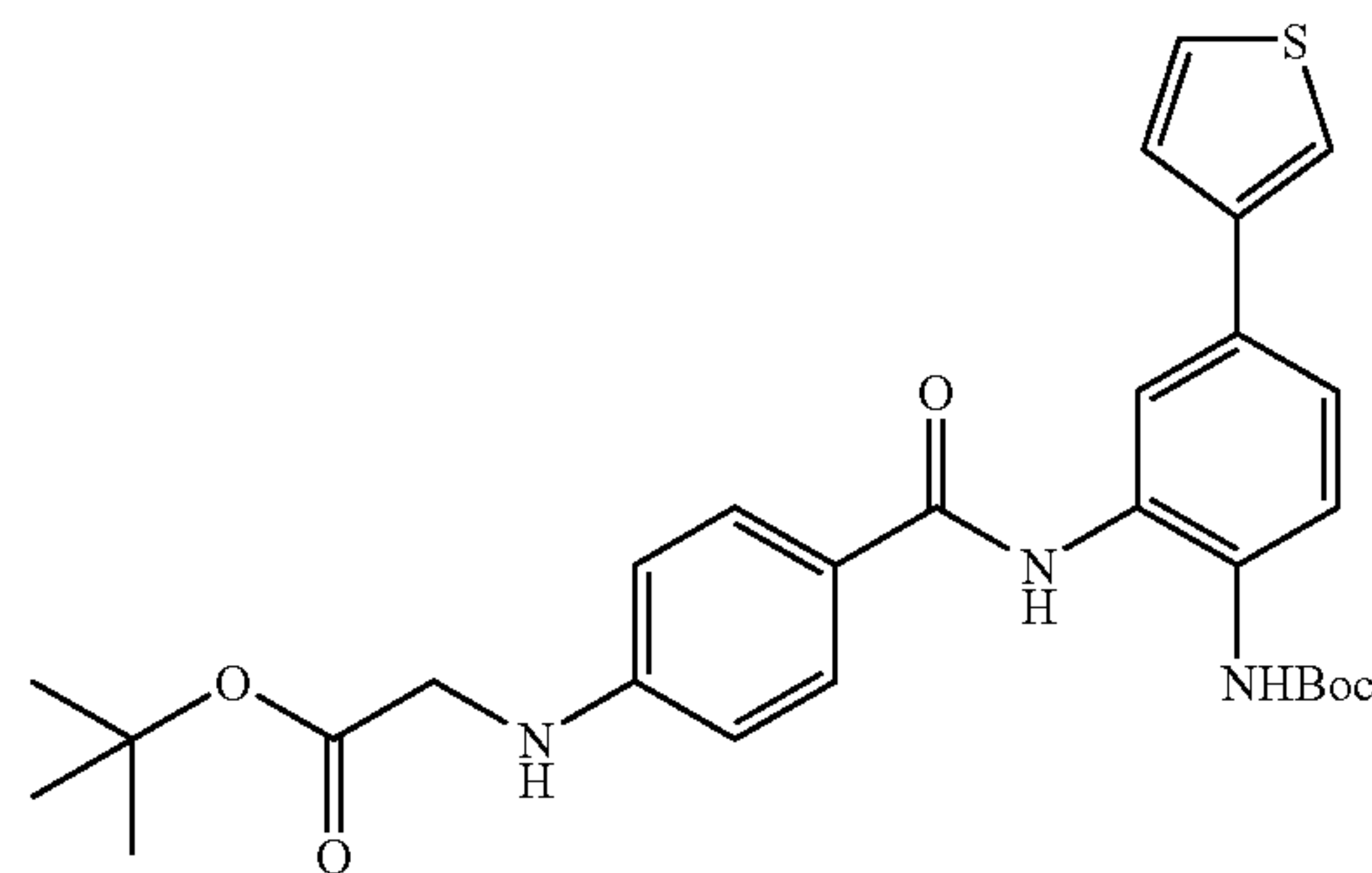
tert-Butyl {4-([2-[(tert-butoxycarbonyl)amino]-5-(3-thienyl)phenyl]amino)carbonyl]phenyl]amino}acetate
