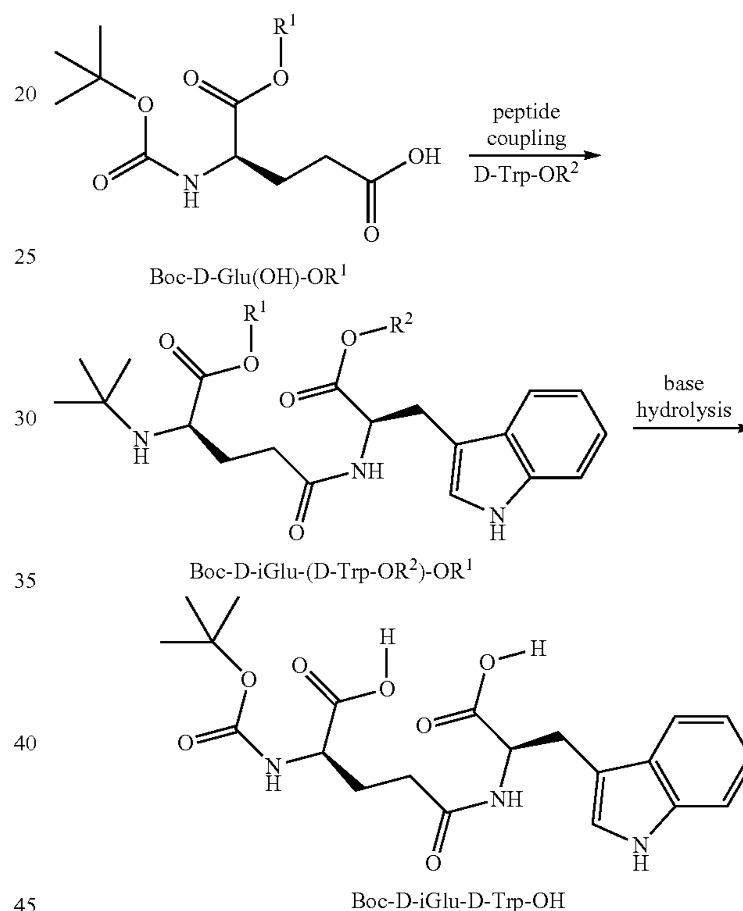
Scheme 5
