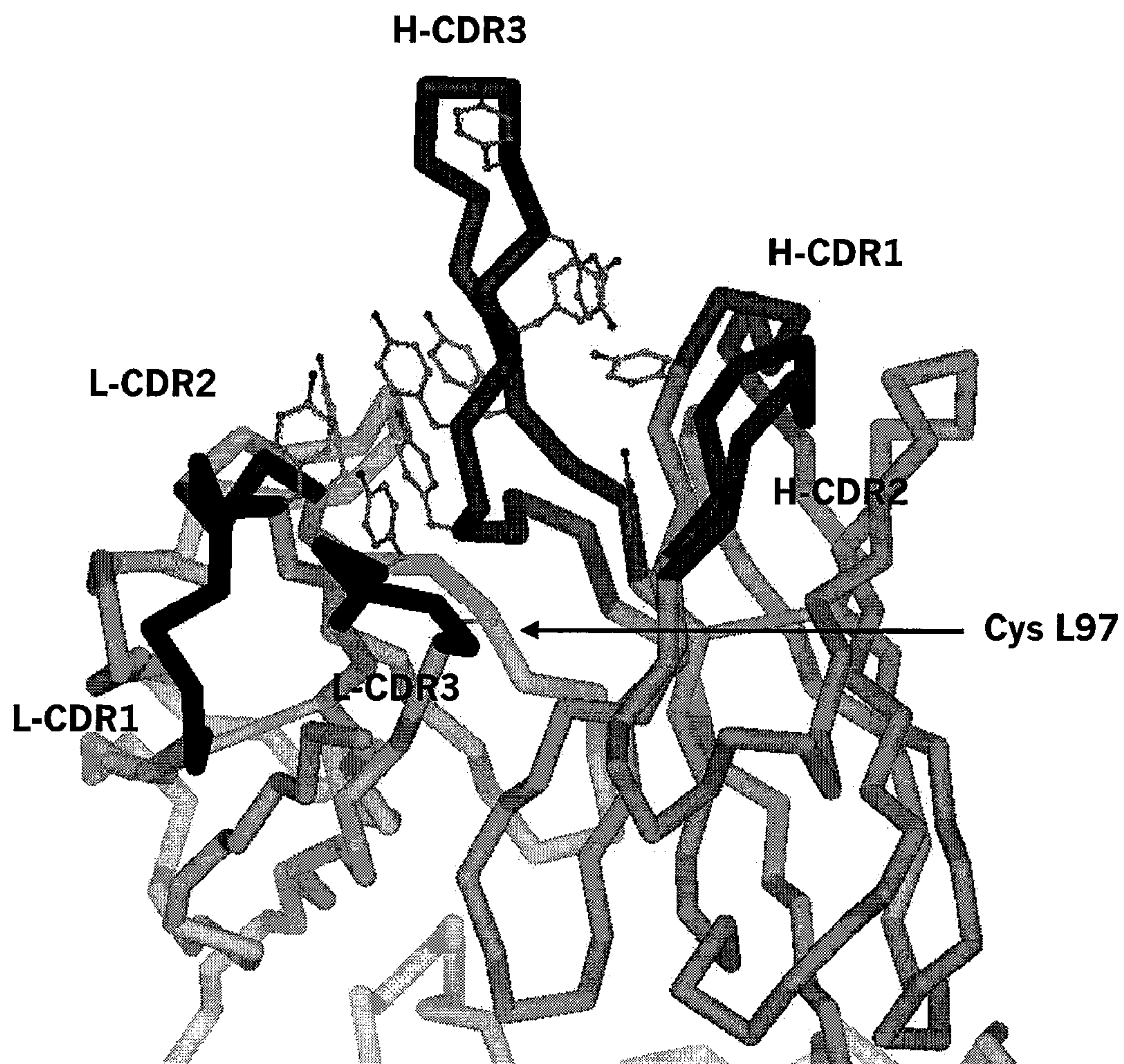
Figure 1. X-ray structure of AIN457 Fab
