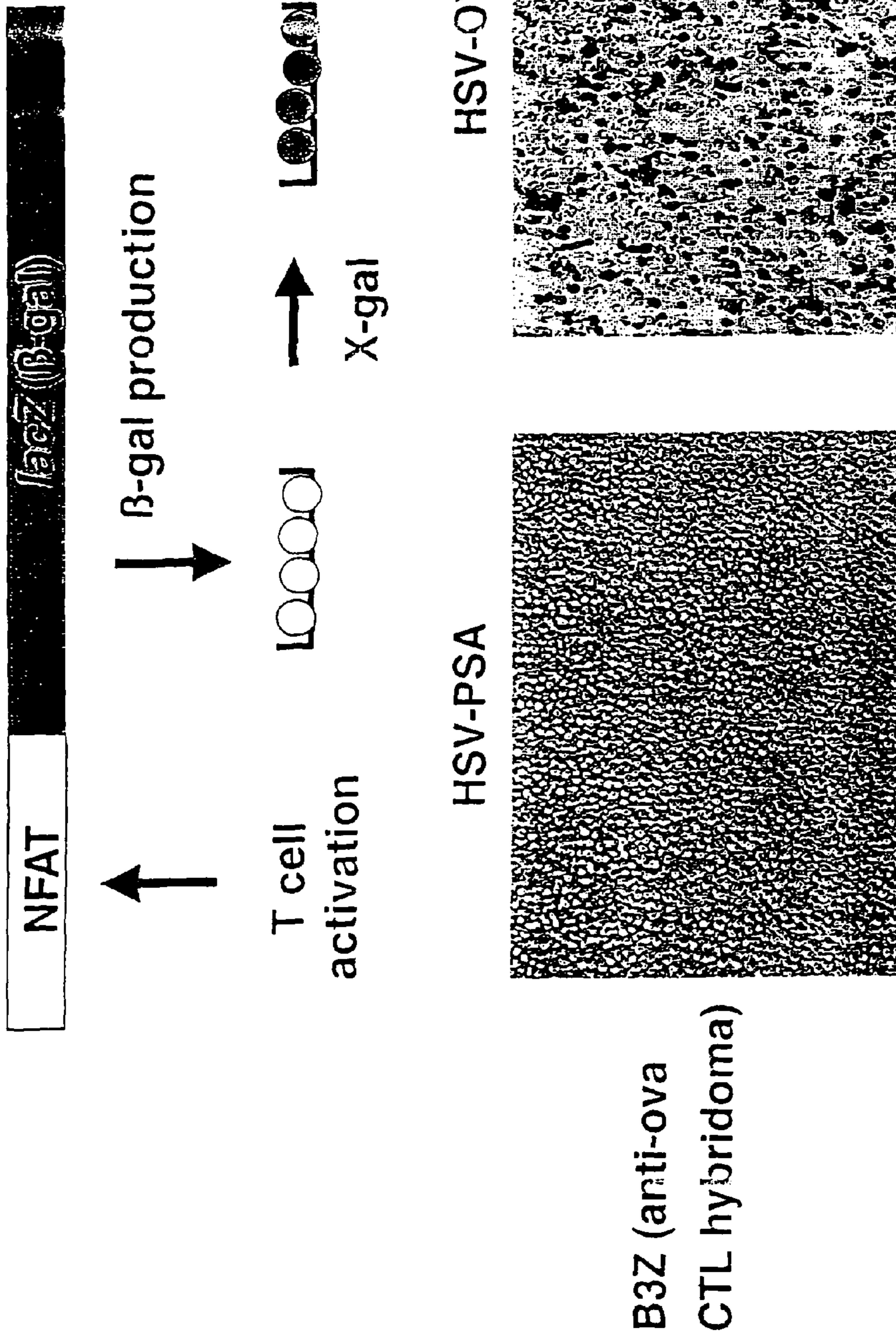
Figure 2: Dendritic cells infected with HSV amplicons present antigen to T cell hybridomas. DCs from a (C57BL/6 x BALB/clyJ)F1 mouse were infected with HSV-OVA and cultured overnight with CTL hybridoma B3Z (specific for OVA). These hybridomas have been previously transfected with lacZ under control of the IL-2 promoter and can be assayed for activation by staining with X-gal. Blue cells represent activated hybridomas and indicate that the DCs have been transduced and are capable of processing the OVA for class I MHC presentation.
