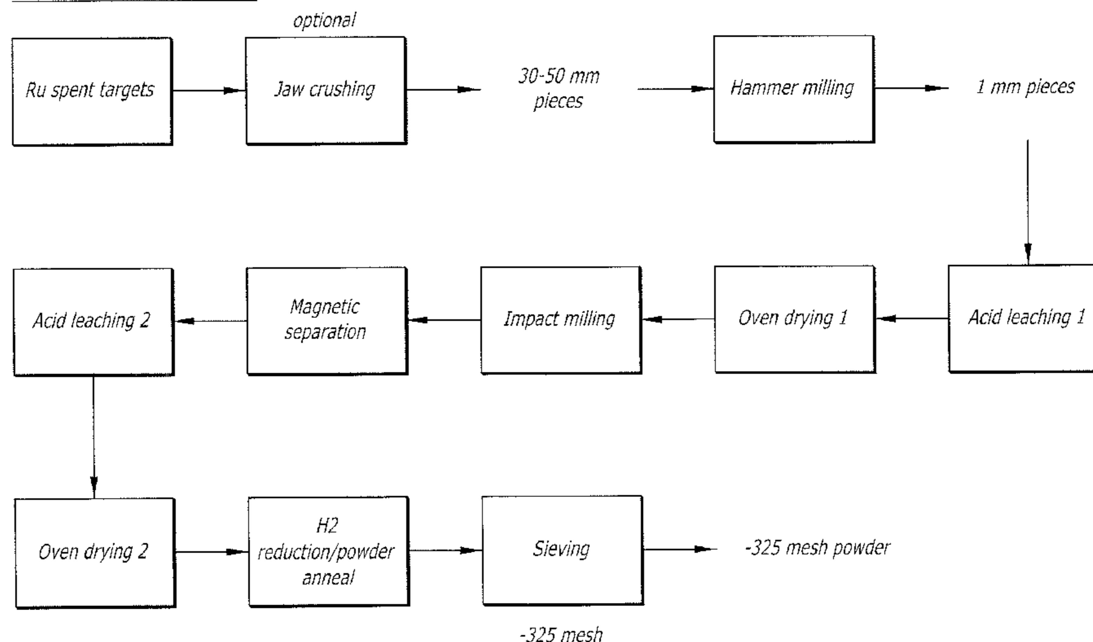
Ru Target Recycle Process Flow
