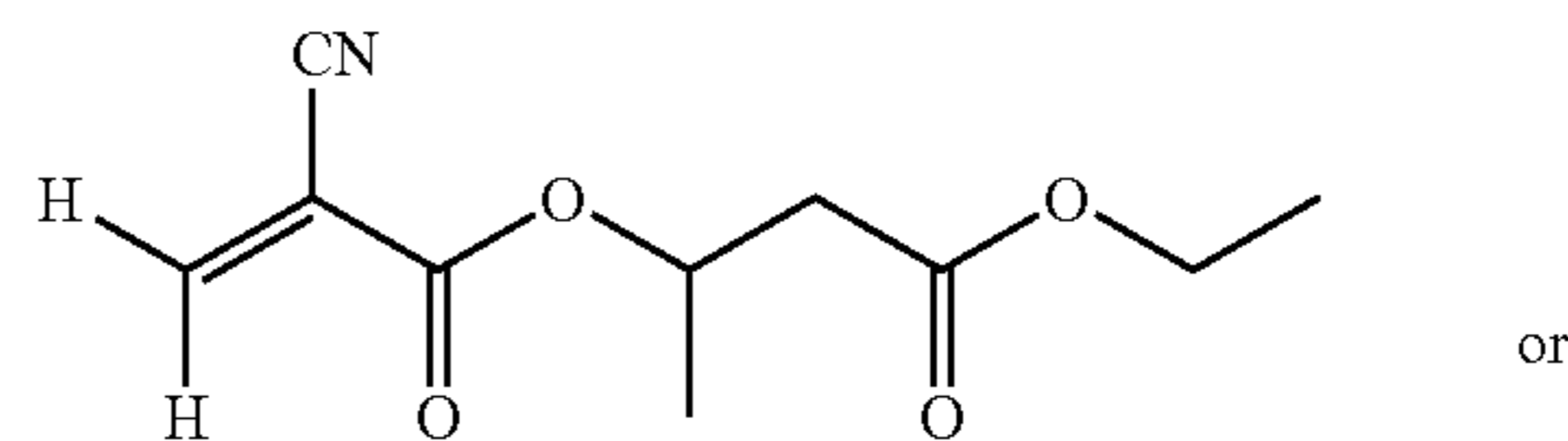
3-(2-Cyano-acryloyloxy)-butyric acid ethyl ester (Et- \beta -HBT-CA)
