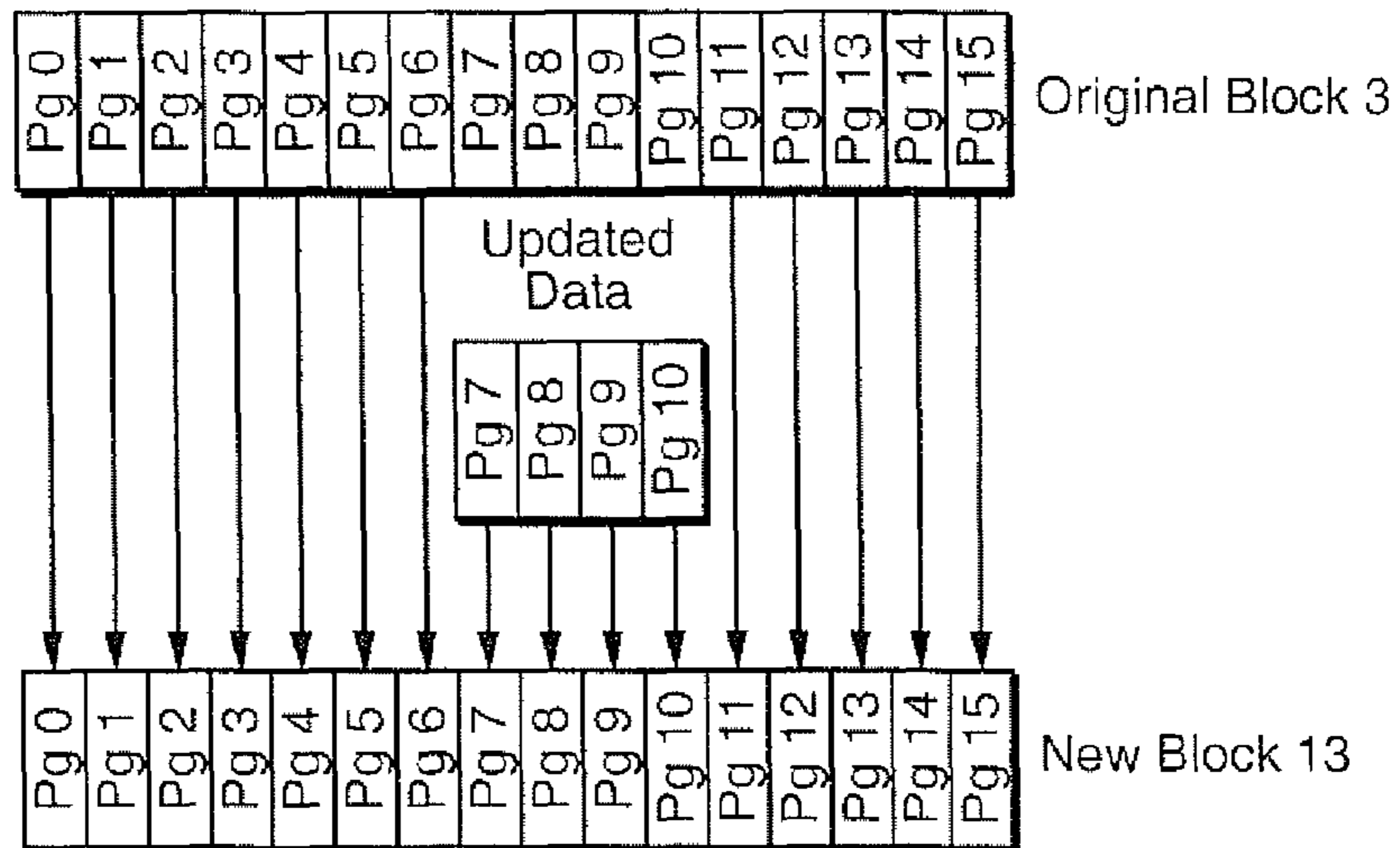
FIG. 6 (PRIOR ART)
