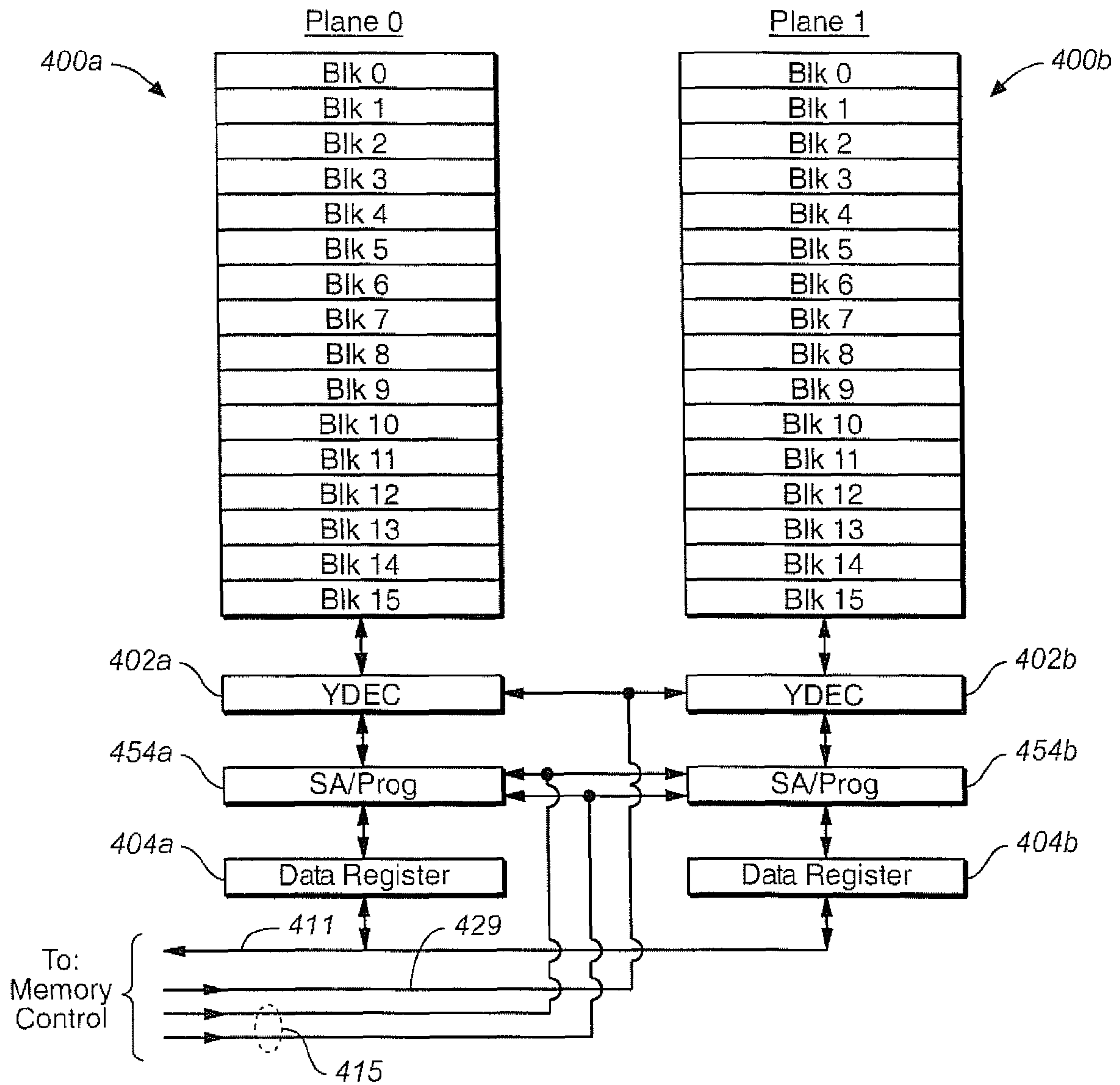
FIG. 3 (PRIOR ART)
