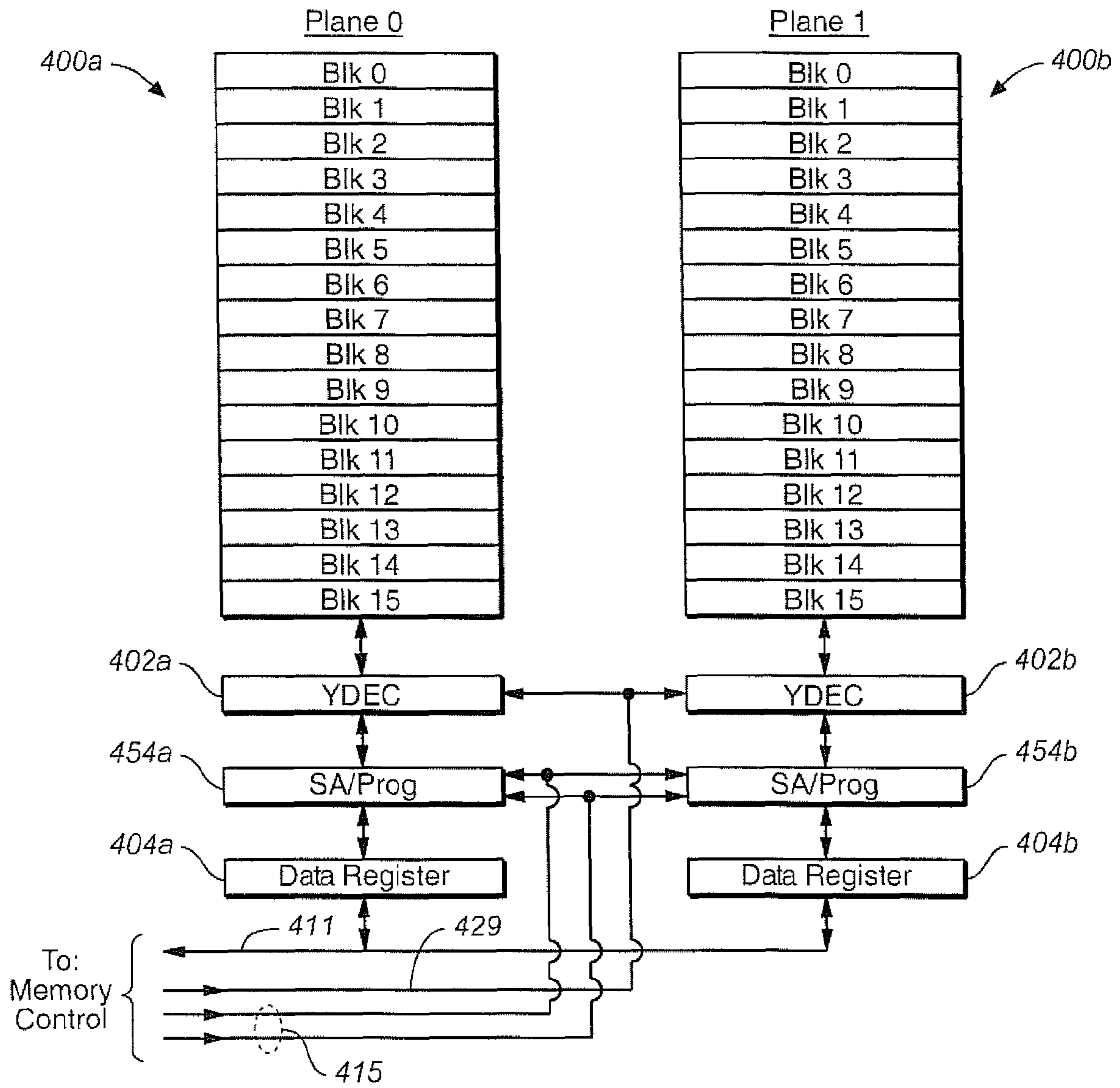
FIG. 3 (PRIOR ART)
