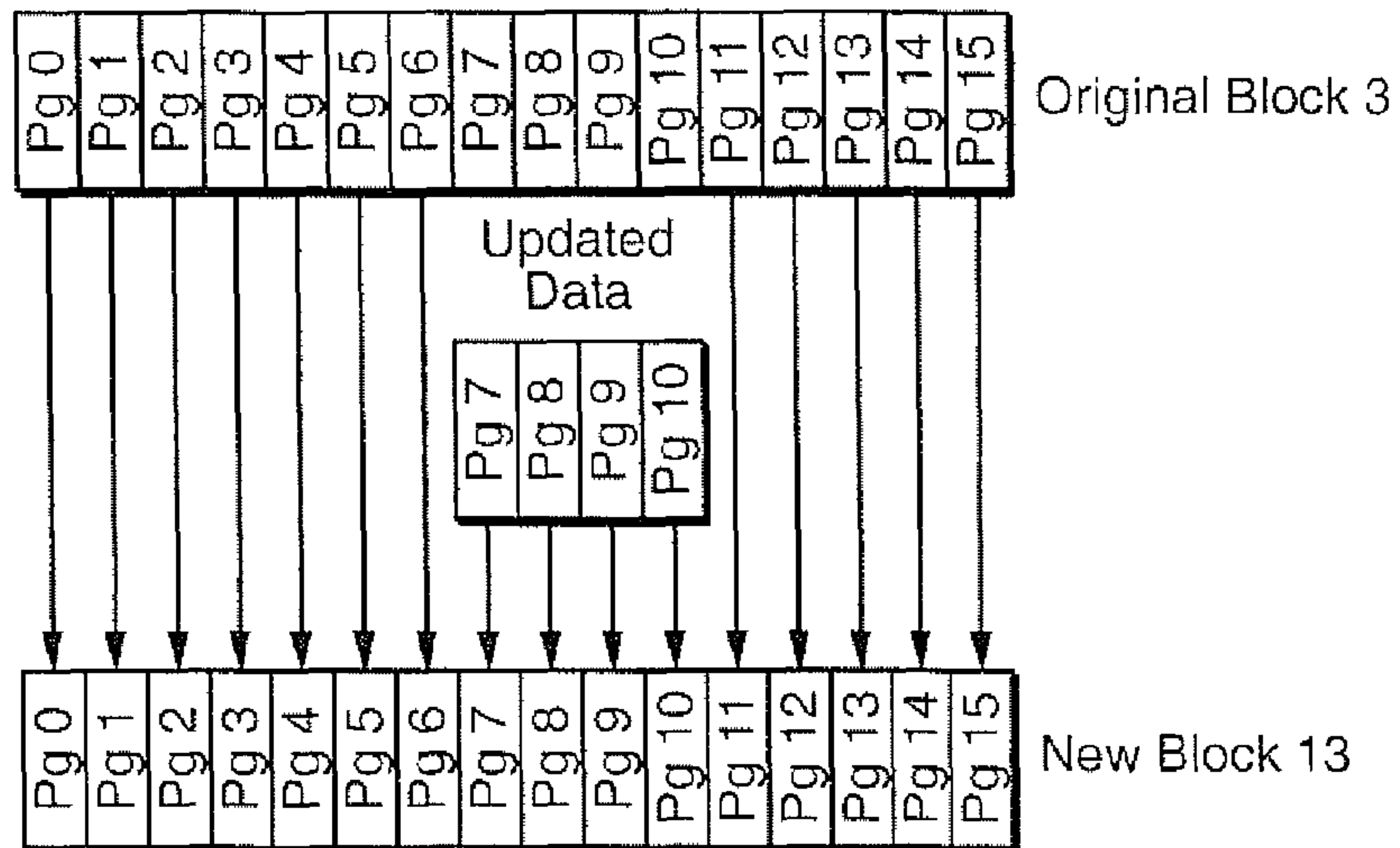
FIG. 6 (PRIOR ART)
