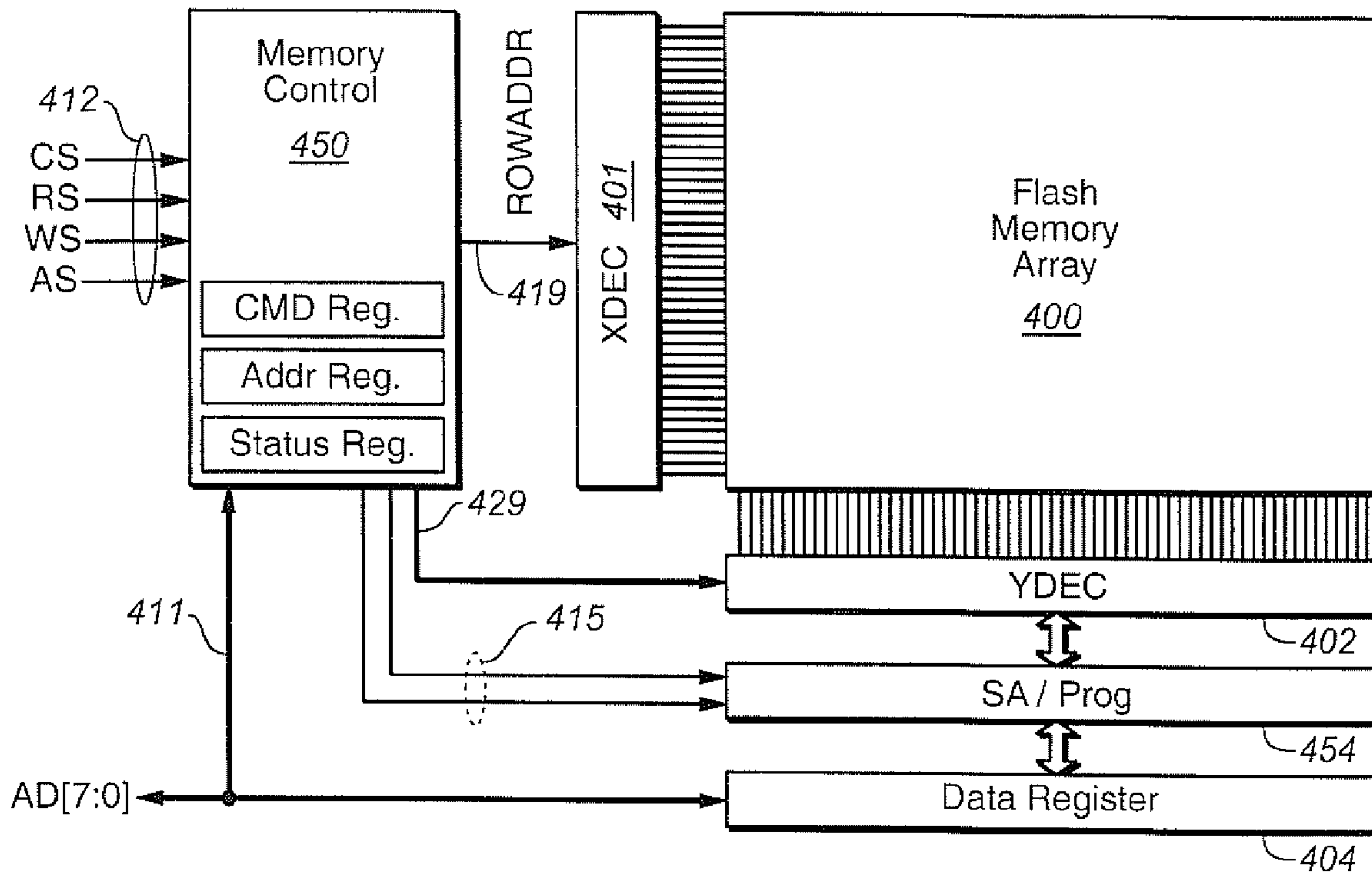
FIG. 1 (PRIOR ART)
