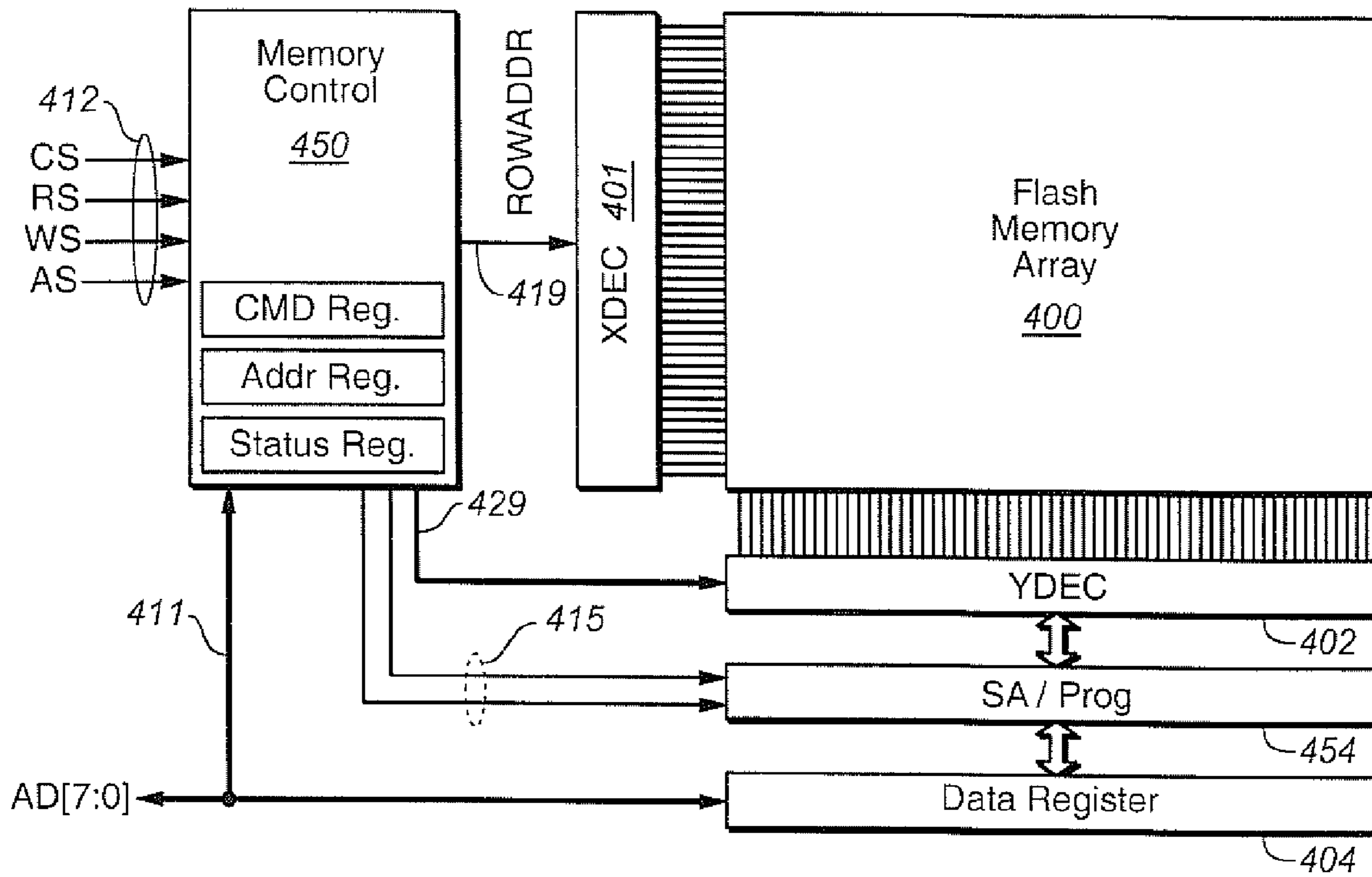
FIG. 1 (PRIOR ART)
