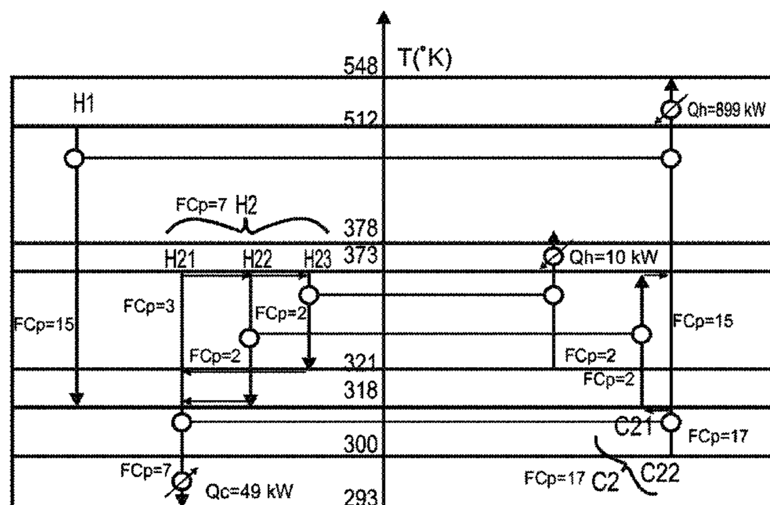
NUMBER OF HEAT EXCHANGERS USED IS 7.
